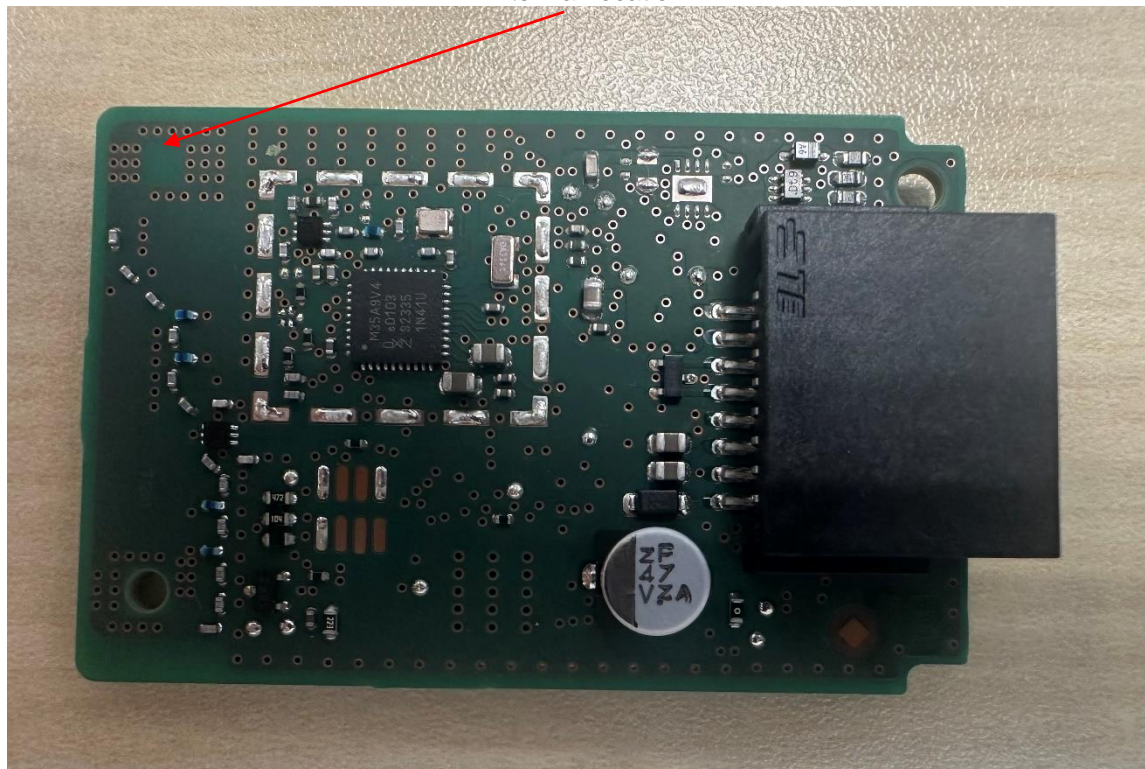
Antenna Location
