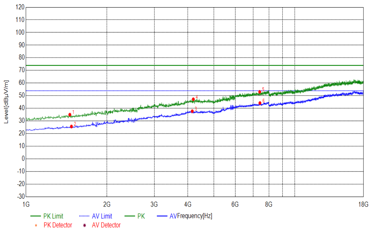
(Plot N: Test Antenna Vertical 1G – 18G)
