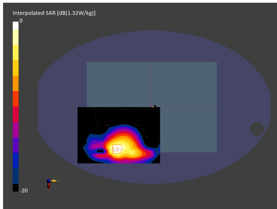
Figure C.22: SAR Testing Results for the A3112 at 2457 MHz Core 1
