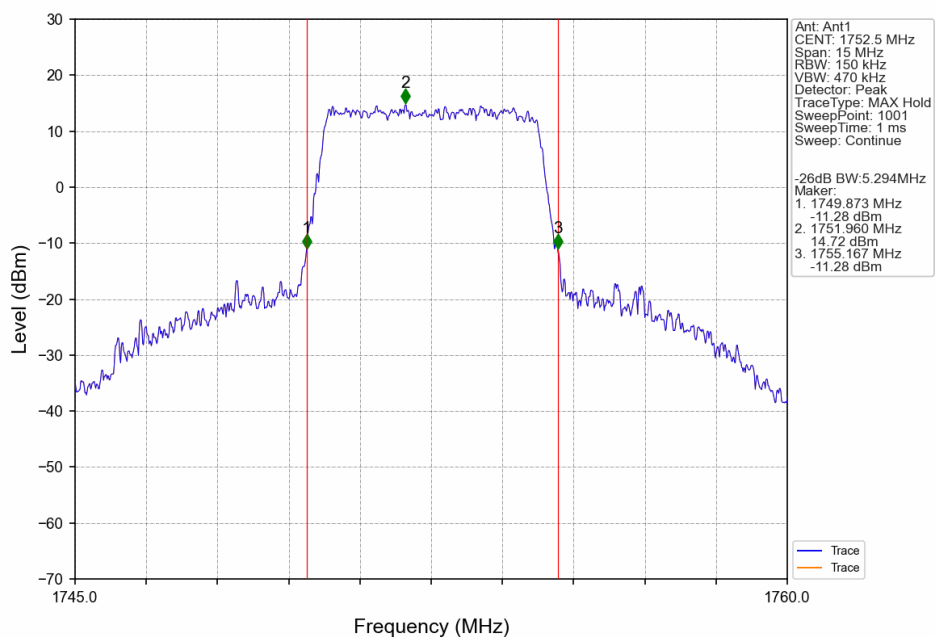
Band4_5MHz_16QAM_HCH_1752.5MHz_RB_25_0 NTN
