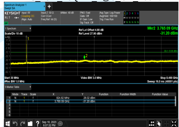
B26 10M 16QAM 1@0 CH 26915
