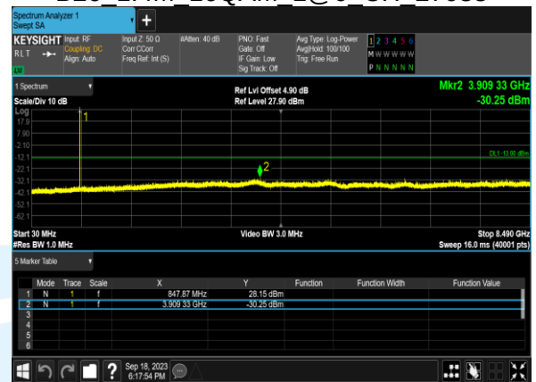
B26 1.4M 16QAM 1@0 CH 27033
