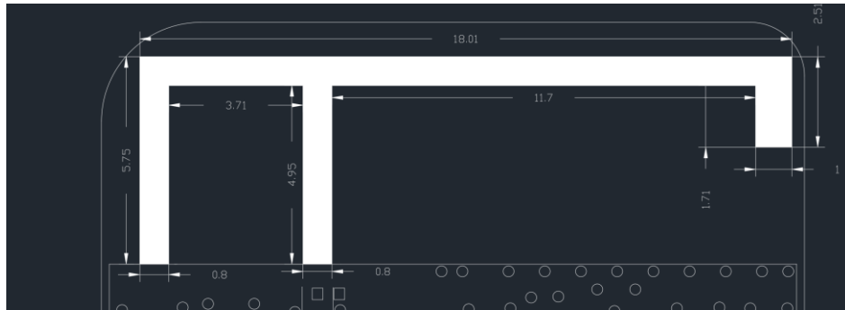
Figure 1 Antenna, Unit: mm
