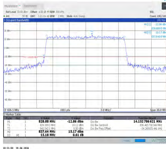
1-N5-15-15-M-8-CP-64QAM-Outer_Full-79@0-Ant0-14.153-15.180-≤15-PASS
