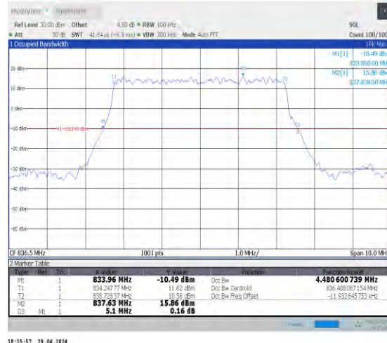
1-N5-15-5-M-2-DFT-PI2BPSK-Outet_Full-25@0-Ant 0-4.481-5.100-≤5-PASS
