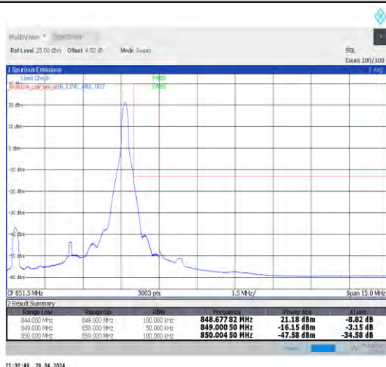
1-N5-15-5-H-5-CP-QPSK-Edge_1RB_Right-1@24-Ant0-1--PASS-see graph
