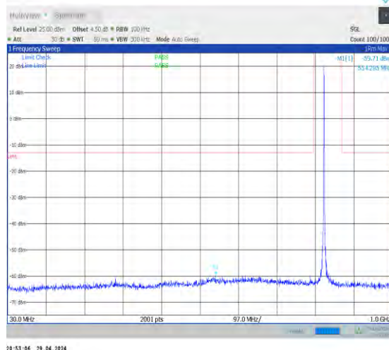
1-N5-15-20-M-1-DFT-PI2BPSK-Inner_1RB_Left-1@ 1-30-1000-Ant0-554.29--59.71--13-PASS
