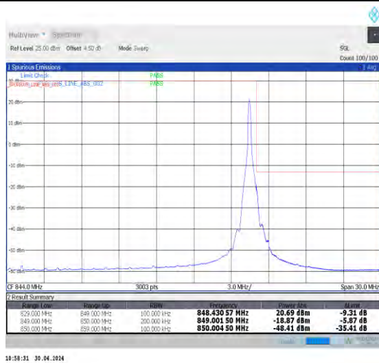
1-N5-15-20-H-2-DFT-PI2BPSK-Edge_1RB_Right-1@105-Ant0-1--PASS-see graph
