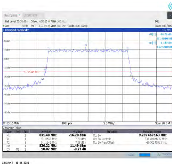
1-N5-15-10-M-6-CP-QPSK-Outer_Full-52@0-Ant0-9. 269-10.020≤10-PASS
