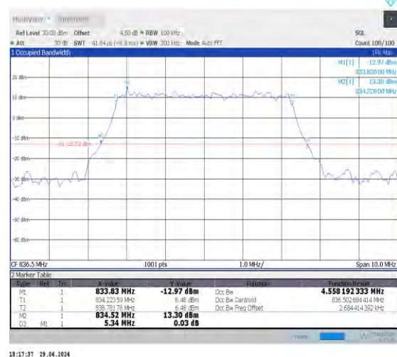
1-N5-15-5-M-8-CP-64QAM-Outer_Full-25@0-Ant0-4 .558-5.340-≤5-PASS
