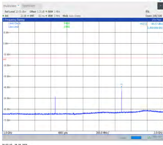
1-N5-15-20-M-1-DFT-PI2BPSK-Inner_1RB_Left-1@ 1-1000-3000-Ant0-2482.00--40.57--13-PASS
