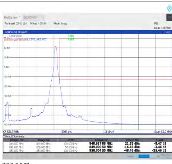
1-N5-15-5-H-2-DFT-PI2BPSK-Edge_1RB_Right-1@24-Ant0-1--PASS-see graph
