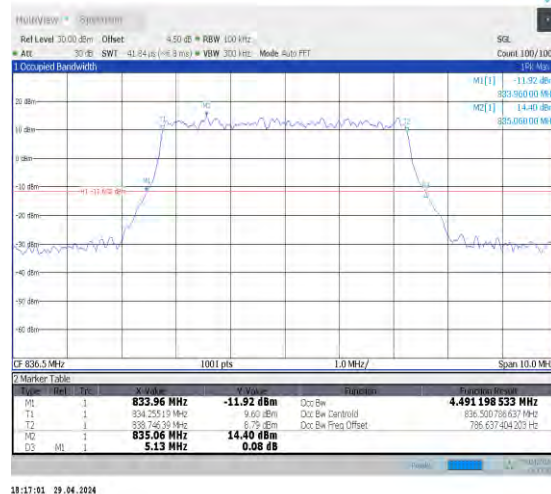
1-N5-15-5-M-4-DFT-64QAM-Outet_Full-25@0-Ant0- 4.491-5.130-≤5-PASS
