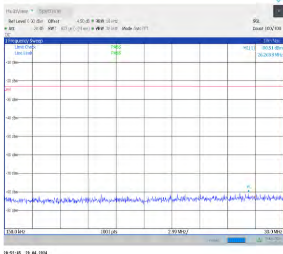
1-N5-15-20-M-1-DFT-PI2BPSK-Inner_1RB_Left-1@ 1-0.15-30-Ant0-26.27--80.51--23-PASS
