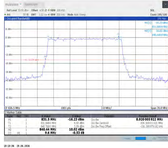
1-N5-15-10-M-5-DFT-256QAM-Outer_Full-50@0-Ant 0-8.92-9.600≤10-PASS
