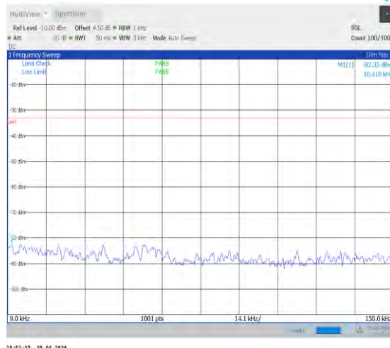
1-N5-15-20-M-1-DFT-PI2BPSK-Inner_1RB_Left-1@ 1-0.009-0.15-Ant0-0.01--82.35--33-PASS
