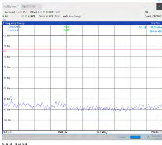
1-N5-15-20-H-1-DFT-PI2BPSK-Inner_1RB_Left-1@1 -0.009-0.15-Ant0-0.02--81.59--33-PASS
