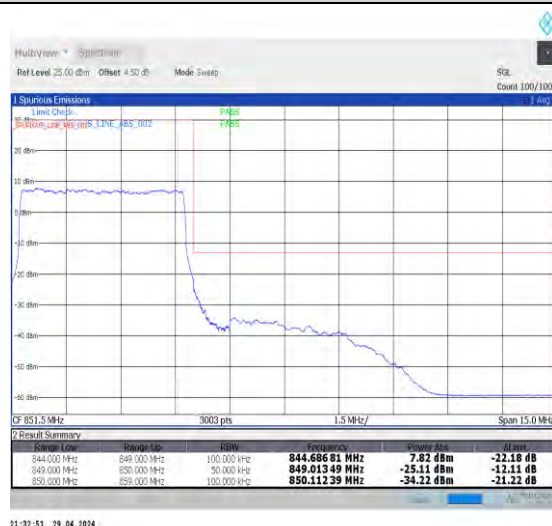
1-N5-15-5-H-6-CP-QPSK-Outer_Full-25@0-Ant0-1--PASS-see graph
