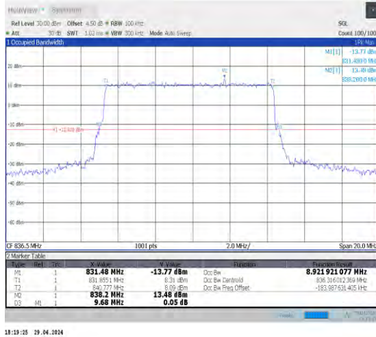
1-N5-15-10-M-4-DFT-64QAM-Outer_Full-50@0-Ant0 -8.922-9.680≤10-PASS
