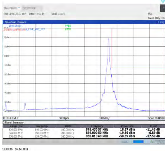
1-N5-15-20-H-5-CP-QPSK-Edge_1RB_Right-1@105-Ant0-1--PASS-see graph
