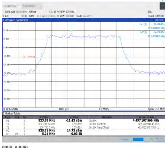
1-N5-15-5-M-3-DFT-16QAM-Outet_Full-25@0-Ant0- 4.497-5.210-≤5-PASS
