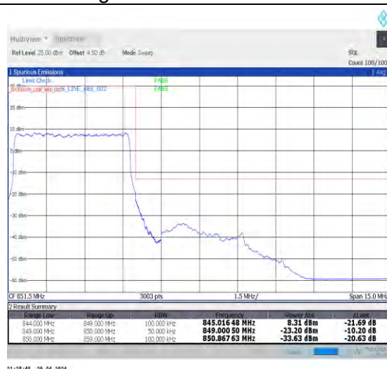
1-N5-15-5-H-3-DFT-PI2BPSK-Outer_Full-25@0-Ant0-1--PASS-see graph
