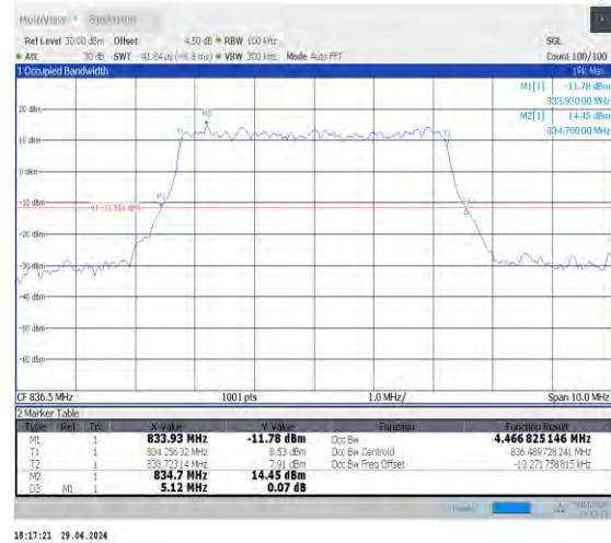
1-N5-15-5-M-6-CP-QPSK-Outer_Full-25@0-Ant0-4. 467-5.120-≤5-PASS
