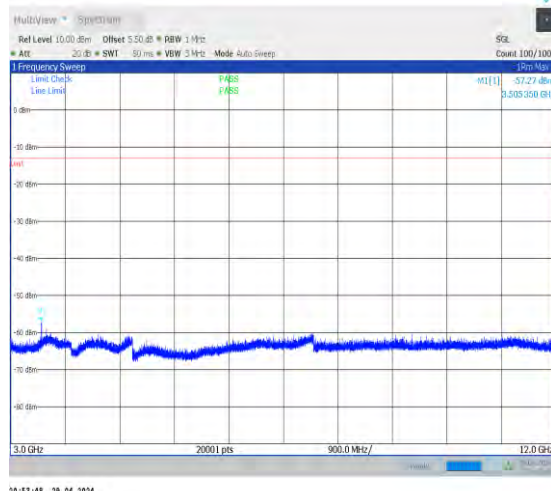
1-N5-15-20-M-1-DFT-PI2BPSK-Inner_1RB_Left-1@ 1-3000-12000-Ant0-3505.35--57.27--13-PASS
