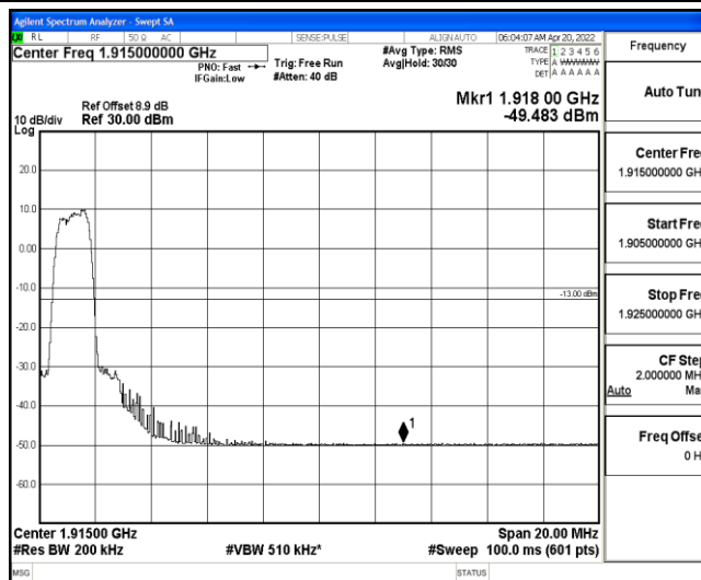
Band25-10MHz-QPSK-26640-6-0-Low--49.48-PASS
