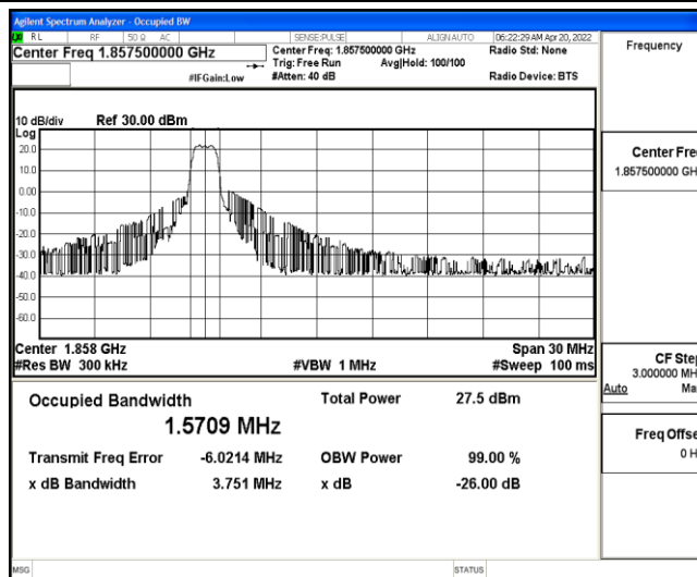
Band25-15MHz-QPSK-26115-6-0-Low-1.5709-3.751-PASS
