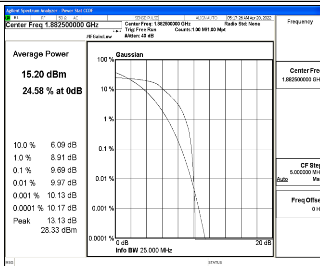
Band25-5MHz-16QAM-26365-6-0-Low-9.69-&lt;=13-PASS
