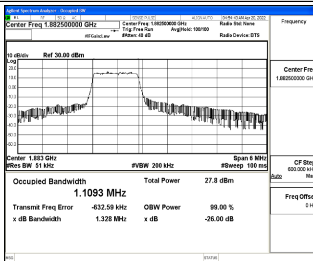
Band25-3MHz-QPSK-26365-6-0-Low-1.1093-1.328-PASS
