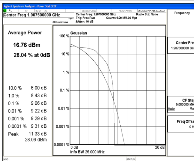
Band25-15MHz-QPSK-26615-6-0-Low-9.06-&lt;=13-PASS
