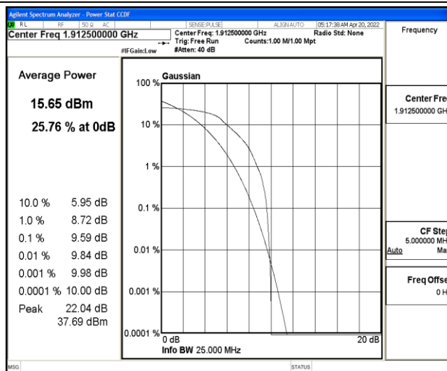
Band25-5MHz-QPSK-26665-6-0-Low-9.59-&lt;=13-PASS
