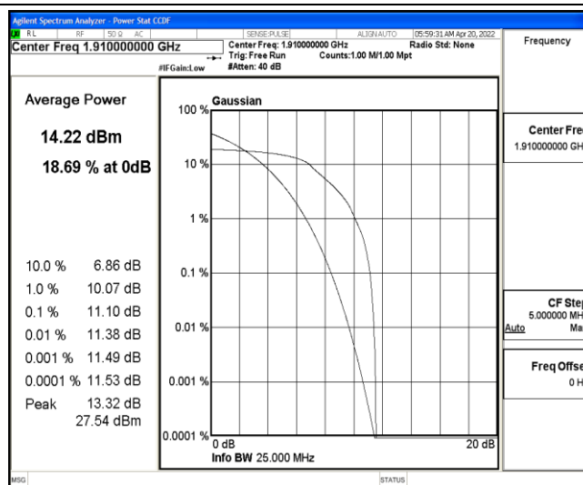
Band25-10MHz-QPSK-26640-6-0-Low-11.10-&lt;=13-PASS
