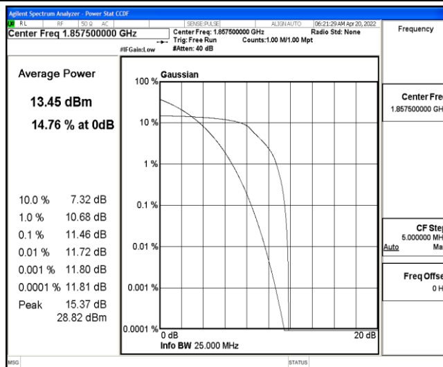
Band25-15MHz-16QAM-26115-6-0-Low-11.46-&lt;=13-PASS
