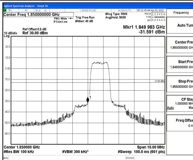
Band25-5MHz-16QAM-26065-6-0-Low--31.59-PASS
