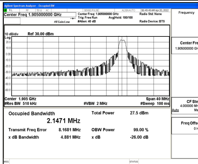
Band25-20MHz-QPSK-26590-6-0-High-2.1471-4.881-PASS
