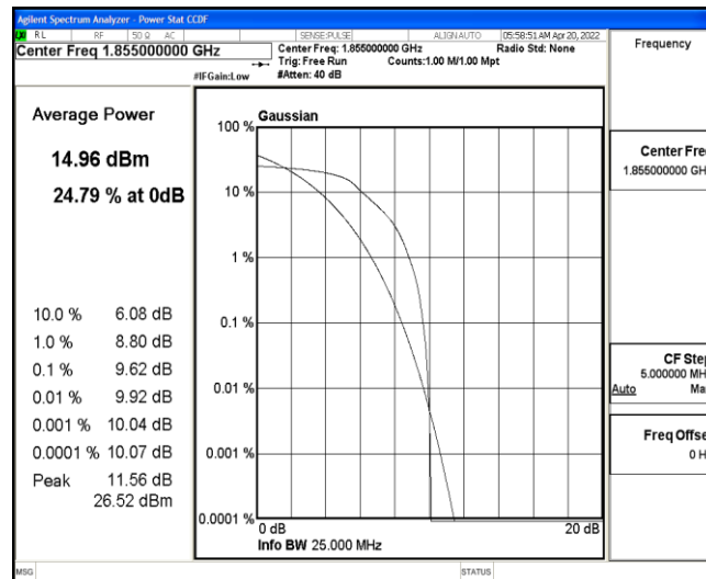
Band25-10MHz-QPSK-26090-6-0-Low-9.62-&lt;=13-PASS
