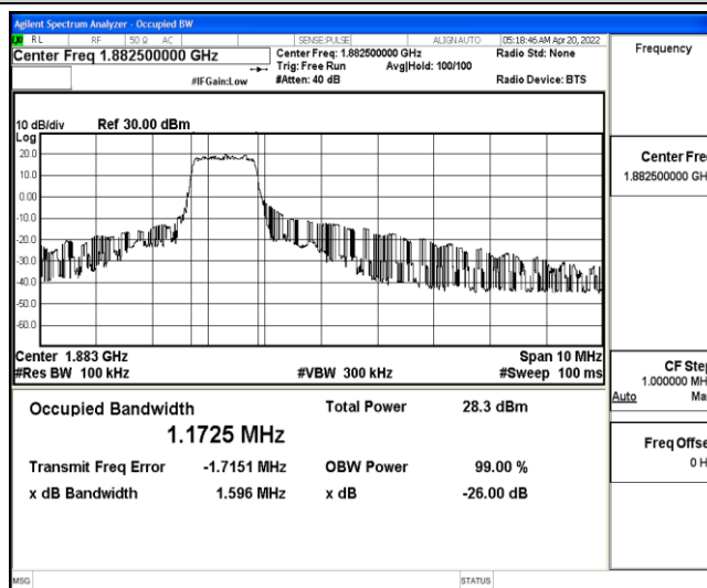
Band25-5MHz-QPSK-26365-6-0-Low-1.1725-1.596-PASS
