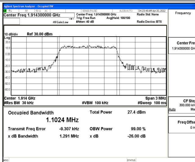
Band25-1.4MHz-QPSK-26683-6-0-High-1.1024-1.291-PASS
