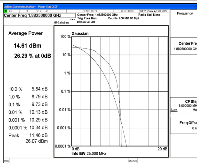
Band25-1.4MHz-16QAM-26365-6-0-Low-9.73-&lt;=13-PASS
