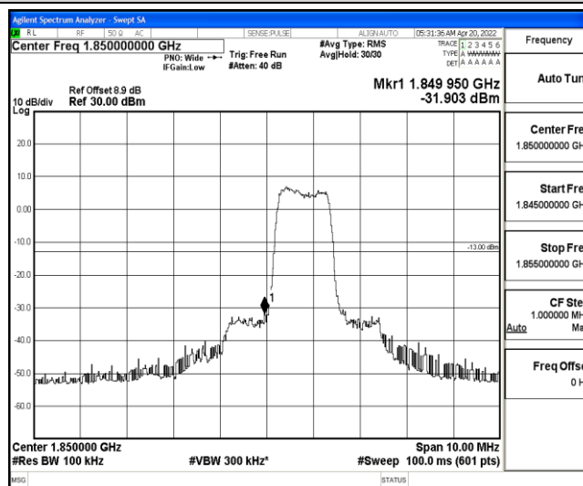
Band25-5MHz-QPSK-26065-6-0-Low--31.90-PASS
