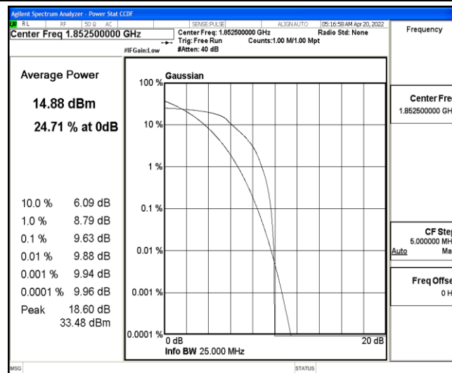
Band25-5MHz-QPSK-26065-6-0-Low-9.63-&lt;=13-PASS
