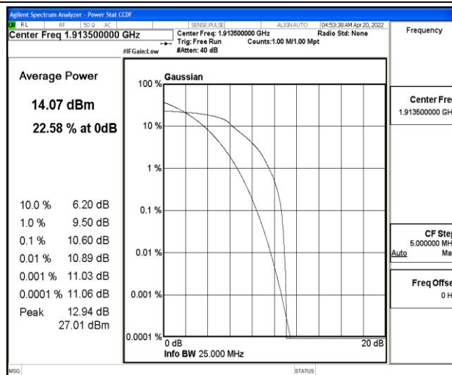
Band25-3MHz-QPSK-26675-6-0-Low-10.60-&lt;=13-PASS
