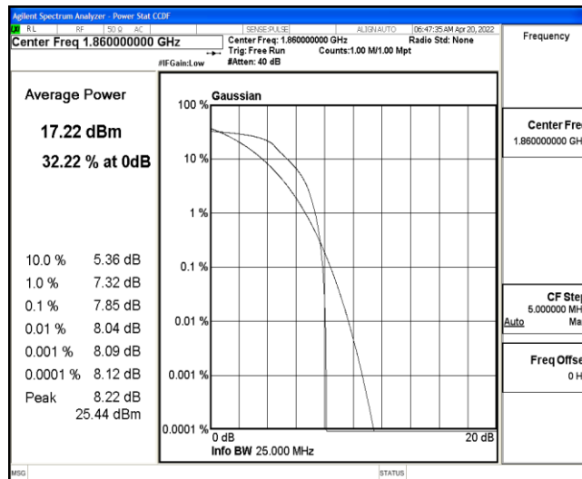
Band25-20MHz-16QAM-26140-6-0-Low-7.85-&lt;=13-PASS
