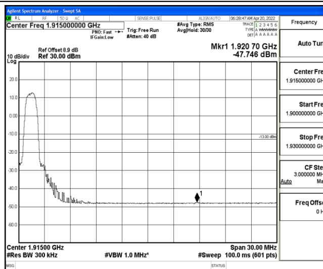
Band25-15MHz-QPSK-26615-6-0-Low--47.75-PASS
