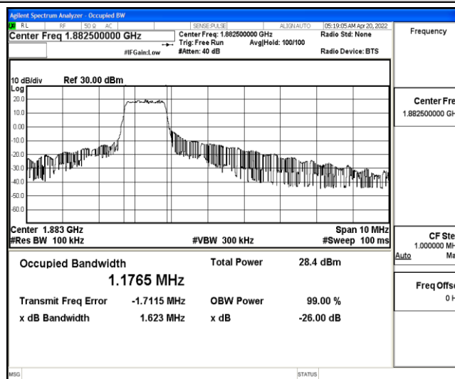
Band25-5MHz-16QAM-26365-6-0-Low-1.1765-1.623-PASS
