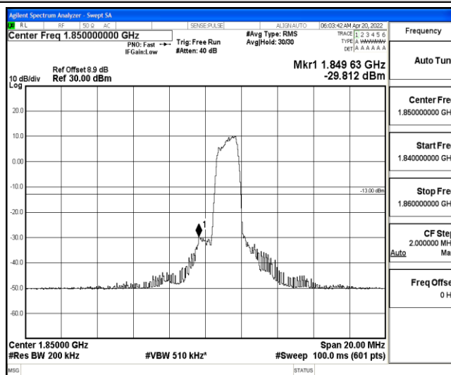
Band25-10MHz-16QAM-26090-6-0-Low--29.81-PASS
