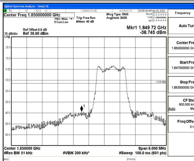
Band25-3MHz-16QAM-26055-6-0-Low--38.74-PASS
