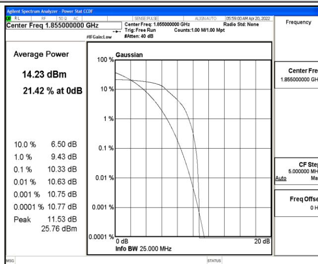
Band25-10MHz-16QAM-26090-6-0-Low-10.33-&lt;=13-PASS
