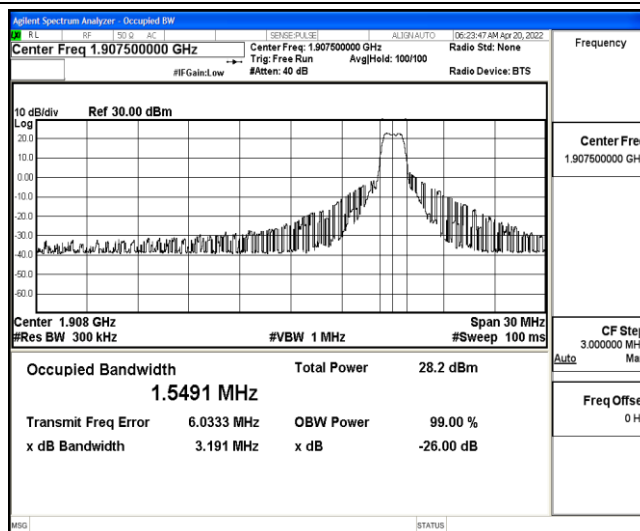
Band25-15MHz-QPSK-26615-6-0-High-1.5491-3.191-PASS
