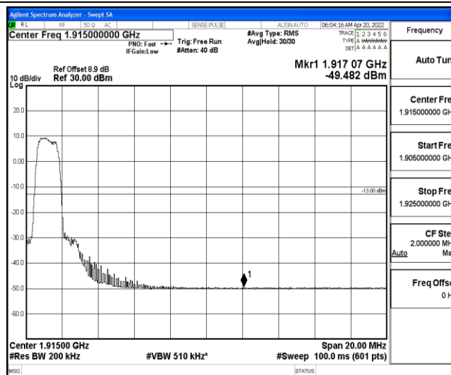
Band25-10MHz-16QAM-26640-6-0-Low--49.48-PASS
