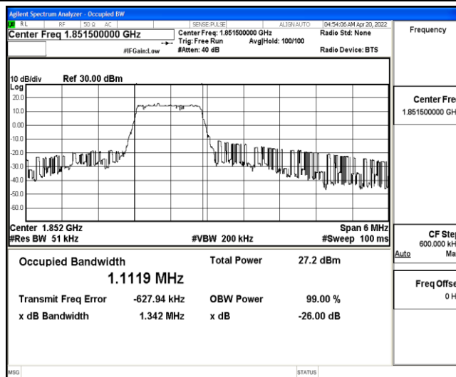
Band25-3MHz-QPSK-26055-6-0-Low-1.1119-1.342-PASS
