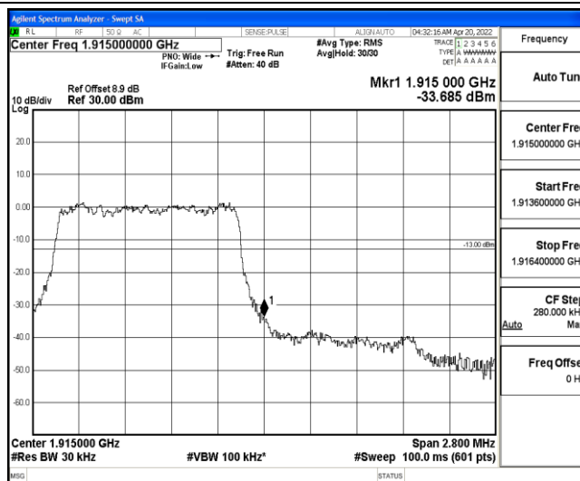
Band25-1.4MHz-16QAM-26683-6-0-Low--33.68-PASS
