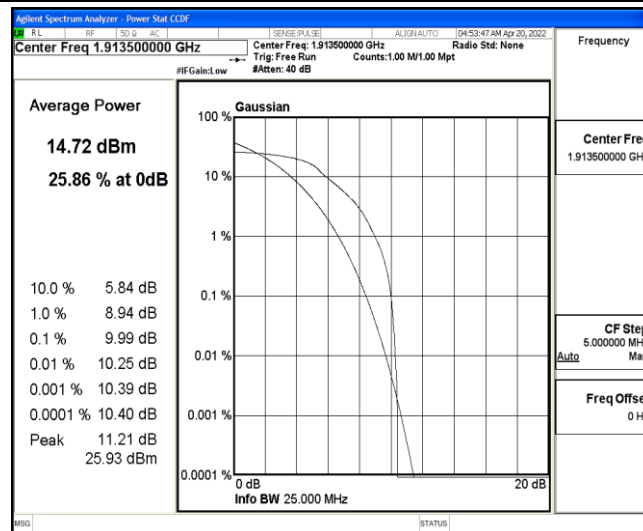
Band25-3MHz-16QAM-26675-6-0-Low-9.99-&lt;=13-PASS
