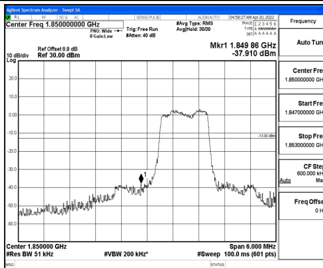
Band25-3MHz-QPSK-26055-6-0-Low--37.91-PASS
