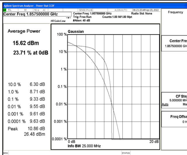
Band25-15MHz-QPSK-26115-6-0-Low-9.33-&lt;=13-PASS
