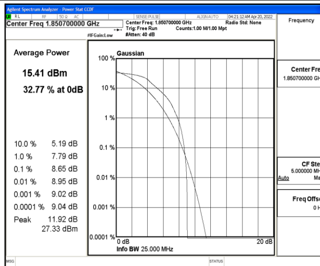
Band25-1.4MHz-QPSK-26047-6-0-Low-8.65-<=13-PASS
