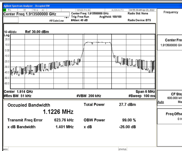
Band25-3MHz-16QAM-26675-6-0-High-1.1226-1.401-PASS
