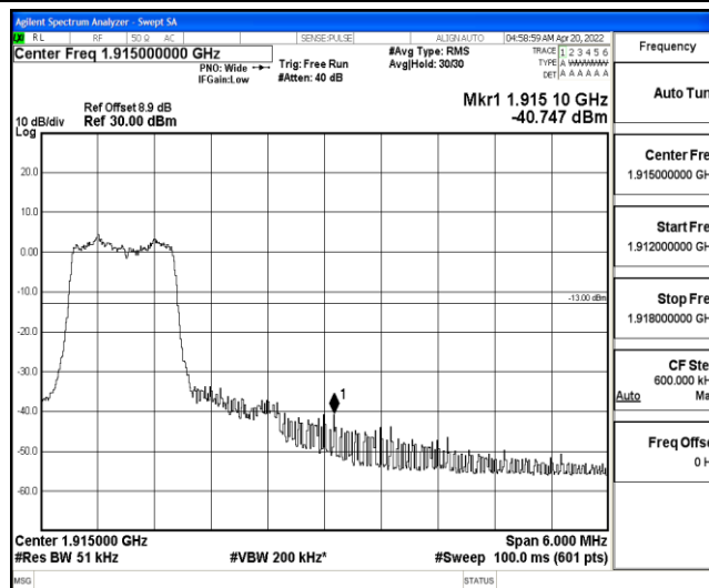
Band25-3MHz-16QAM-26675-6-0-Low--40.75-PASS
