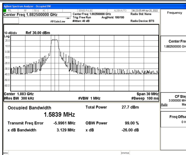
Band25-15MHz-QPSK-26365-6-0-Low-1.5839-3.129-PASS
