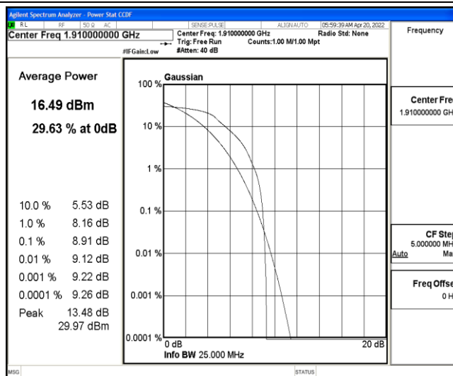
Band25-10MHz-16QAM-26640-6-0-Low-8.91-&lt;=13-PASS
