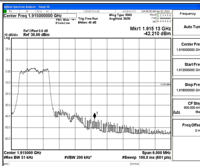
Band25-3MHz-QPSK-26675-6-0-Low--42.21-PASS
