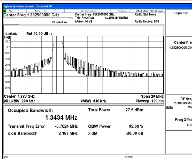
Band25-10MHz-QPSK-26365-6-0-Low-1.3434-2.193-PASS
