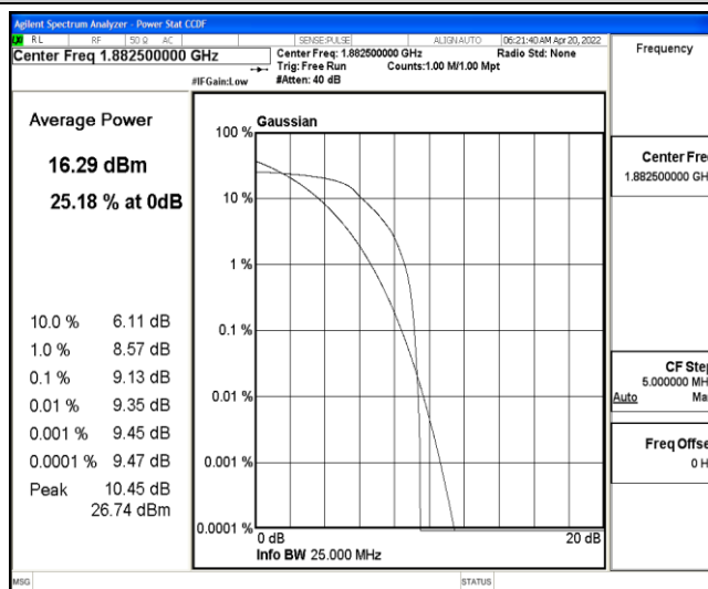
Band25-15MHz-QPSK-26365-6-0-Low-9.13-&lt;=13-PASS
