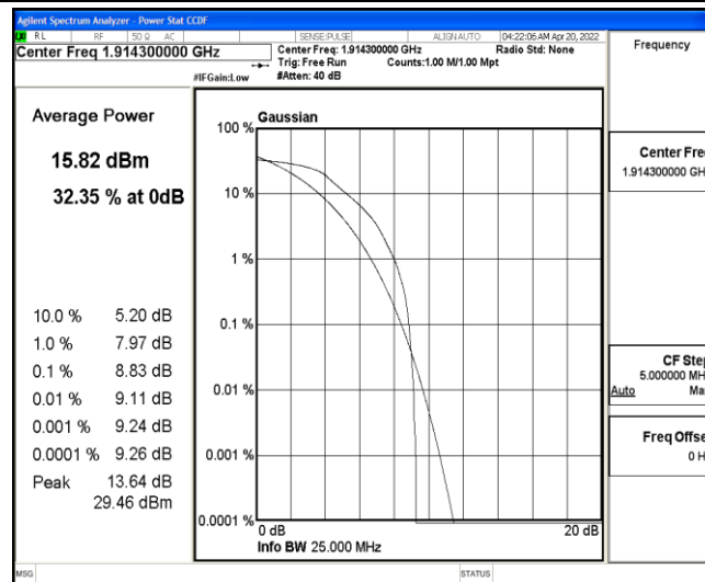
Band25-1.4MHz-16QAM-26683-6-0-Low-8.83-&lt;=13-PASS
