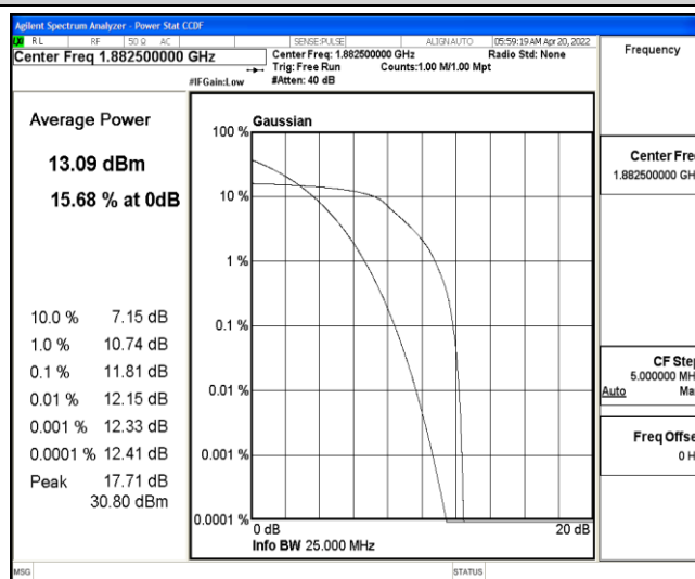
Band25-10MHz-16QAM-26365-6-0-Low-11.81-&lt;=13-PASS
