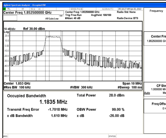
Band25-5MHz-16QAM-26065-6-0-Low-1.1835-1.610-PASS
