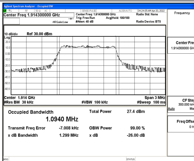
Band25-1.4MHz-16QAM-26683-6-0-High-1.0940-1.299-PASS
