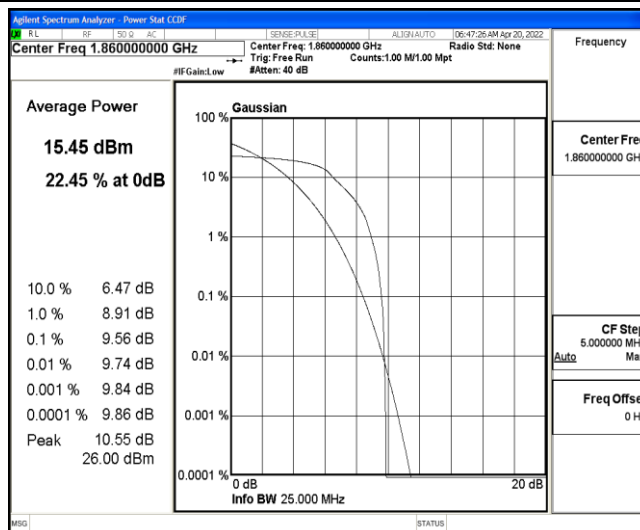
Band25-20MHz-QPSK-26140-6-0-Low-9.56-&lt;=13-PASS
