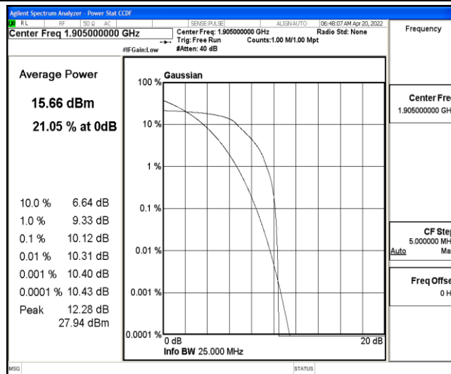
Band25-20MHz-QPSK-26590-6-0-Low-10.12-&lt;=13-PASS
