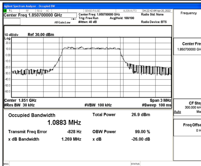
Band25-1.4MHz-16QAM-26047-6-0-Low-1.0883-1.269-PASS
