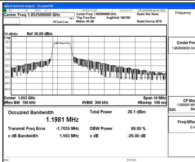
Band25-5MHz-QPSK-26065-6-0-Low-1.1981-1.593-PASS
