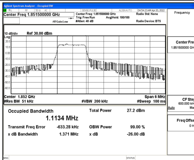
Band25-3MHz-16QAM-26055-6-0-Low-1.1134-1.371-PASS
