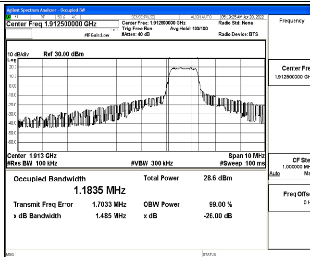
Band25-5MHz-QPSK-26665-6-0-High-1.1835-1.485-PASS
