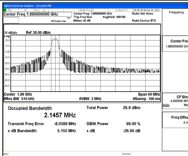
Band25-20MHz-QPSK-26140-6-0-Low-2.1457-5.155-PASS
