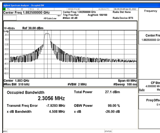
Band25-20MHz-16QAM-26365-6-0-Low-2.3056-4.508-PASS
