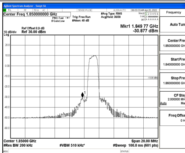
Band25-10MHz-QPSK-26090-6-0-Low--30.88-PASS
