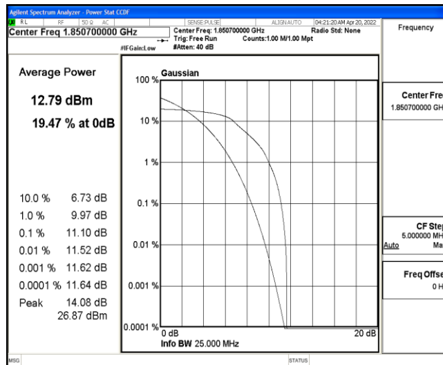
Band25-1.4MHz-16QAM-26047-6-0-Low-11.10-&lt;=13-PASS
