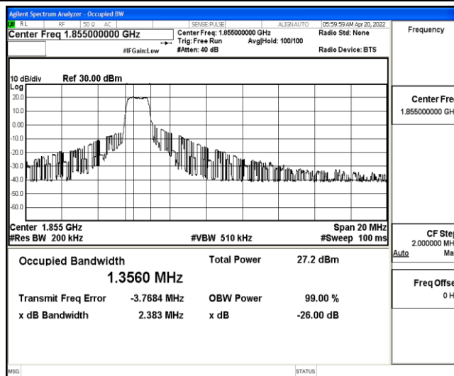
Band25-10MHz-QPSK-26090-6-0-Low-1.3560-2.383-PASS
