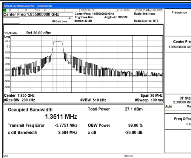
Band25-10MHz-16QAM-26090-6-0-Low-1.3511-2.684-PASS
