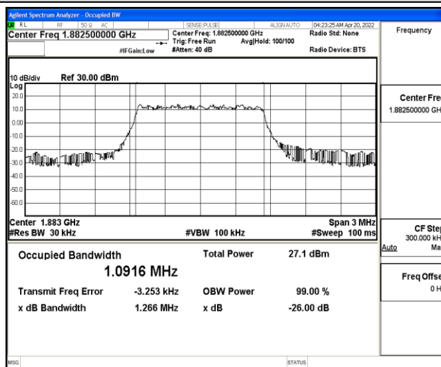
Band25-1.4MHz-16QAM-26365-6-0-Low-1.0916-1.266-PASS
