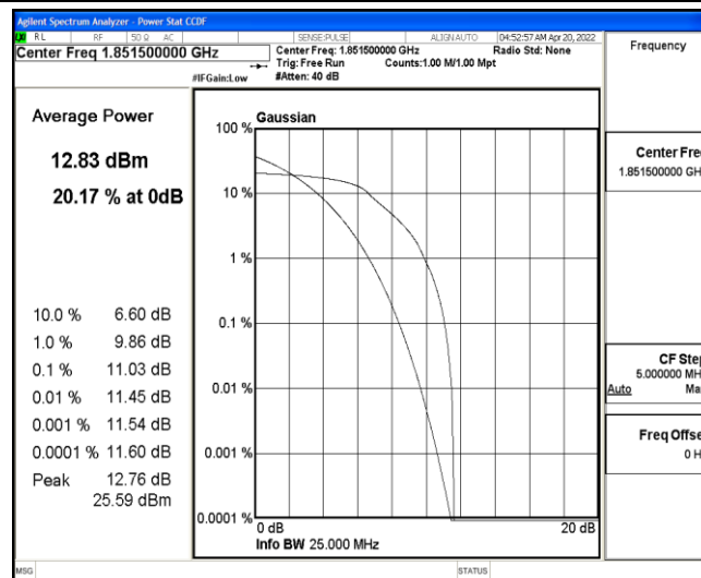
Band25-3MHz-QPSK-26055-6-0-Low-11.03-&lt;=13-PASS
