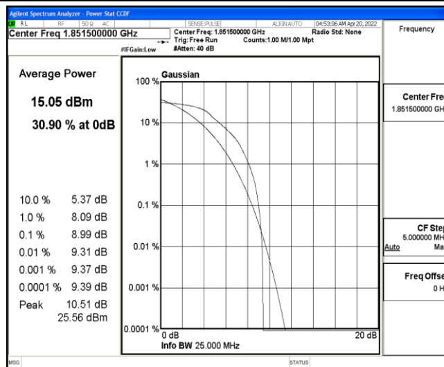
Band25-3MHz-16QAM-26055-6-0-Low-8.99-&lt;=13-PASS
