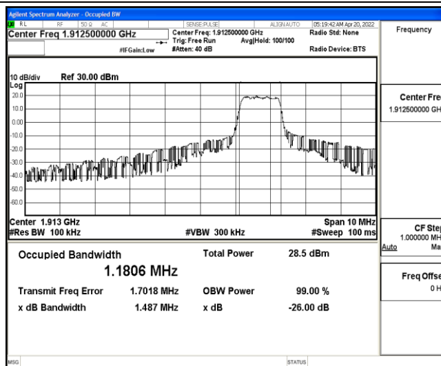
Band25-5MHz-16QAM-26665-6-0-High-1.1806-1.487-PASS
