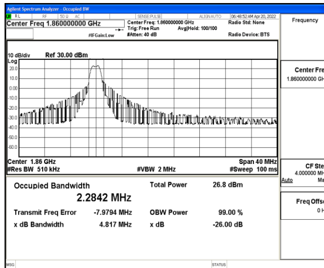
Band25-20MHz-16QAM-26140-6-0-Low-2.2842-4.817-PASS
