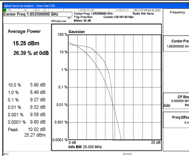
Band25-5MHz-16QAM-26065-6-0-Low-9.27-&lt;=13-PASS
