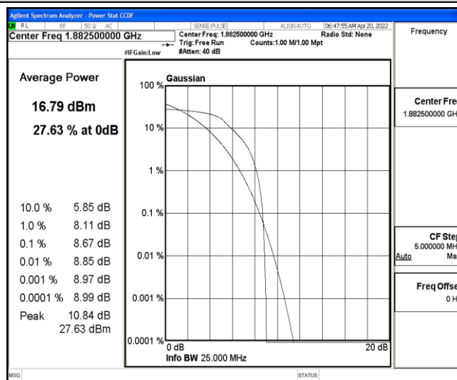
Band25-20MHz-16QAM-26365-6-0-Low-8.67-&lt;=13-PASS
