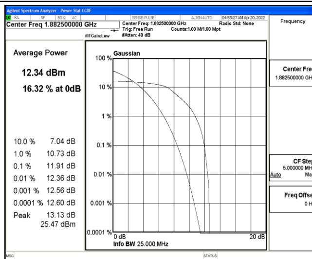
Band25-3MHz-16QAM-26365-6-0-Low-11.91-&lt;=13-PASS
