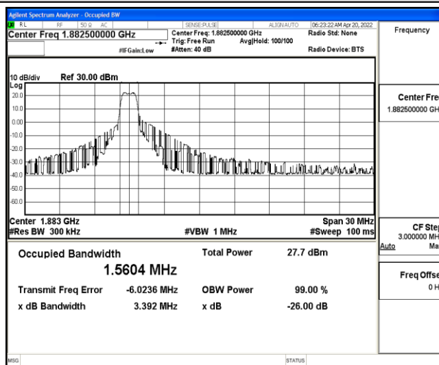
Band25-15MHz-16QAM-26365-6-0-Low-1.5604-3.392-PASS
