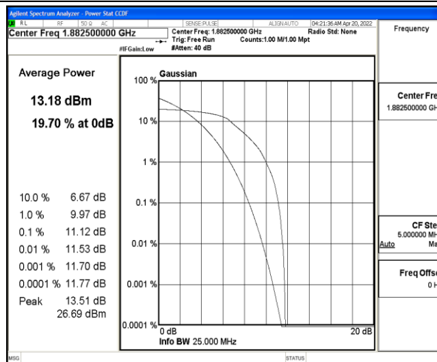
Band25-1.4MHz-QPSK-26365-6-0-Low-11.12-<=13-PASS
