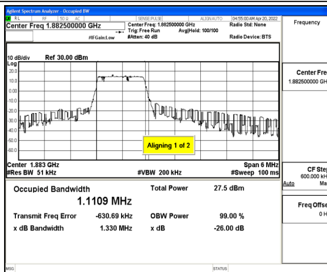
Band25-3MHz-16QAM-26365-6-0-Low-1.1109-1.330-PASS
