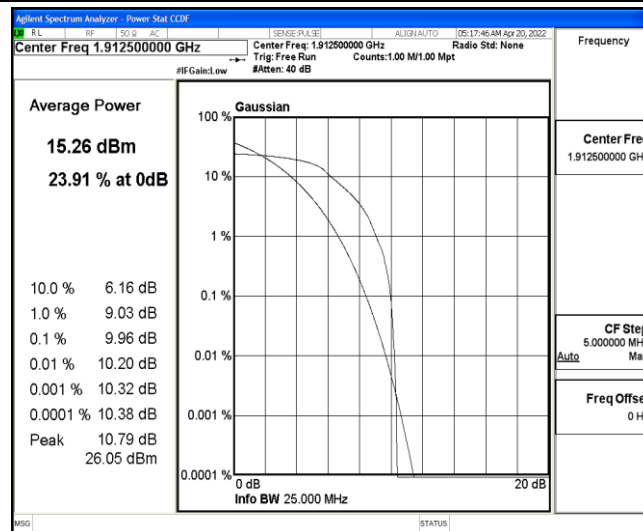
Band25-5MHz-16QAM-26665-6-0-Low-9.96-&lt;=13-PASS
