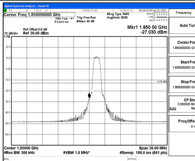
Band25-15MHz-QPSK-26115-6-0-Low--27.03-PASS
