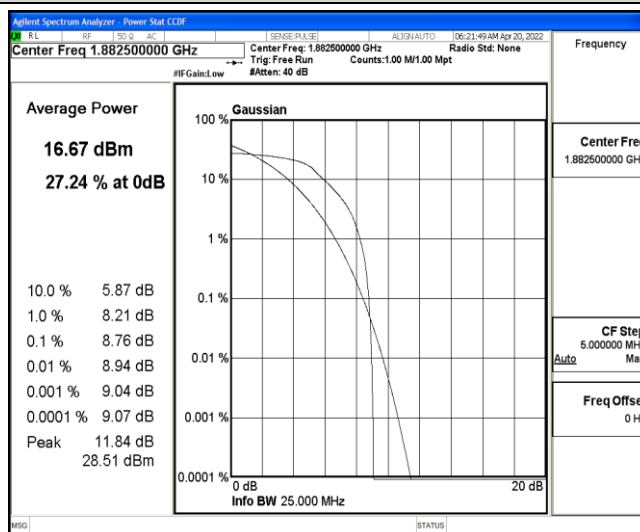
Band25-15MHz-16QAM-26365-6-0-Low-8.76-&lt;=13-PASS
