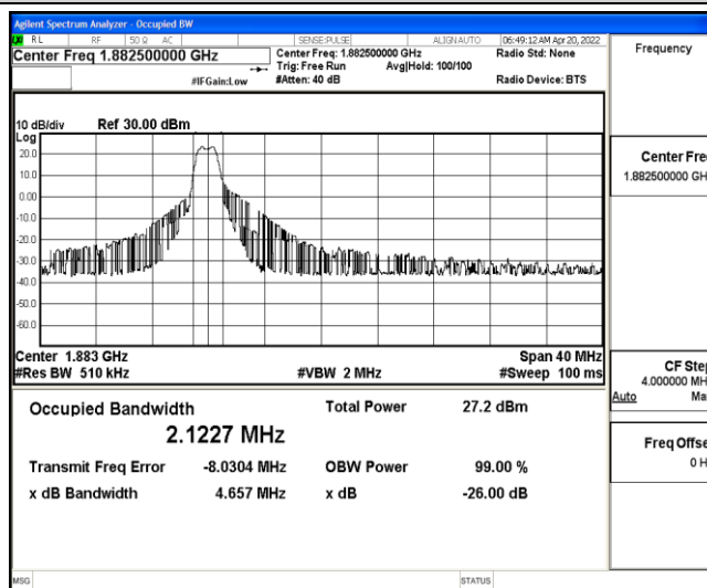
Band25-20MHz-QPSK-26365-6-0-Low-2.1227-4.657-PASS
