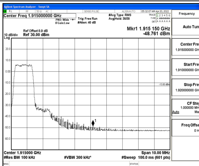
Band25-5MHz-16QAM-26665-6-0-Low--48.76-PASS
