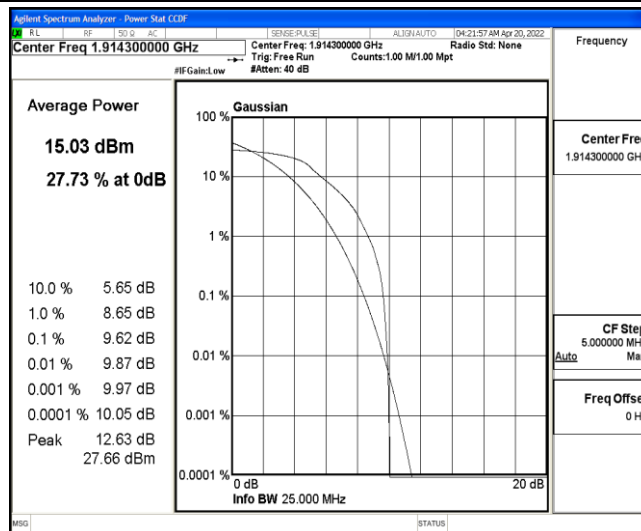
Band25-1.4MHz-QPSK-26683-6-0-Low-9.62-&lt;=13-PASS
