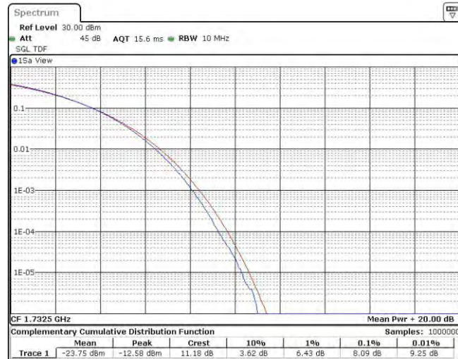
Band4-10MHz-QPSK-20175-50RB#0
