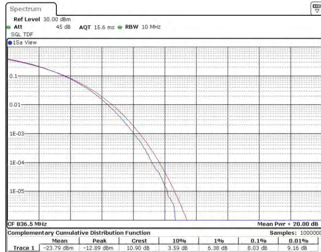
Band5-10MHz-QPSK-20525-50RB#0
