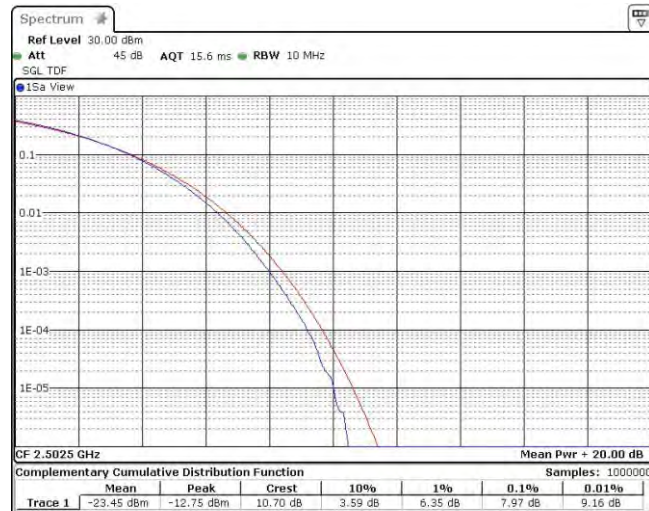
Band7-5MHz-QPSK-20775-25RB#0
