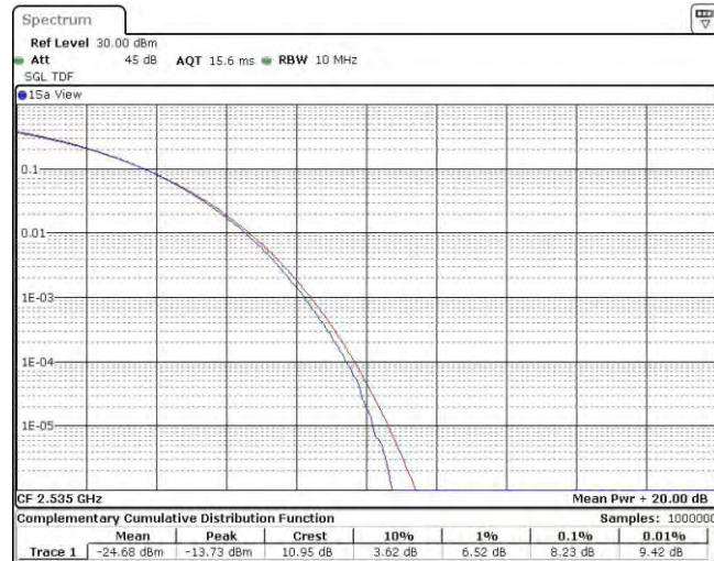
Band7-10MHz-QPSK-21100-50RB#0
