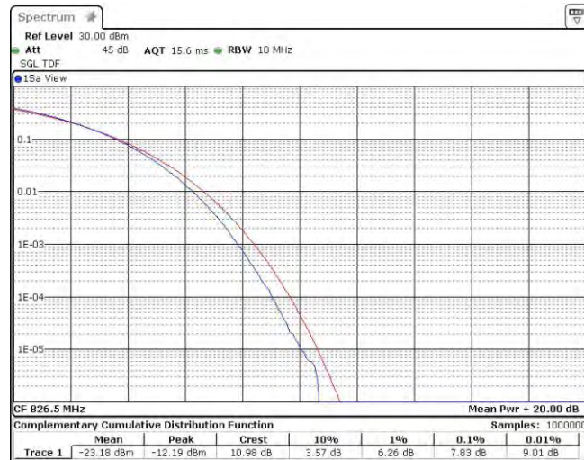
Band5-5MHz-QPSK-20425-25RB#0
