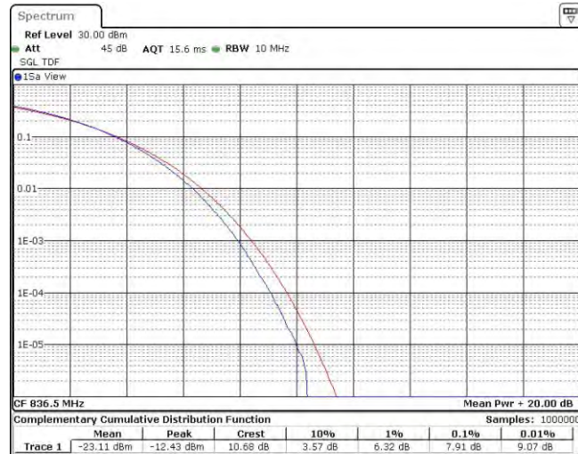
Band5-5MHz-16QAM-20525-25RB#0
