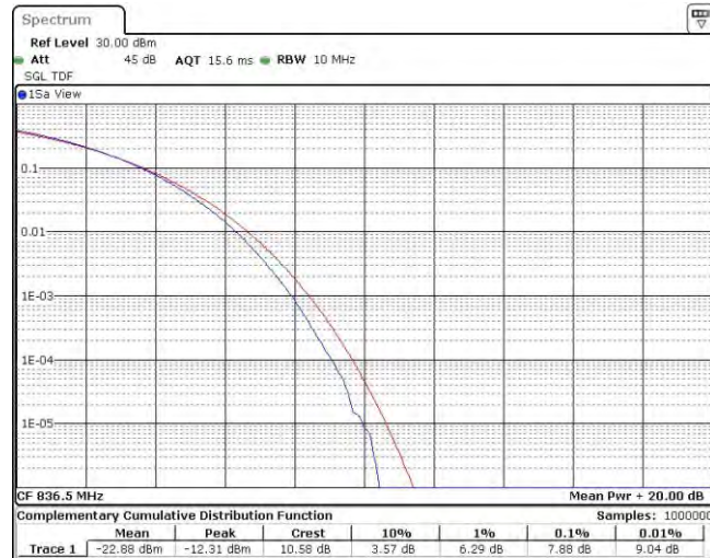
Band5-3MHz-16QAM-20525-15RB#0
