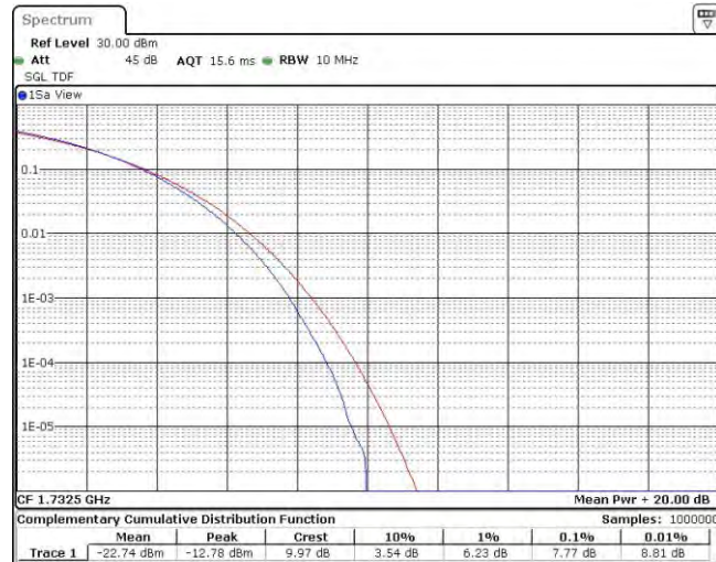
Band4-3MHz-QPSK-20175-15RB#0
