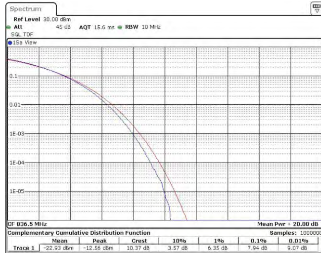
Band5-1.4MHz-16QAM-20525-6RB#0
