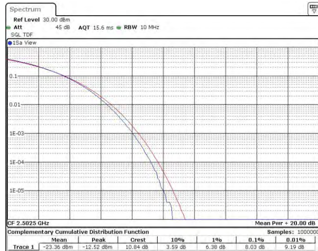
Band7-5MHz-16QAM-20775-25RB#0
