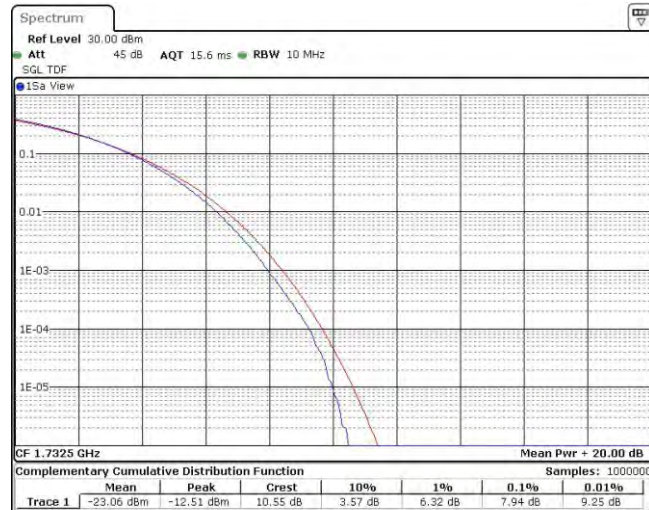
Band4-5MHz-QPSK-20175-25RB#0
