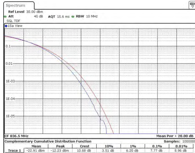
Band5-3MHz-QPSK-20525-15RB#0
