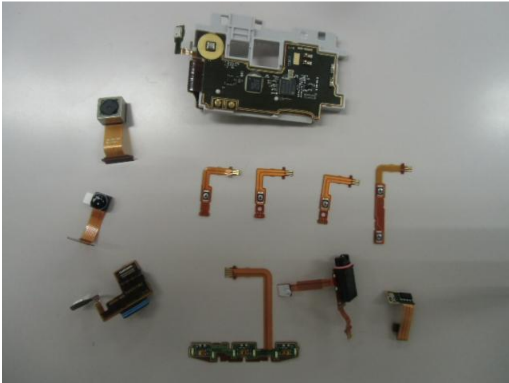
Side Key & Sub FPC
