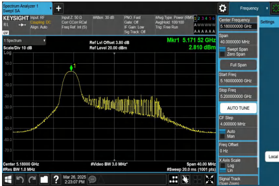
11AX20MIMO-Ant1-5180-52Tone-RU37-PASS
