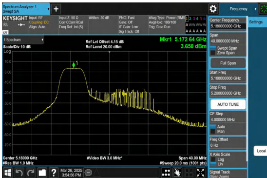
11AX20MIMO-Ant1-5180-106Tone-RU53-PASS
