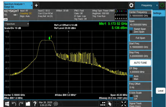
11AX20MIMO-Ant2-5180-106Tone-RU53-PASS
