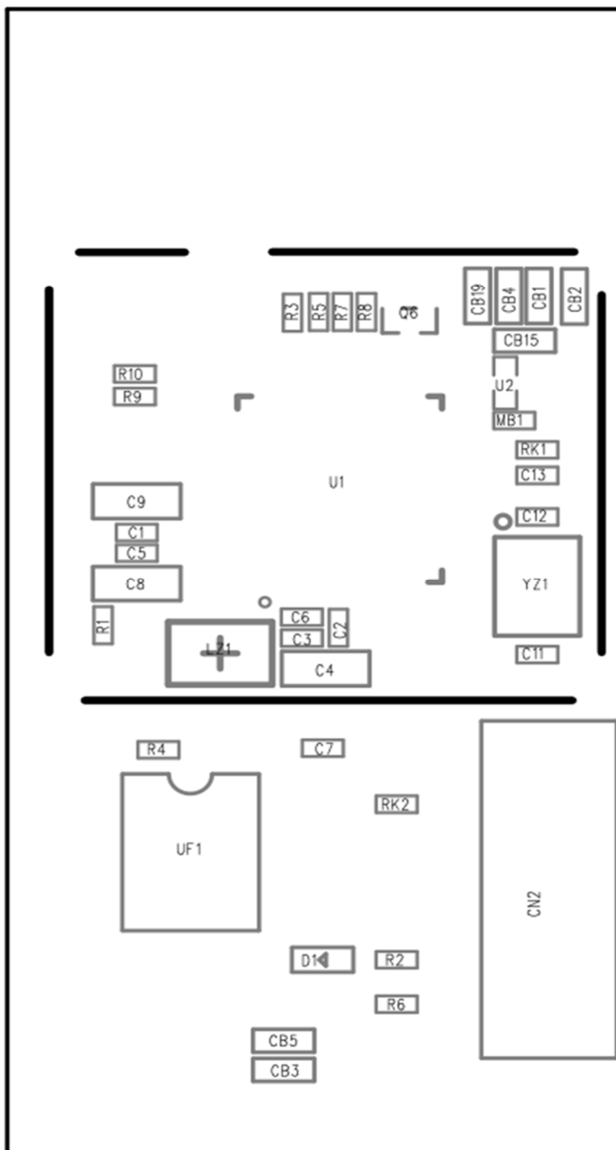
Top Silkscreen
