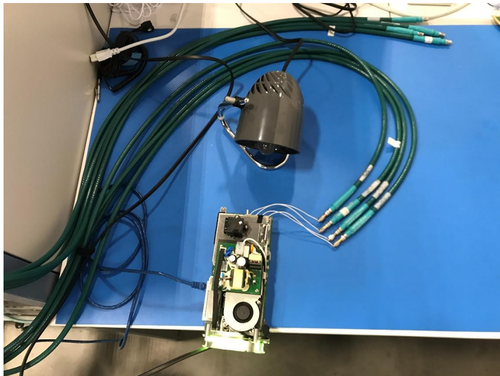
Photograph 3: RF Conducted Test Set Up
