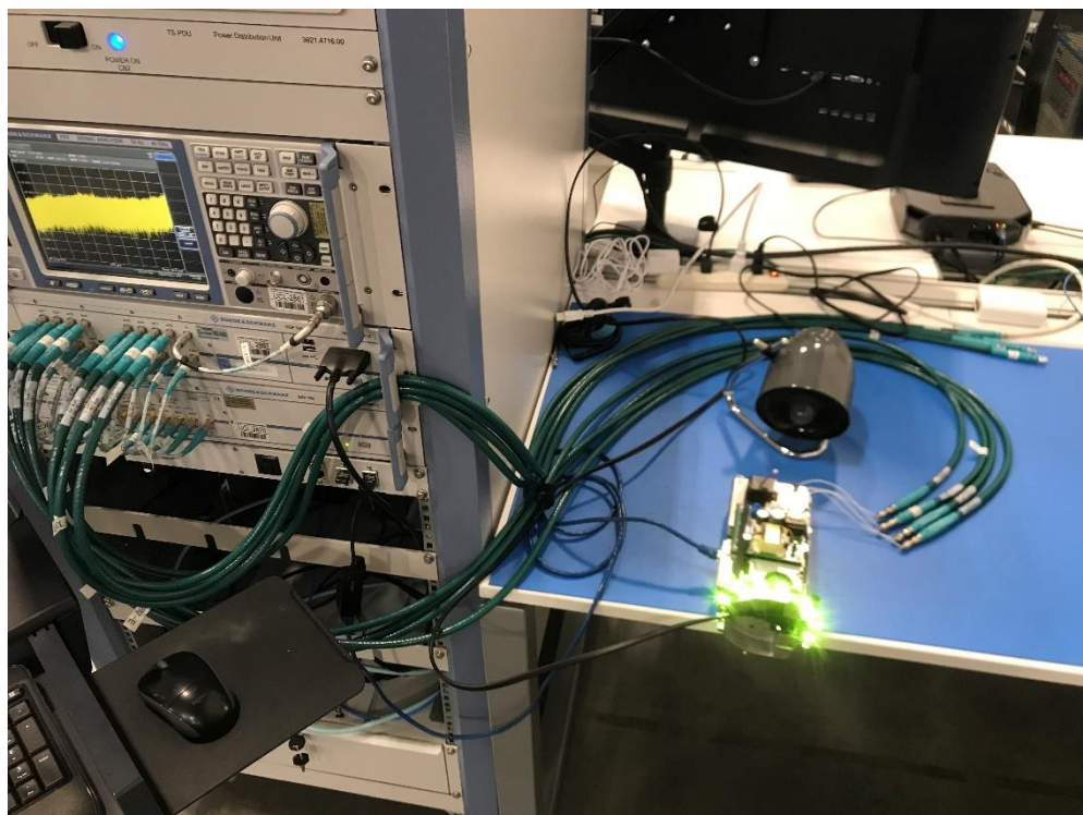
Photograph 1: RF Conducted Test Set Up
