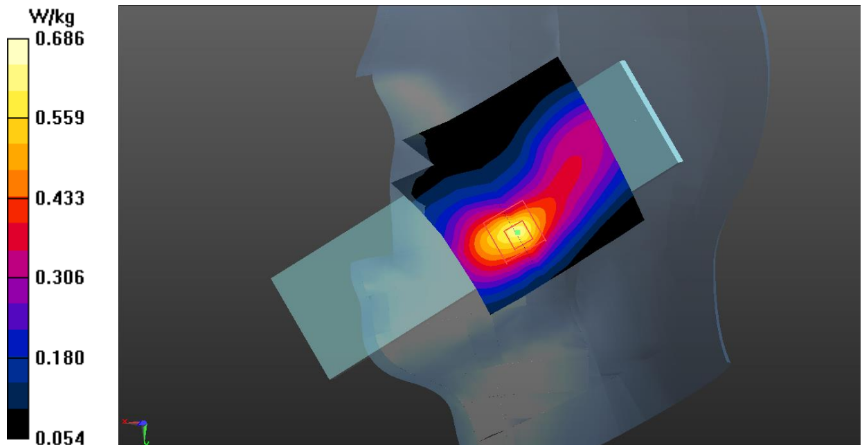
Fig.13 LTE Band 5 Head
