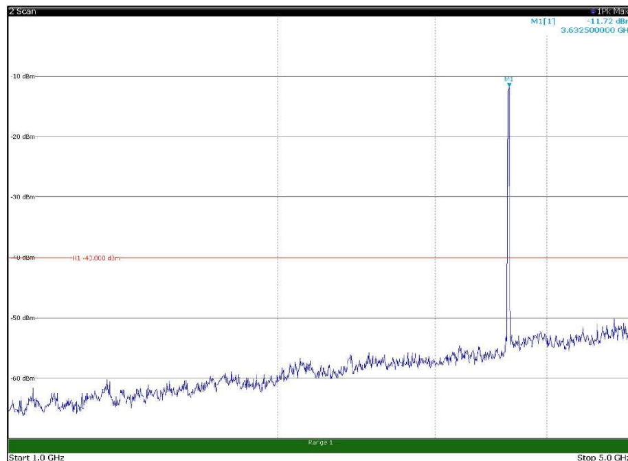
Channel: MIDDLE, Modulation: QPSK, BW=20MHz, Range: 1GHz - 5GHz, Polarization: Vertical
