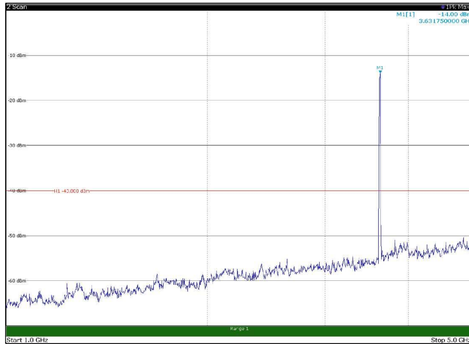
Channel: MIDDLE, Modulation: QPSK, BW=20MHz, Range: 1GHz - 5GHz, Polarization: Horizontal
