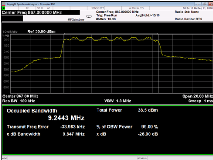
Figure 350: 16QAM 10MHz B.W.; 867.0MHz, 15kHz- Output
