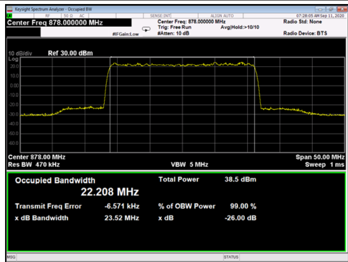
Figure 424: 64QAM 25MHz B.W.; 878.5MHz, 60kHz - Output
