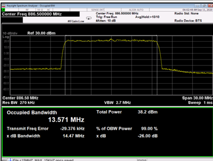
Figure 408: 64QAM 15MHz B.W.; 886.5MHz, 30kHz - Output
