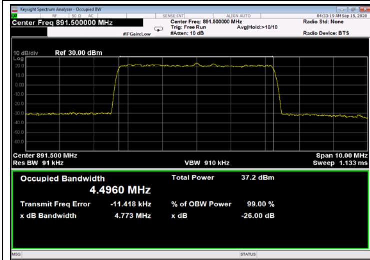
Figure 432: 256QAM 5MHz B.W.; 891.5MHz, 15kHz - Output
