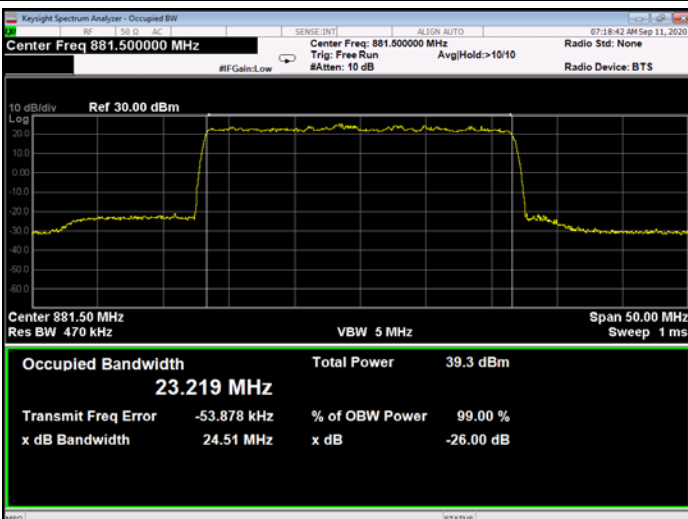
Figure 426: 64QAM 25MHz B.W.; 881.5MHz, 30kHz - Output
