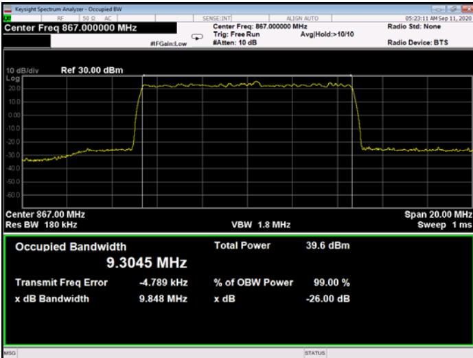
Figure 392: 64QAM 10MHz B.W.; 867.0MHz, 15kHz - Output
