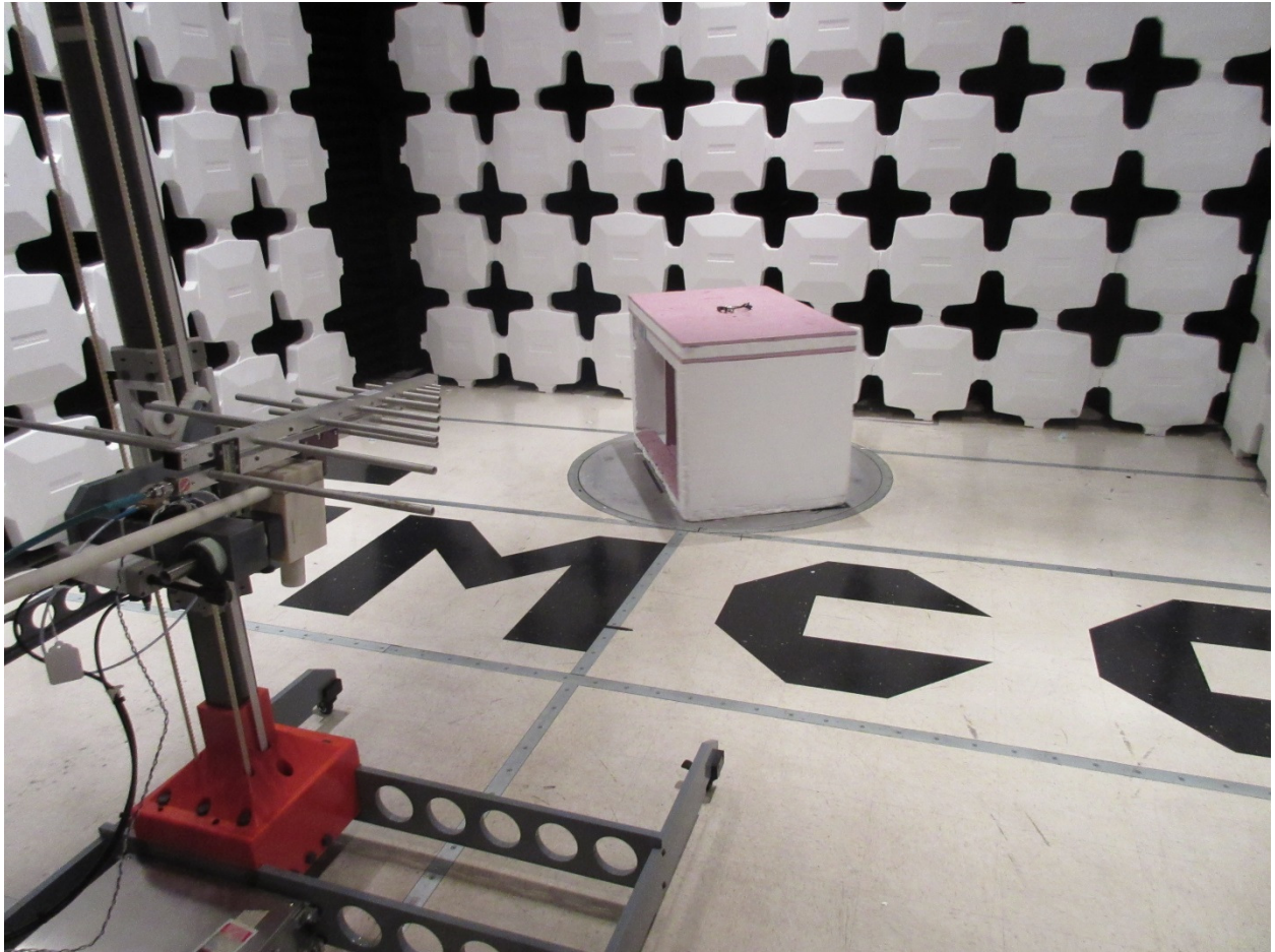
RADIATED EMISSIONS TEST SET UP PHOTO BELOW 1GHZ
