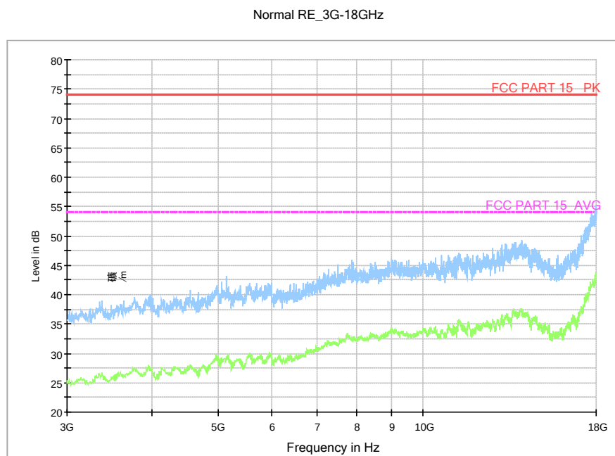
Fig.84. Radiated emission: 8DPSK, Channel 78, 3 GHz - 18 GHz
