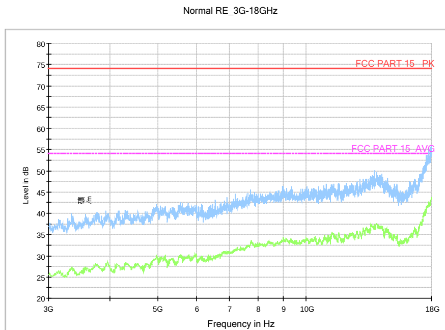
Fig.62. Radiated emission: GFSK, Channel 39, 3 GHz - 18 GHz
