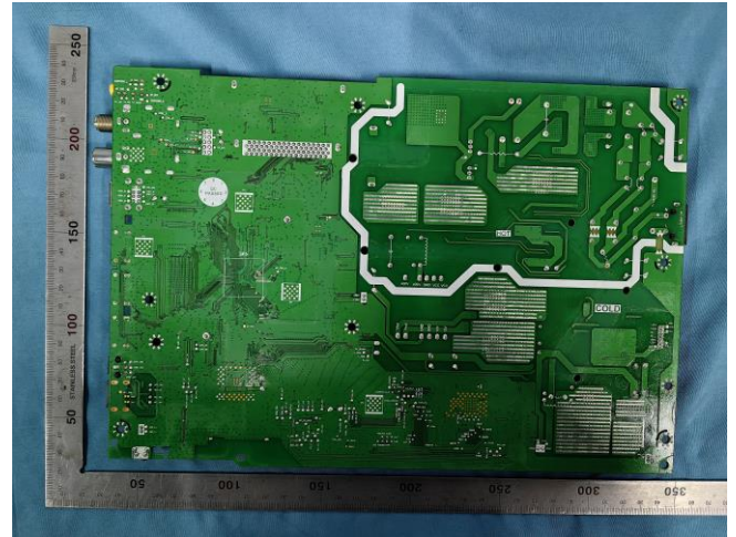
Test board 2
