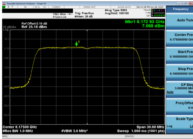
Plot 7-252. Power Spectral Density Plot Antenna WF7a Standard Power (20MHz 802.11ax (UNII Band 5) – Ch. 45, MCS4)
