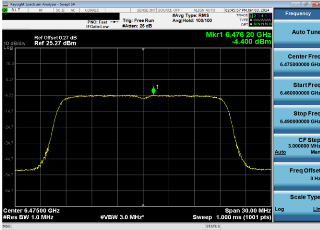
Plot 7-313. Power Spectral Density Plot Antenna WF2a LPI (20MHz 802.11ax (UNII Band 6) – Ch. 105, MCS11)
