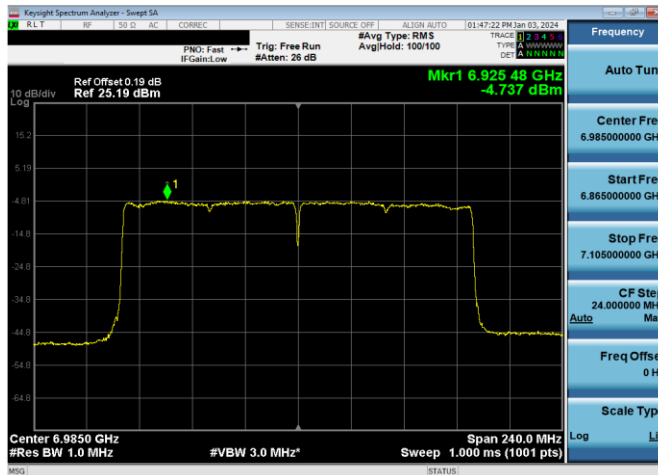
Plot 7-290. Power Spectral Density Plot Antenna WF2a LPI (160MHz 802.11ax (UNII Band 8) – Ch. 207, MCS2)
