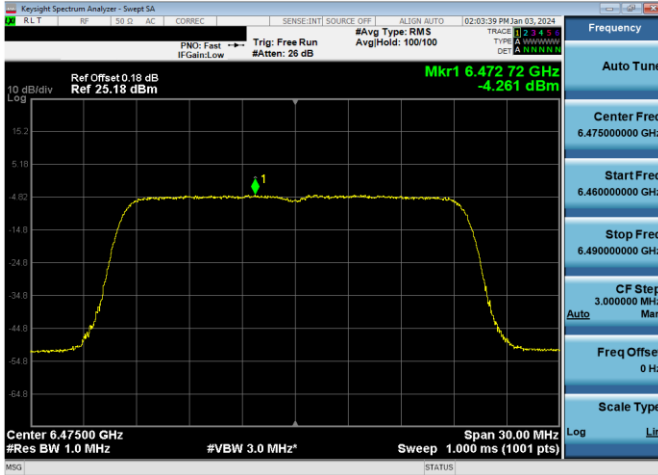
Plot 7-297. Power Spectral Density Plot Antenna WF2a LPI (20MHz 802.11ax (UNII Band 6) – Ch. 105, MCS4)
