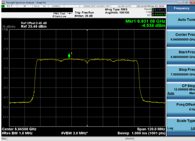
Plot 7-325. Power Spectral Density Plot Antenna WF2a LPI (80MHz 802.11ax (UNII Band 8) – Ch. 199, MCS11)
