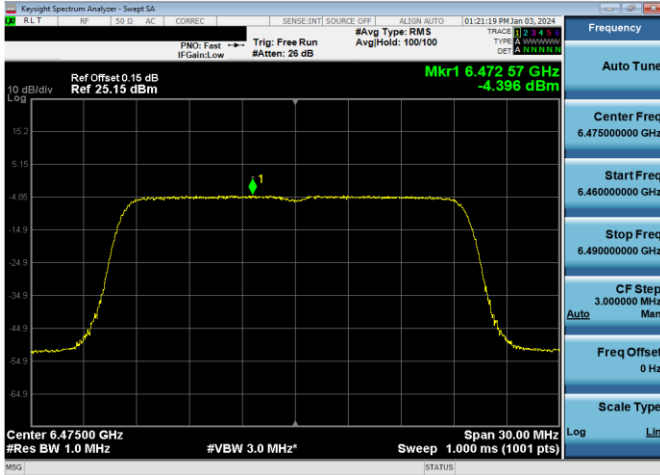
Plot 7-277. Power Spectral Density Plot Antenna WF2a LPI (20MHz 802.11ax (UNII Band 6) – Ch. 105, MCS2)
