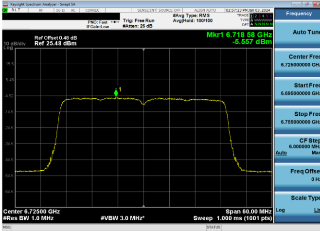
Plot 7-319. Power Spectral Density Plot Antenna WF2a LPI (40MHz 802.11ax (UNII Band 7) – Ch. 155, MCS11)
