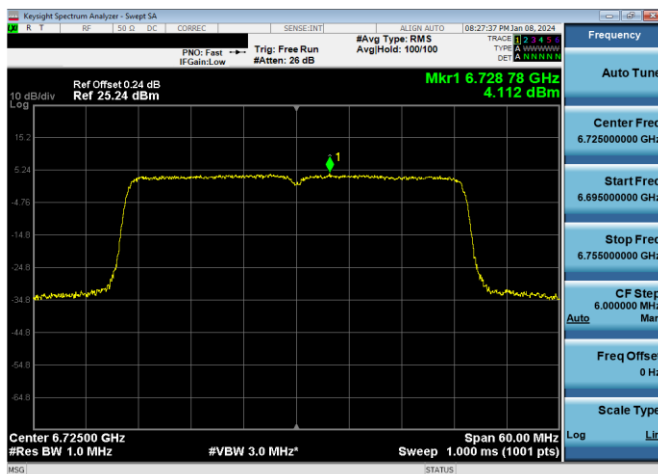
Plot 7-258. Power Spectral Density Plot Antenna WF7a Standard Power (40MHz 802.11ax (UNII Band 7) – Ch. 155, MCS4)
