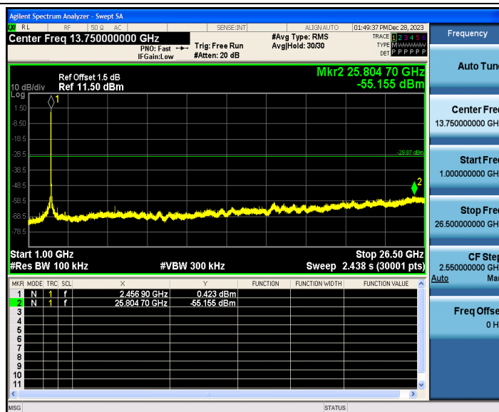
802.11n(HT20)_Ant2_2462_0~Reference
