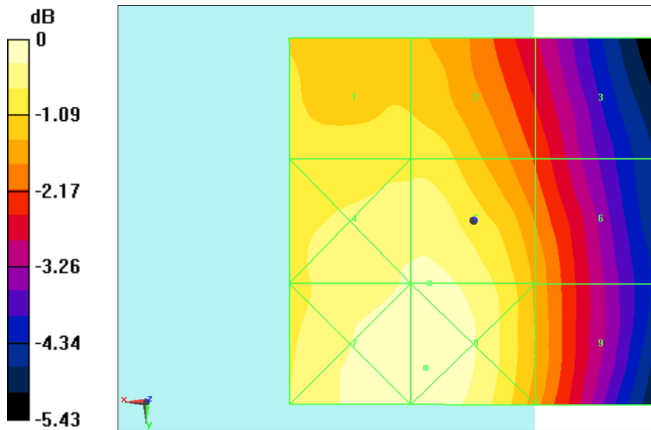
Fig B.2 HAC RF E-Field GSM1900
