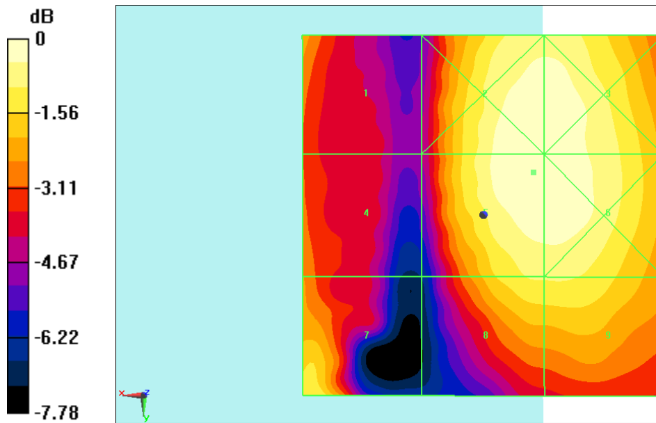
Fig B.4 HAC RF E-Field LTE Band41 PC3 QPSK
