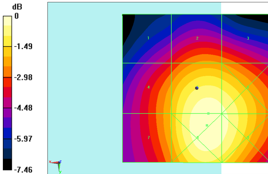
Fig B.5 HAC RF E-Field WIFI2.4G
