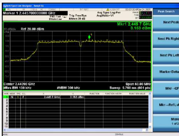
VHT-40 MHz CHANNEL 7, CARRIER LEVEL
