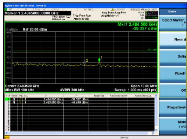
802.11n-40 MHz CHANNEL 8, BAND EDGE
