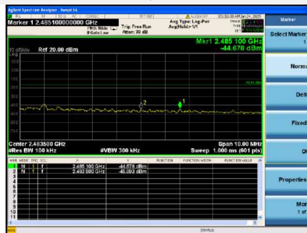
VHT-40 MHz CHANNEL 7, BAND EDGE
