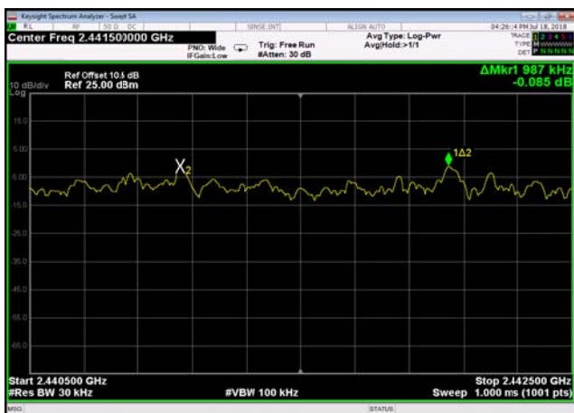
pi/4DQPSK,Hopping2DH5,2440.5~2442.5
