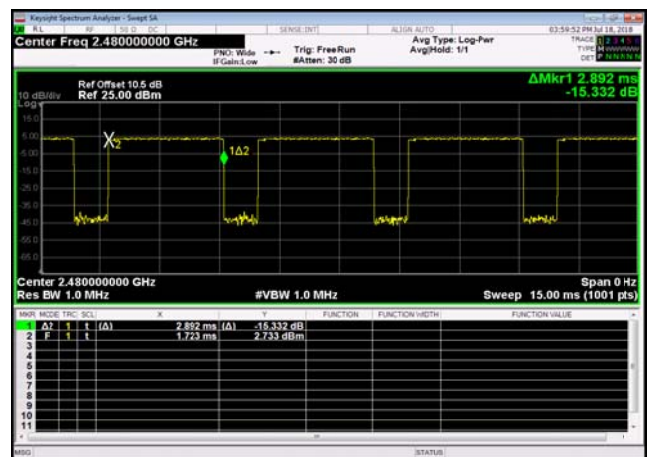
pi/4DQPSK,2480,2DH5,Transmission Time
