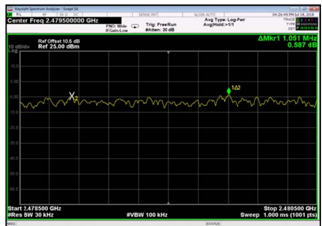
pi/4DQPSK,Hopping2DH5,2478.5~2480.5
