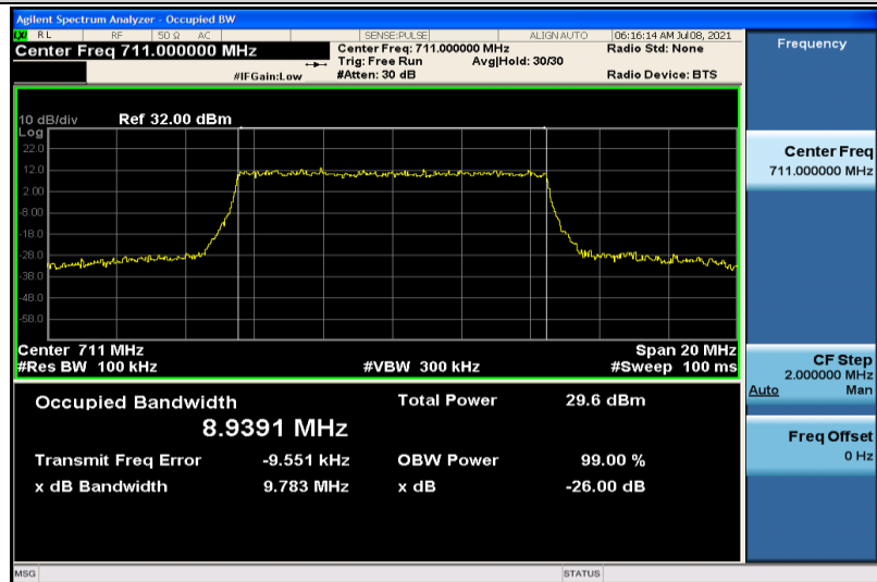
Band17-10MHz-QPSK-23800-50RB#0-8.9391
