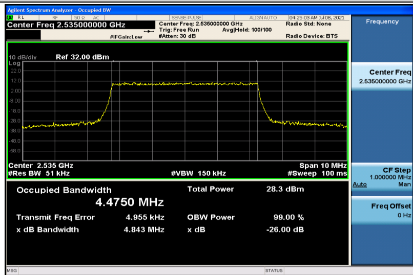
Band7-5MHz-16QAM-21100-25RB#0-4.4750
