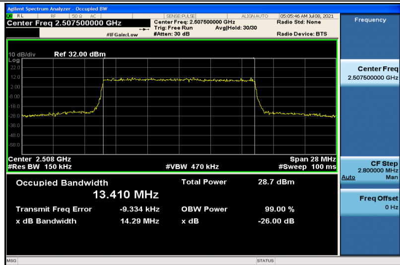
Band7-15MHz-16QAM-20825-75RB#0-13.410
