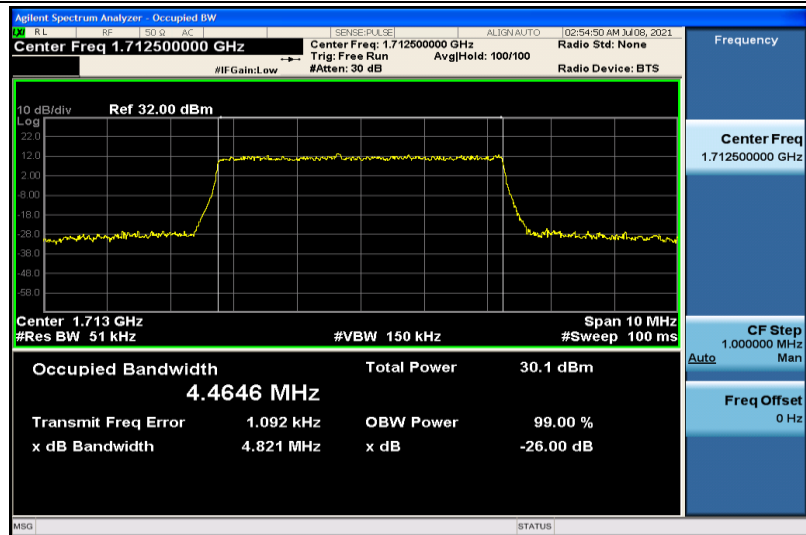
Band4-5MHz-QPSK-19975-25RB#0-4.4646
