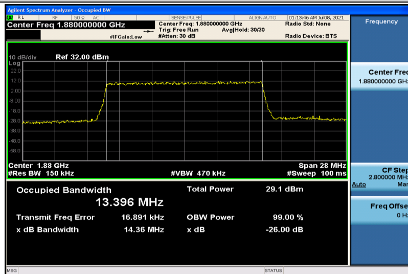
Band2-15MHz-16QAM-18900-75RB#0-13.396
