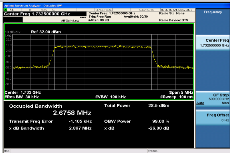
Band4-3MHz-16QAM-20175-15RB#0-2.6758
