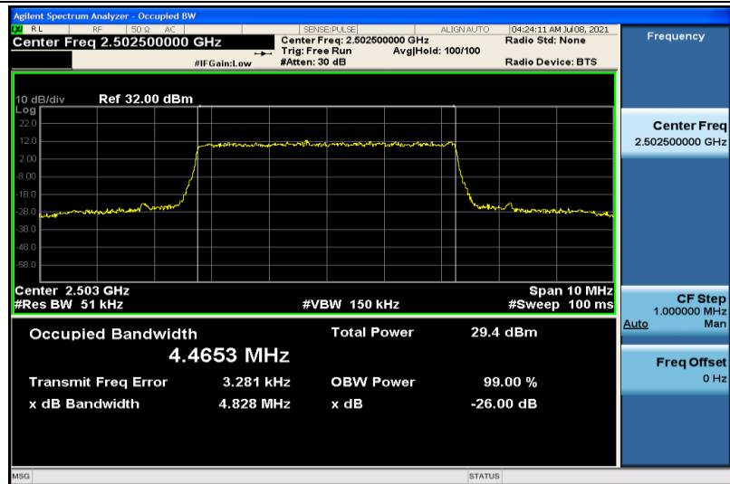
Band7-5MHz-QPSK-20775-25RB#0-4.4653
