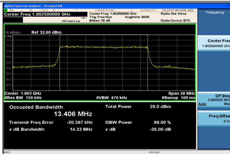
Band2-15MHz-16QAM-19125-75RB#0-13.406
