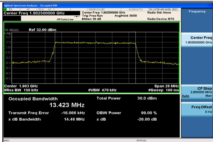
Band2-15MHz-QPSK-19125-75RB#0-13.423
