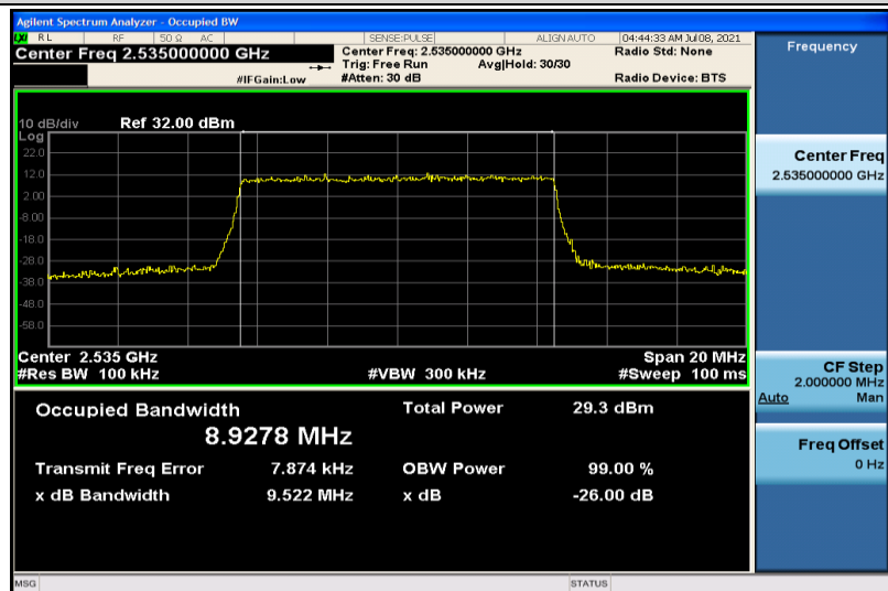
Band7-10MHz-QPSK-21100-50RB#0-8.9278
