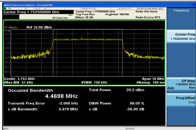
Band4-5MHz-16QAM-20375-25RB#0-4.4698
