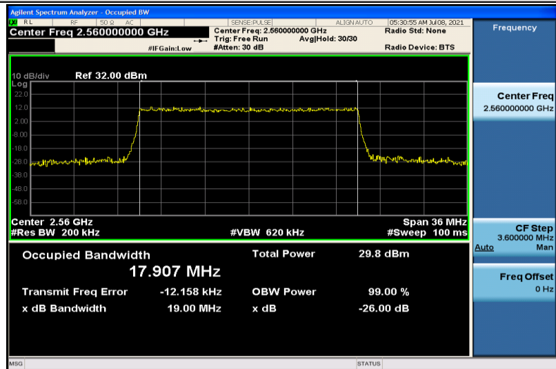
Band7-20MHz-QPSK-21350-100RB#0-17.907
