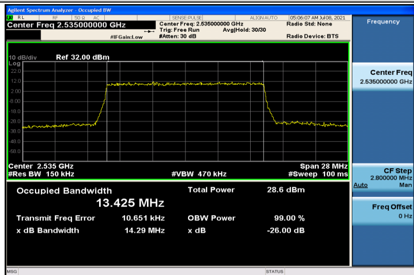
Band7-15MHz-16QAM-21100-75RB#0-13.425
