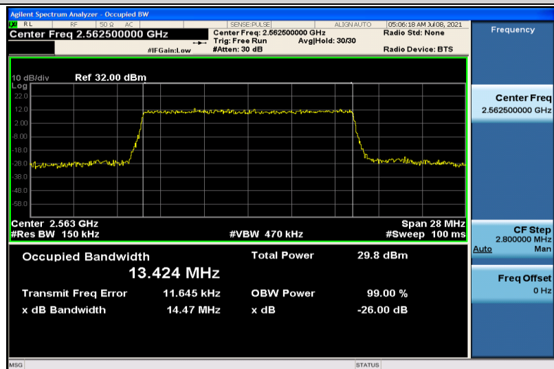
Band7-15MHz-QPSK-21375-75RB#0-13.424
