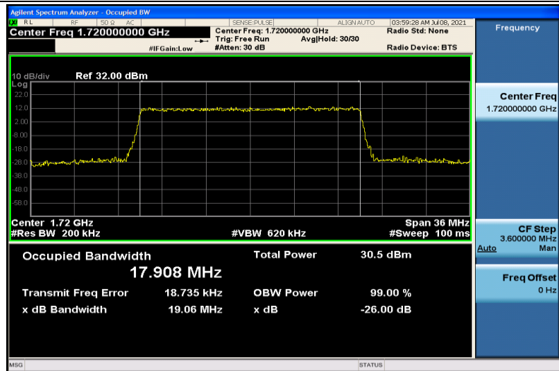
Band4-20MHz-QPSK-20050-100RB#0-17.908
