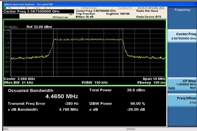
Band7-5MHz-16QAM-21425-25RB#0-4.4650
