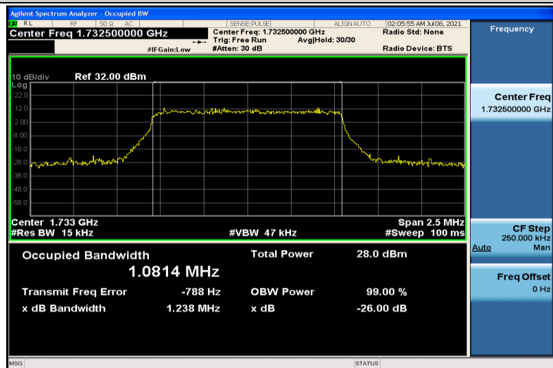
Band4-1.4MHz-16QAM-20175-6RB#0-1.0814
