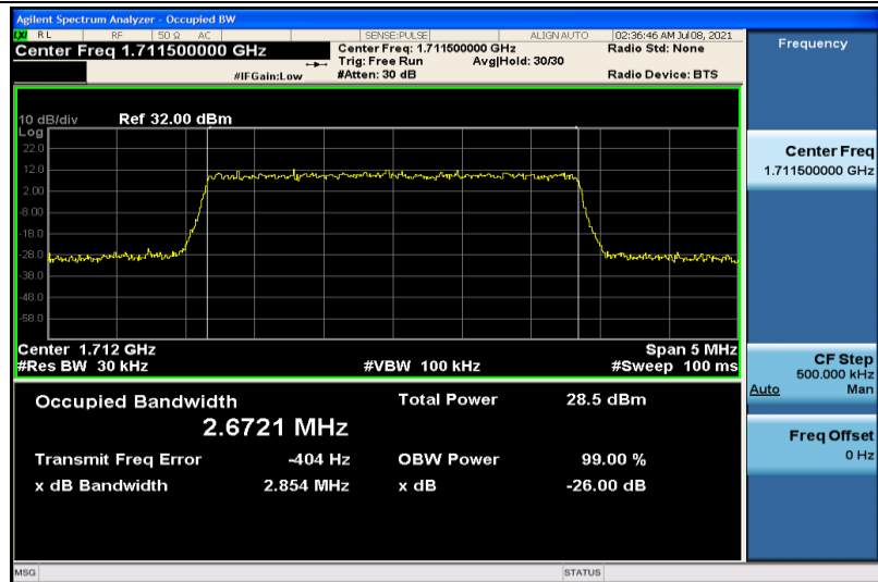
Band4-3MHz-16QAM-19965-15RB#0-2.6721
