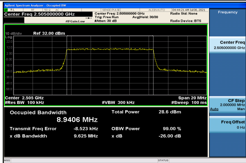
Band7-10MHz-16QAM-20800-50RB#0-8.9406
