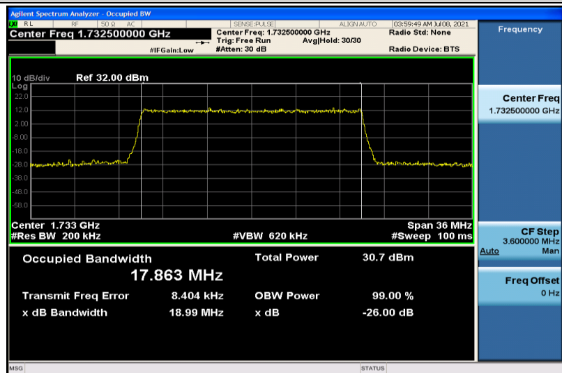
Band4-20MHz-QPSK-20175-100RB#0-17.863
