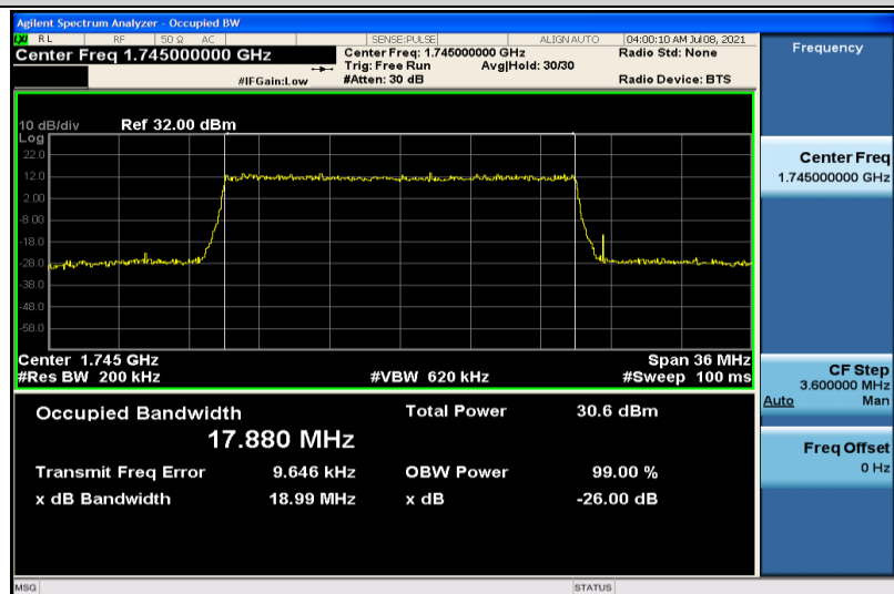
Band4-20MHz-QPSK-20300-100RB#0-17.880
