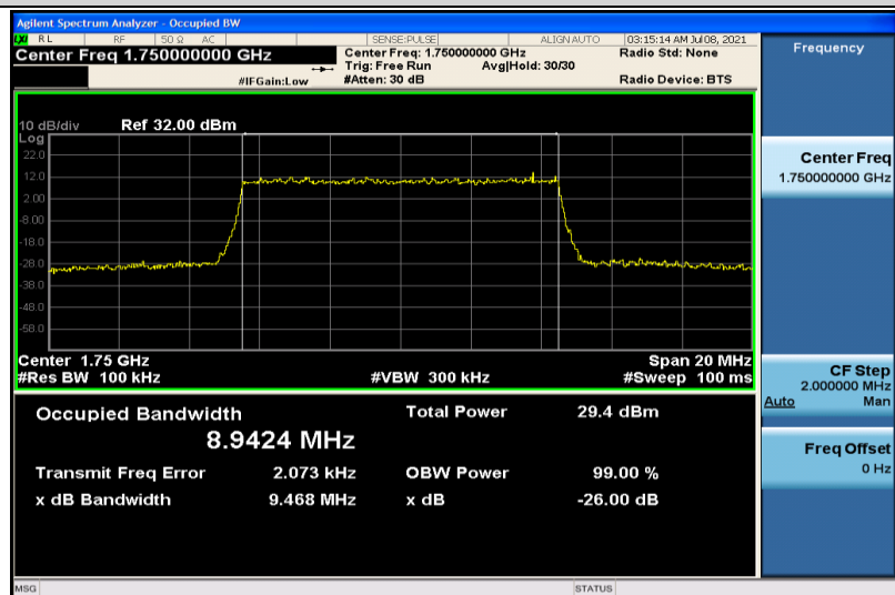
Band4-10MHz-16QAM-20350-50RB#0-8.9424
