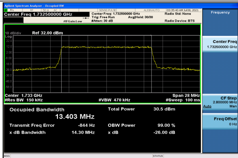
Band4-15MHz-QPSK-20175-75RB#0-13.403
