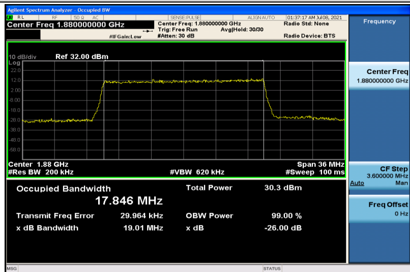
Band2-20MHz-QPSK-18900-100RB#0-17.846
