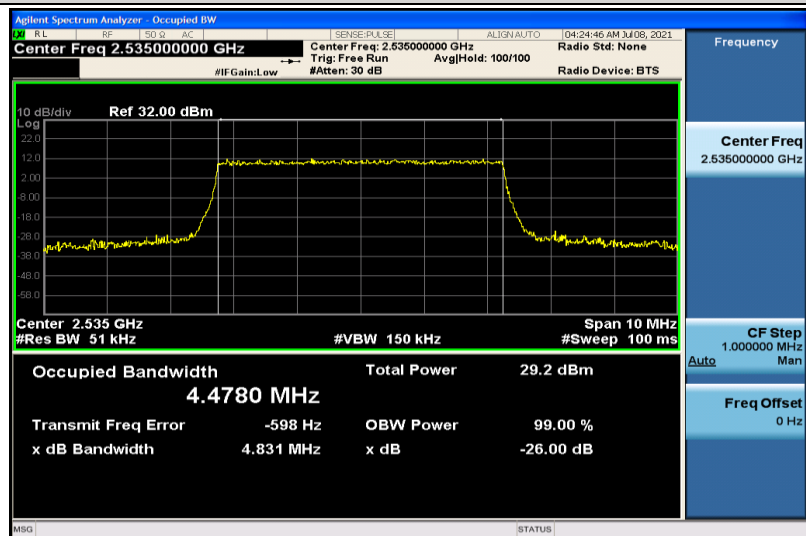
Band7-5MHz-QPSK-21100-25RB#0-4.4780
