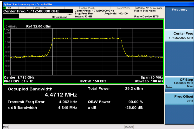
Band4-5MHz-16QAM-19975-25RB#0-4.4712
