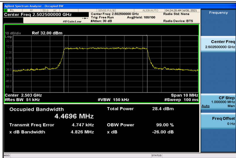
Band7-5MHz-16QAM-20775-25RB#0-4.4696
