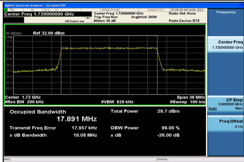
Band4-20MHz-16QAM-20050-100RB#0-17.891
