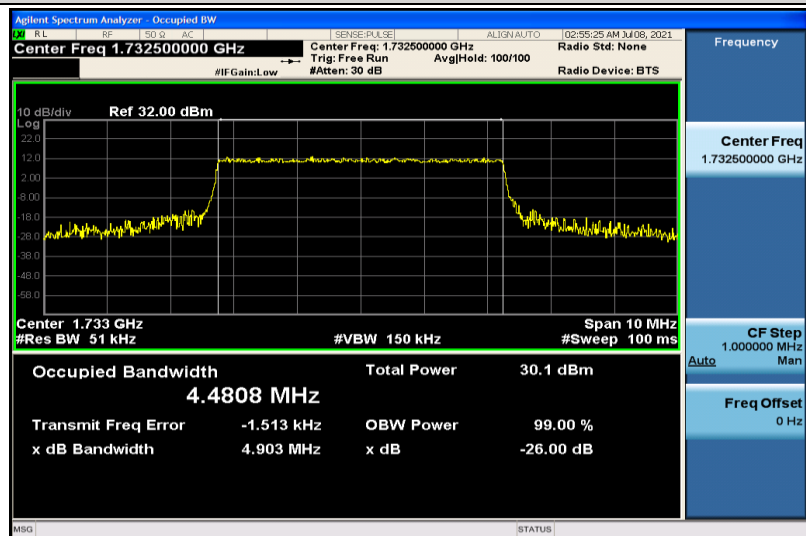
Band4-5MHz-QPSK-17325-25RB#0-4.4808
