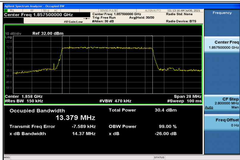
Band2-15MHz-QPSK-18675-75RB#0-13.379
