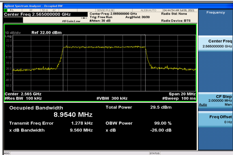
Band7-10MHz-QPSK-21400-50RB#0-8.9540
