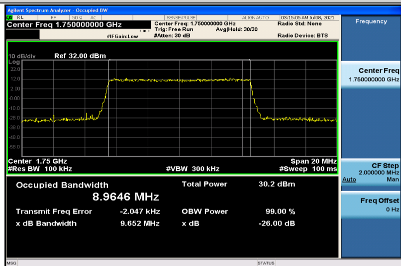
Band4-10MHz-QPSK-20350-50RB#0-8.9646
