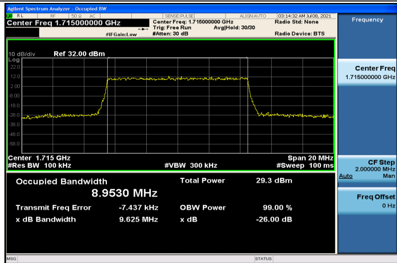
Band4-10MHz-16QAM-20000-50RB#0-8.9530
