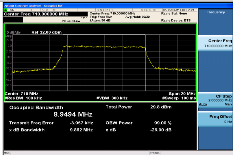
Band17-10MHz-QPSK-23790-50RB#0-8.9494
