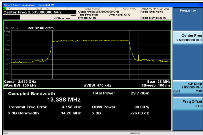
Band7-15MHz-QPSK-21100-75RB#0-13.388
