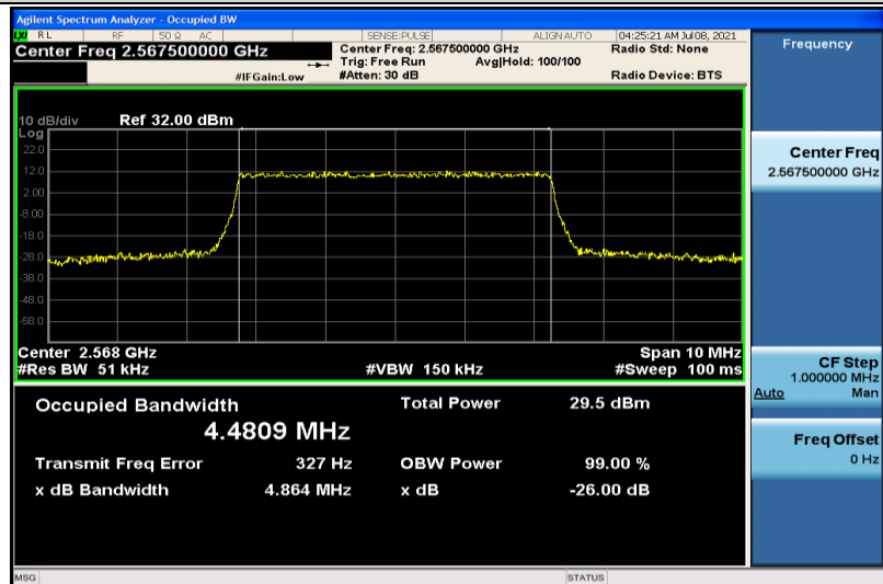
Band7-5MHz-QPSK-21425-25RB#0-4.4809
