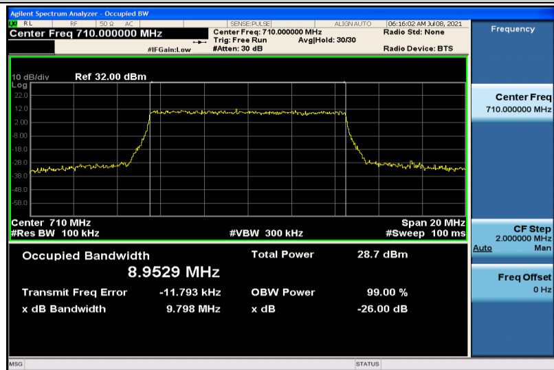
Band17-10MHz-16QAM-23790-50RB#0-8.9529
