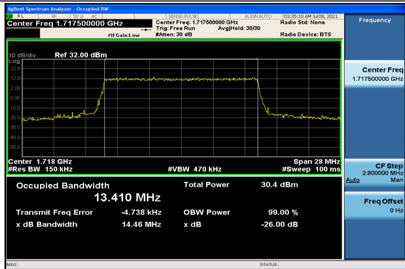
Band4-15MHz-QPSK-20025-75RB#0-13.410
