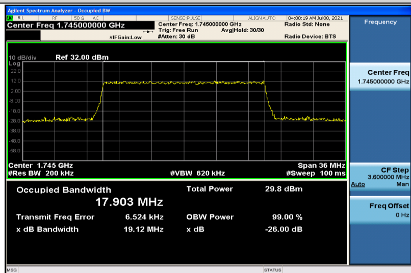
Band4-20MHz-16QAM-20300-100RB#0-17.903
