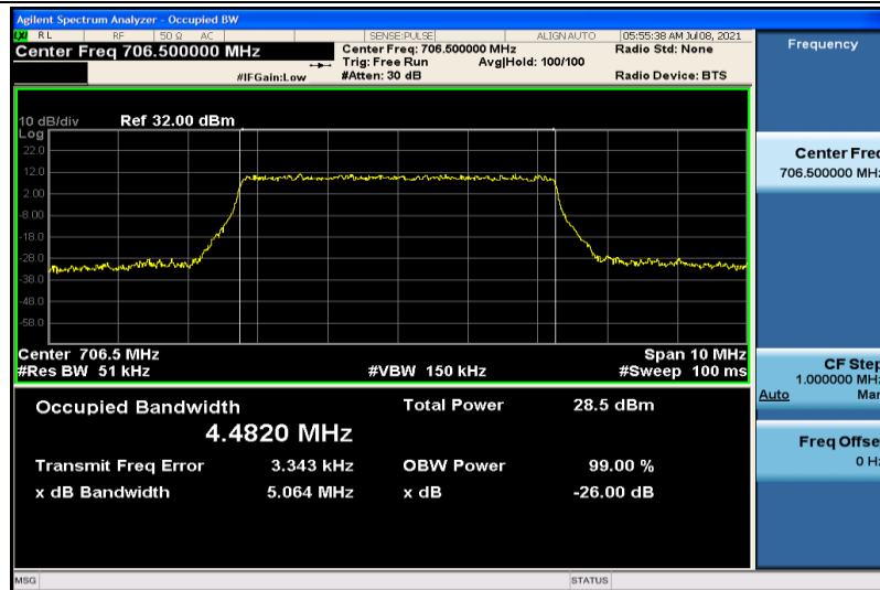
Band17-5MHz-16QAM-23755-25RB#0-4.4820
