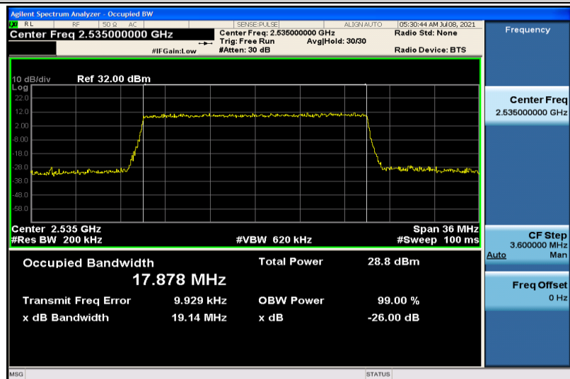
Band7-20MHz-16QAM-21100-100RB#0-17.878
