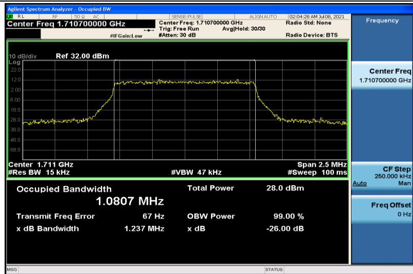
Band4-1.4MHz-16QAM-19957-6RB#0-1.0807
