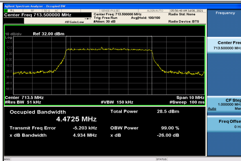
Band17-5MHz-16QAM-23825-25RB#0-4.4725
