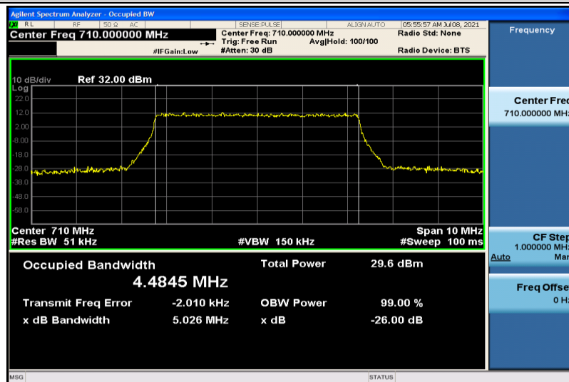
Band17-5MHz-QPSK-23790-25RB#0-4.4845
