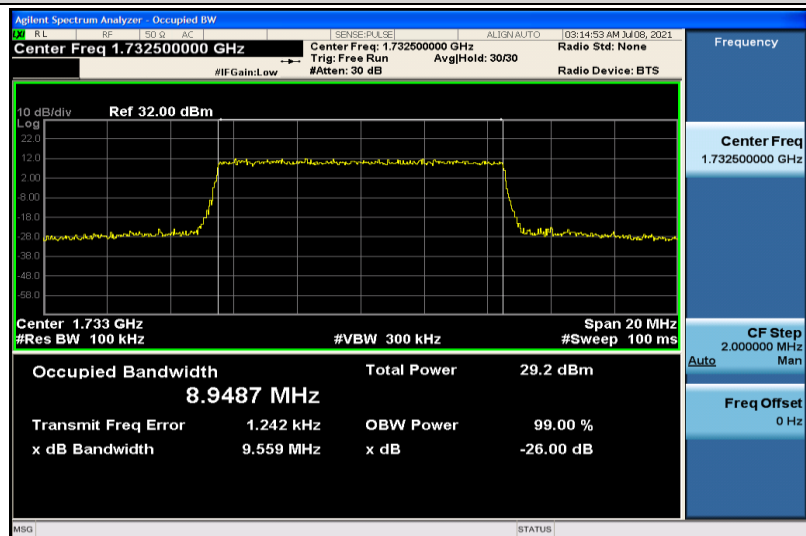
Band4-10MHz-16QAM-20175-50RB#0-8.9487
