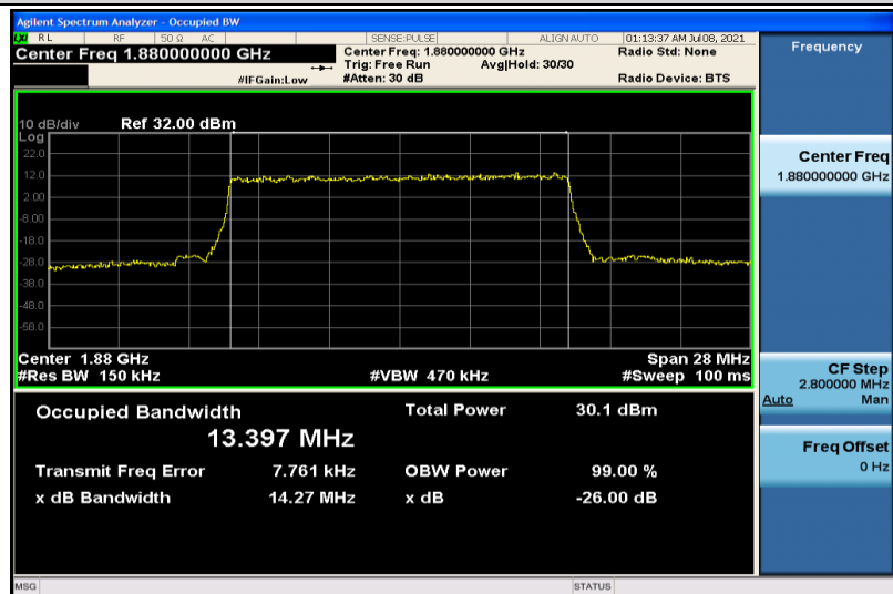
Band2-15MHz-QPSK-18900-75RB#0-13.397
