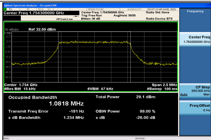
Band4-1.4MHz-QPSK-20393-6RB#0-1.0818
