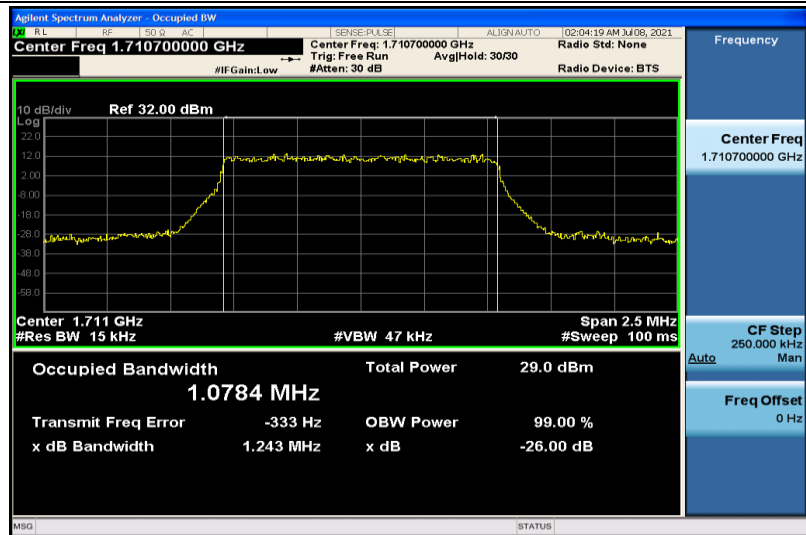
Band4-1.4MHz-QPSK-19957-6RB#0-1.0784
