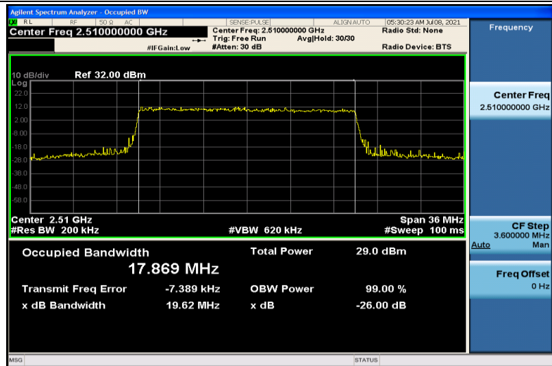
Band7-20MHz-16QAM-20850-100RB#0-17.869
