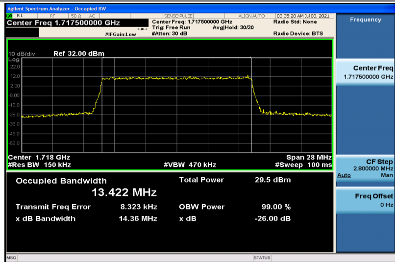
Band4-15MHz-16QAM-20025-75RB#0-13.422
