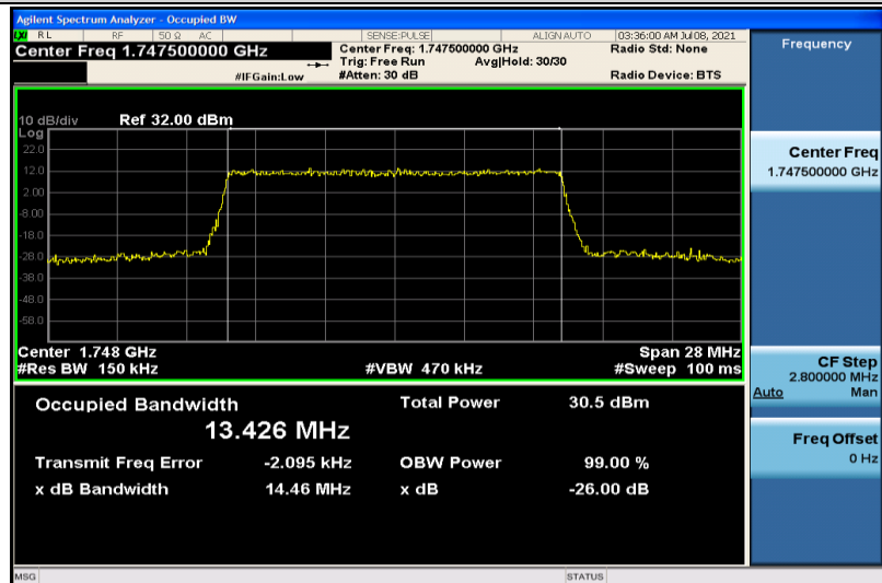
Band4-15MHz-QPSK-20325-75RB#0-13.426
