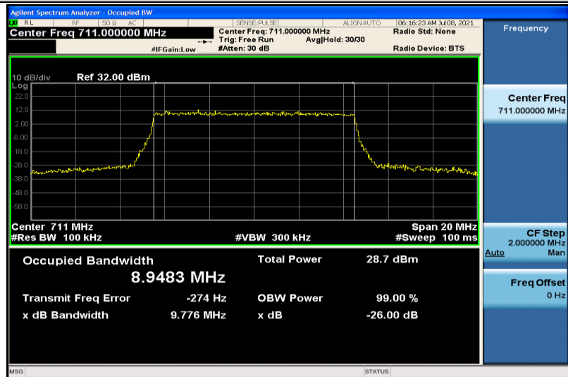
Band17-10MHz-16QAM-23800-50RB#0-8.9483
