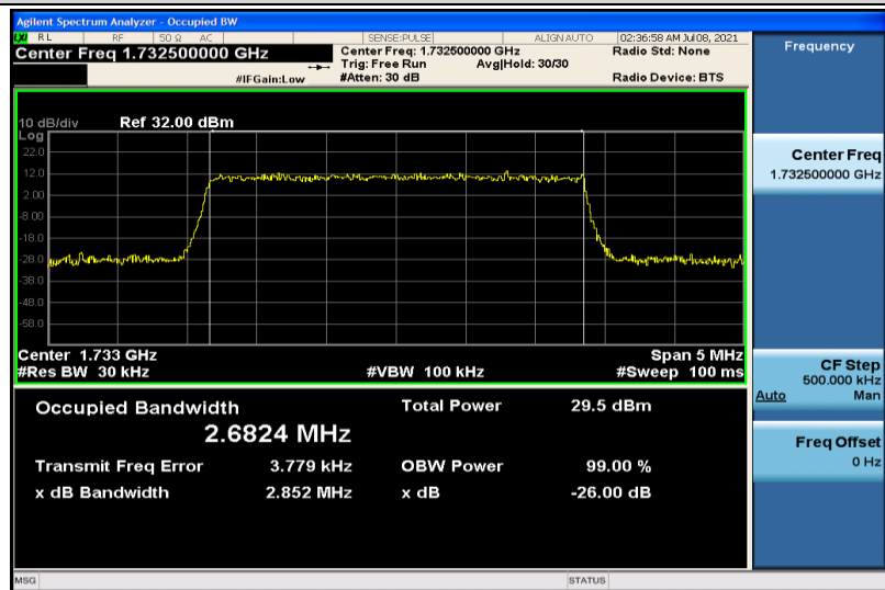
Band4-3MHz-QPSK-20175-15RB#0-2.6824
