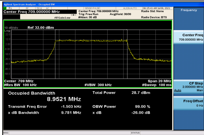
Band17-10MHz-16QAM-23780-50RB#0-8.9521
