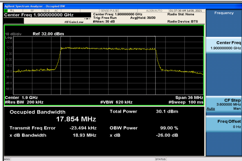
Band2-20MHz-QPSK-19100-100RB#0-17.854
