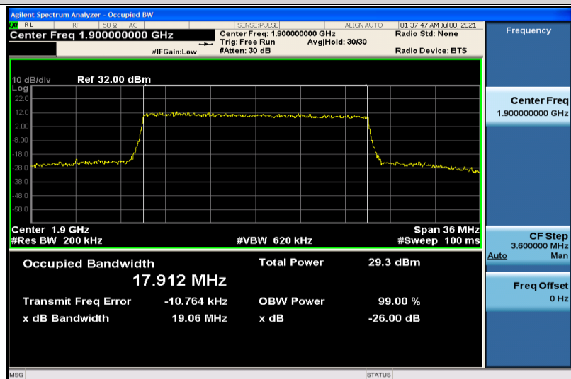
Band2-20MHz-16QAM-19100-100RB#0-17.912
