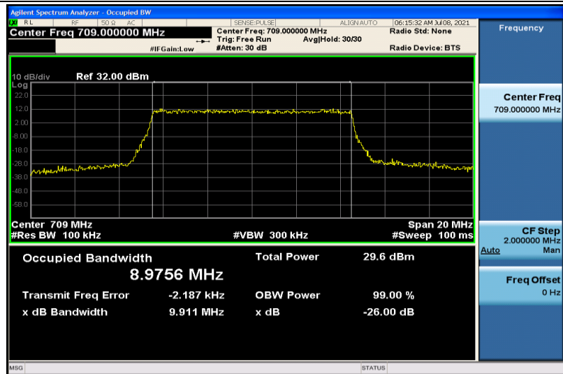
Band17-10MHz-QPSK-23780-50RB#0-8.9756
