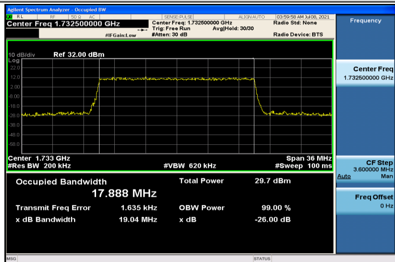
Band4-20MHz-16QAM-20175-100RB#0-17.888
