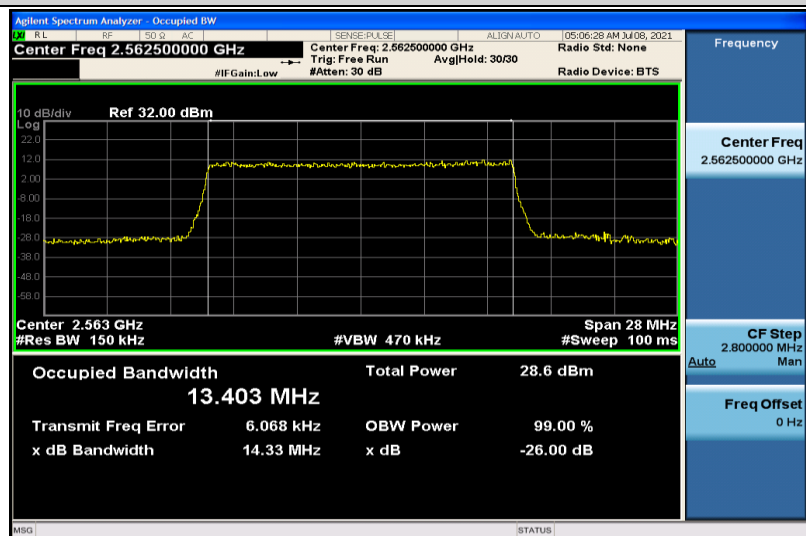
Band7-15MHz-16QAM-21375-75RB#0-13.403
