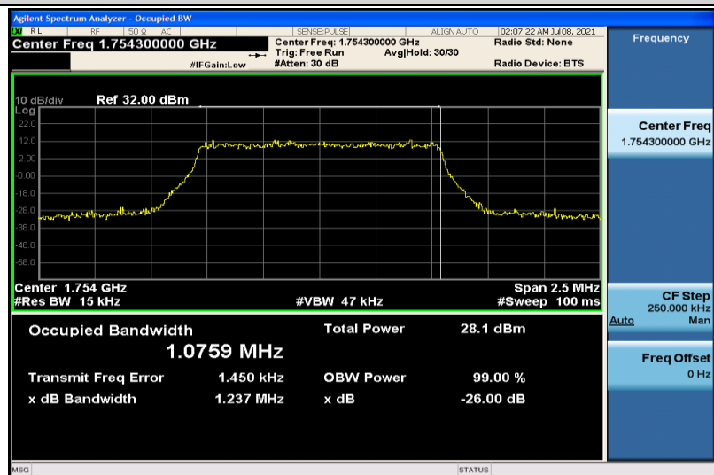
Band4-1.4MHz-16QAM-20393-6RB#0-1.0759
