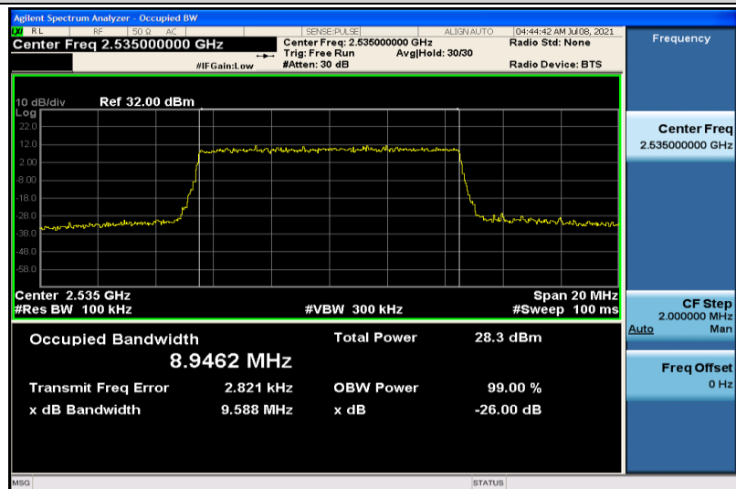
Band7-10MHz-16QAM-21100-50RB#0-8.9462
