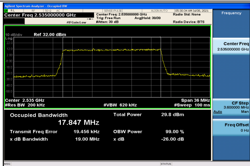
Band7-20MHz-QPSK-21100-100RB#0-17.847
