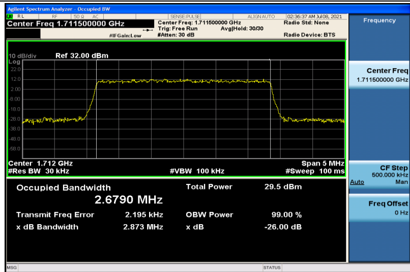
Band4-3MHz-QPSK-19965-15RB#0-2.6790
