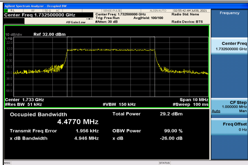
Band4-5MHz-16QAM-20175-25RB#0-4.4770
