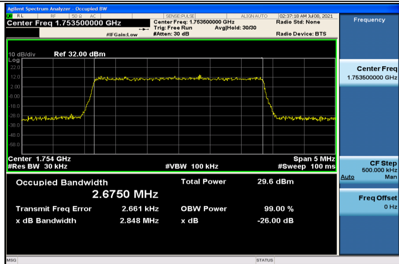
Band4-3MHz-QPSK-20385-15RB#0-2.6750
