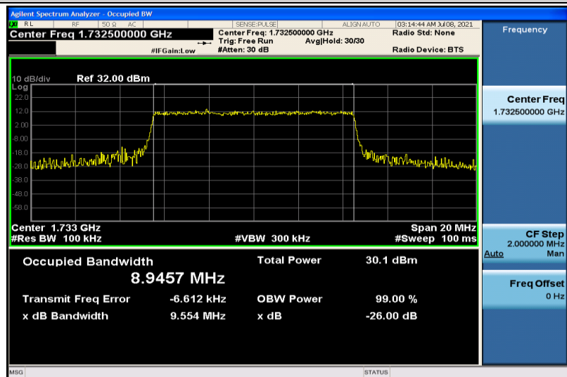
Band4-10MHz-QPSK-20175-50RB#0-8.9457
