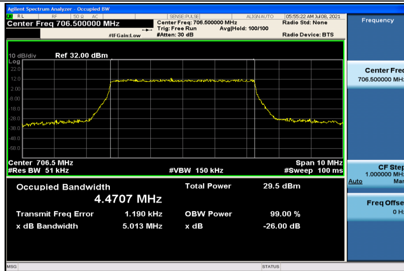
Band17-5MHz-QPSK-23755-25RB#0-4.4707
