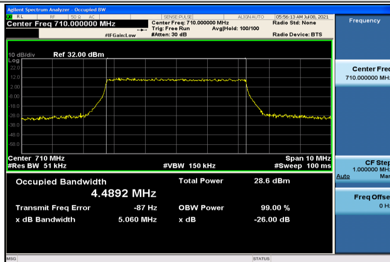
Band17-5MHz-16QAM-23790-25RB#0-4.4892
