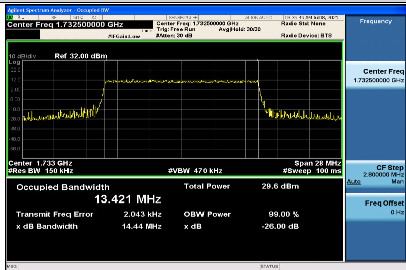
Band4-15MHz-16QAM-20175-75RB#0-13.421
