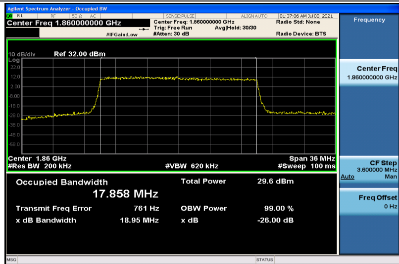
Band2-20MHz-16QAM-18700-100RB#0-17.858
