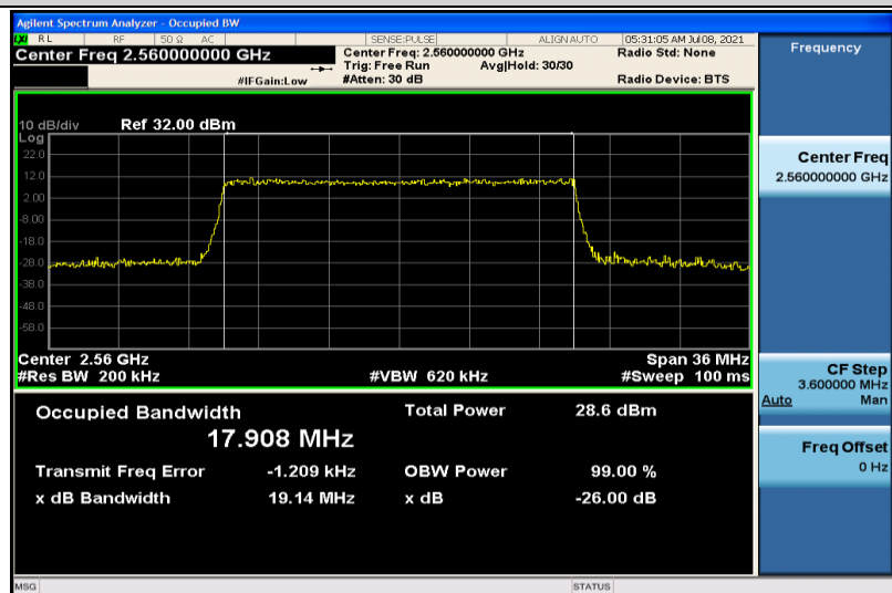
Band7-20MHz-16QAM-21350-100RB#0-17.908
