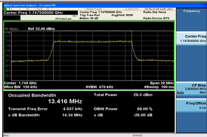
Band4-15MHz-16QAM-20325-75RB#0-13.416
