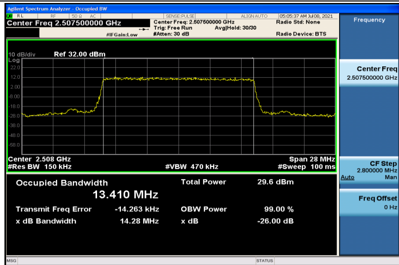
Band7-15MHz-QPSK-20825-75RB#0-13.410
