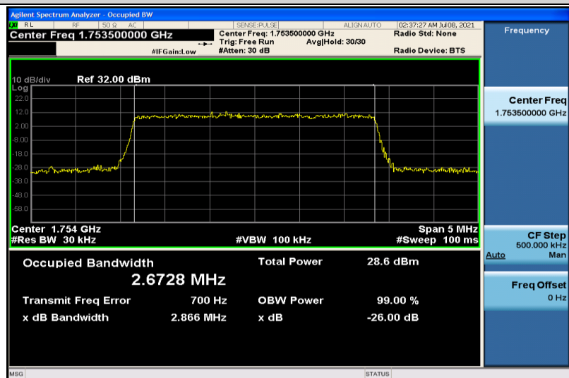
Band4-3MHz-16QAM-20385-15RB#0-2.6728
