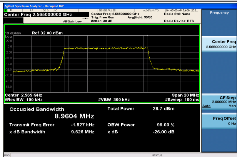
Band7-10MHz-16QAM-21400-50RB#0-8.9604
