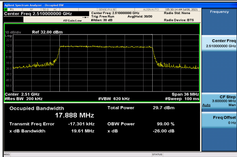
Band7-20MHz-QPSK-20850-100RB#0-17.888
