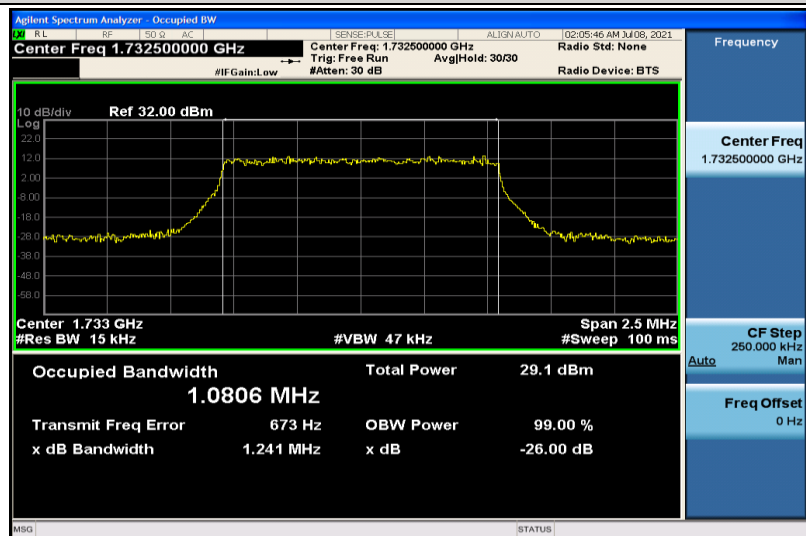
Band4-1.4MHz-QPSK-20175-6RB#0-1.0806
