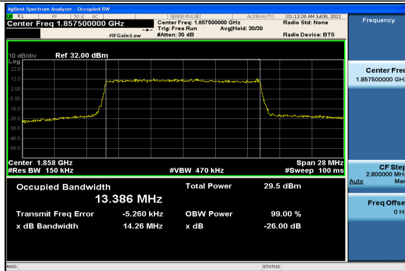
Band2-15MHz-16QAM-18675-75RB#0-13.386
