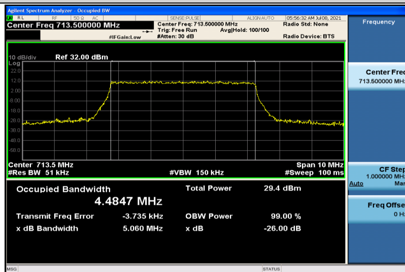
Band17-5MHz-QPSK-23825-25RB#0-4.4847
