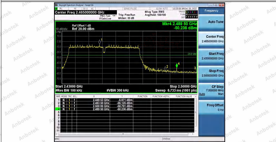
11N40_Ant1_High_2452
