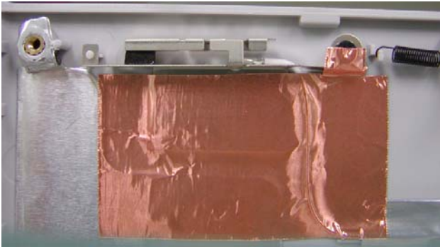
Aux antenna
