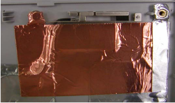
Main and Aux Antenna Photo: Main antenna
