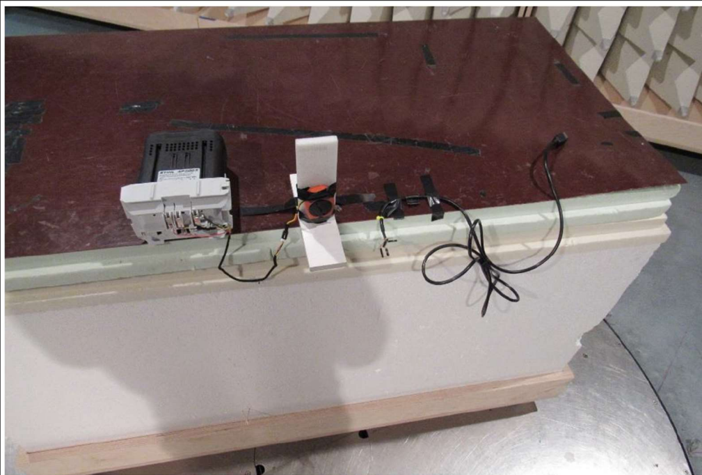
Test Setup Near View Below 1GHz
