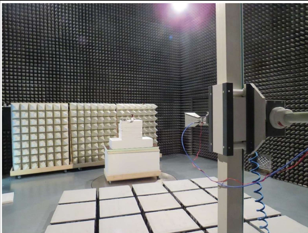
Test setup Radiated Emissions 6.5 - 18 GHz
