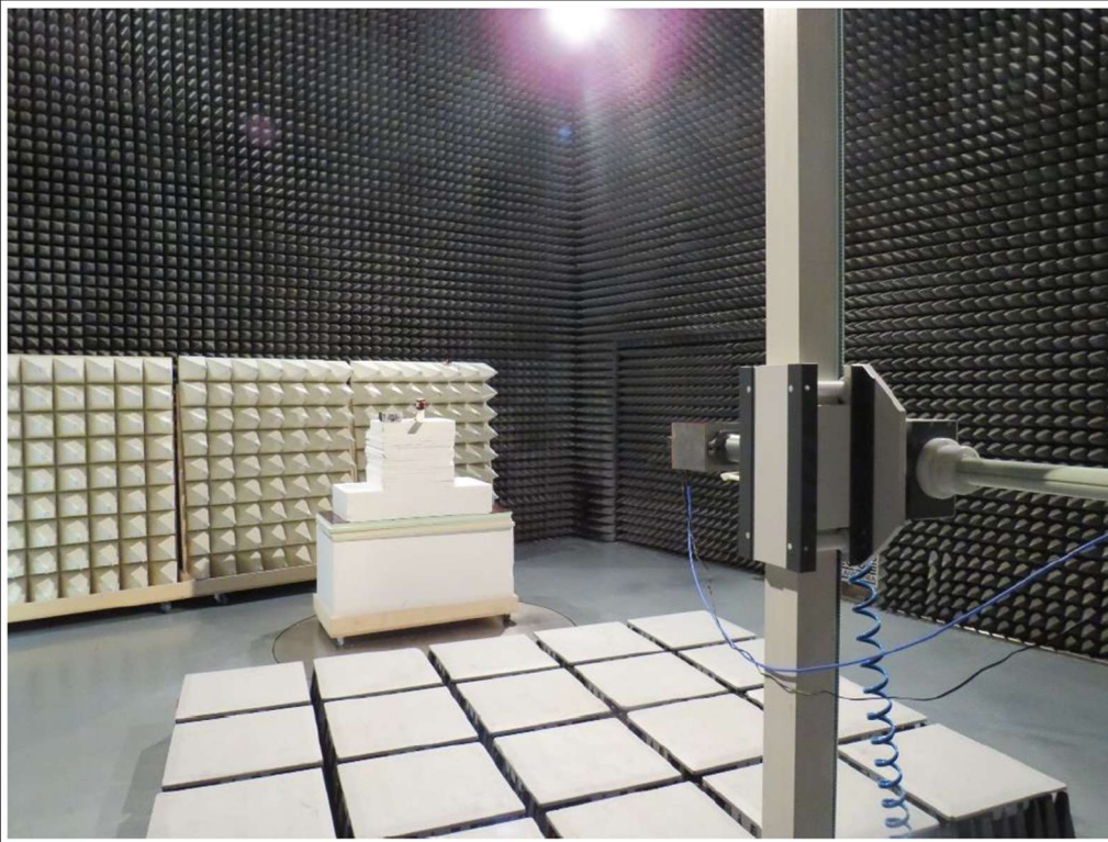
Test Setup Radiated Emissions above 18 GHz
