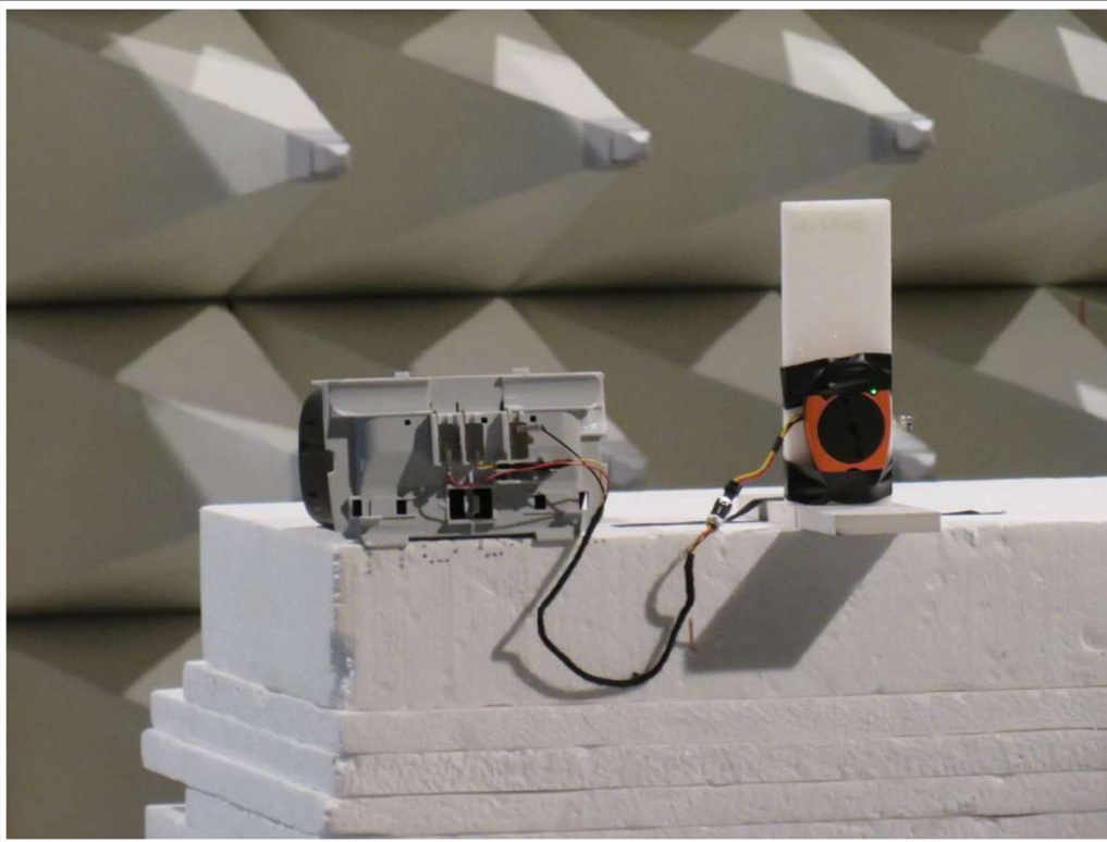
Test Setup Near View Above 1GHz - EUT vertical
