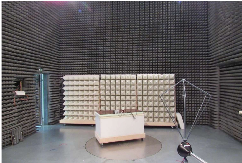
Test Setup Radiated Emissions below 200 MHz
