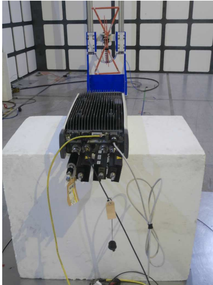
Radiated Emissions 30 MHz to 1 GHz
