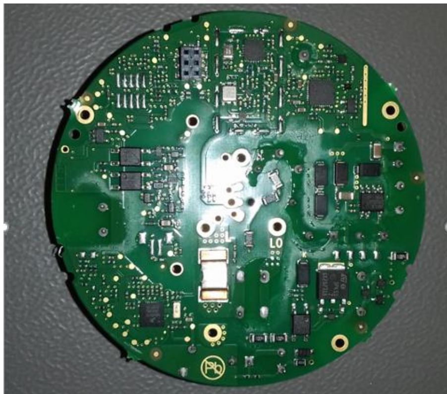
Figure 2 Main PCB bottom
