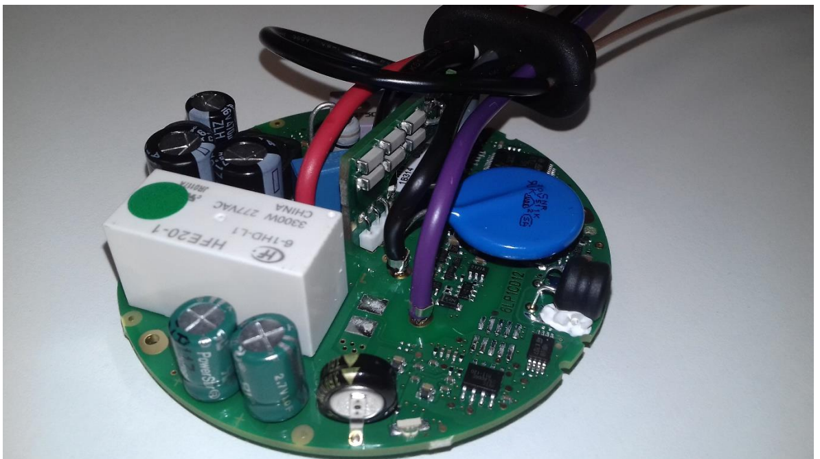
Figure 8 Internal assembly
