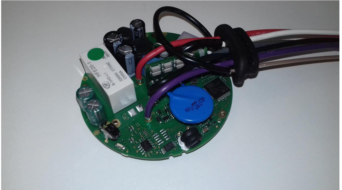
Figure 7 Internal assembly
