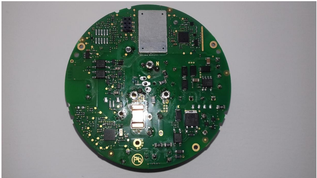
Figure 1 Main PCB bottom
