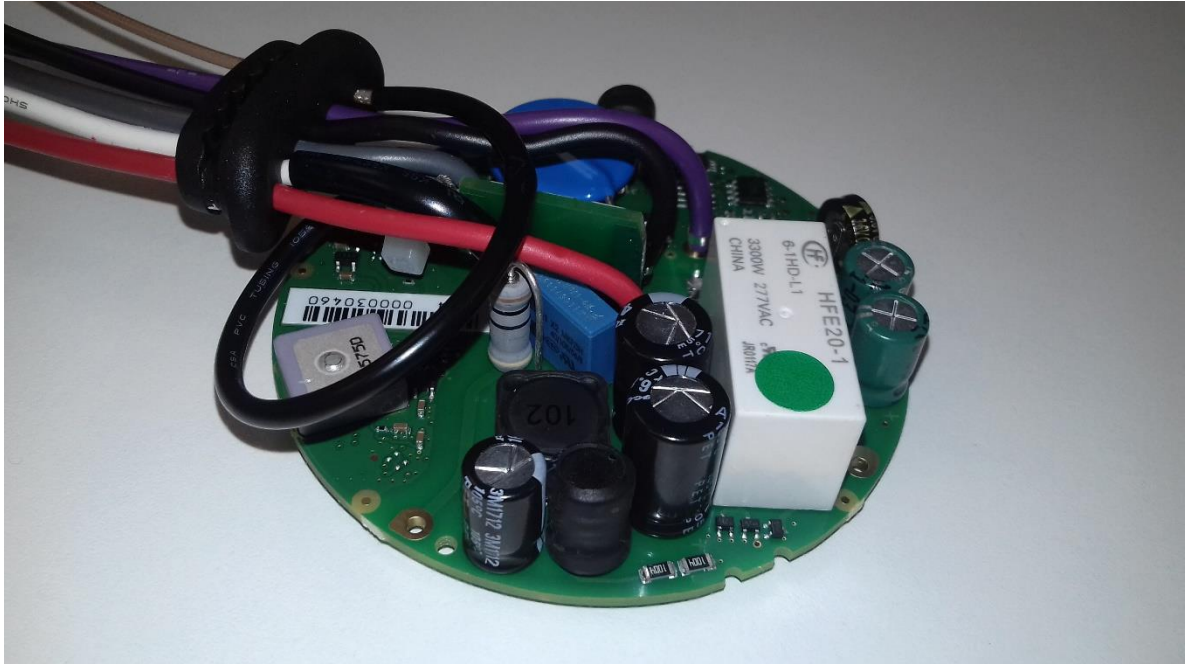
Figure 9 Internal assembly
