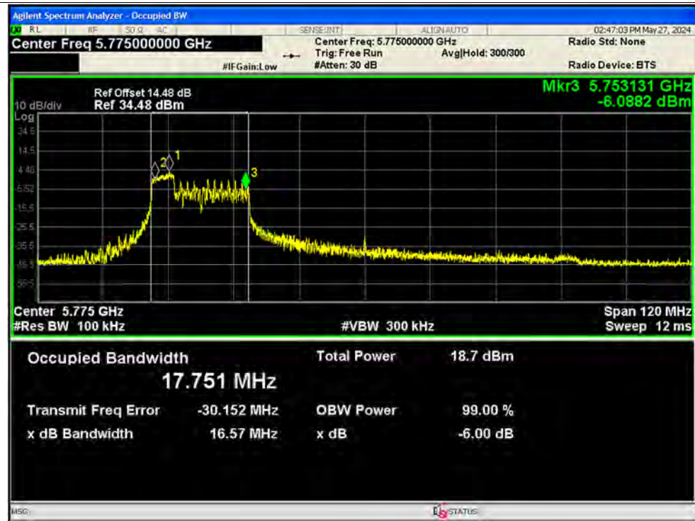
-6dB Bandwidth NVNT ax80 52@37 5775MHz Ant2
