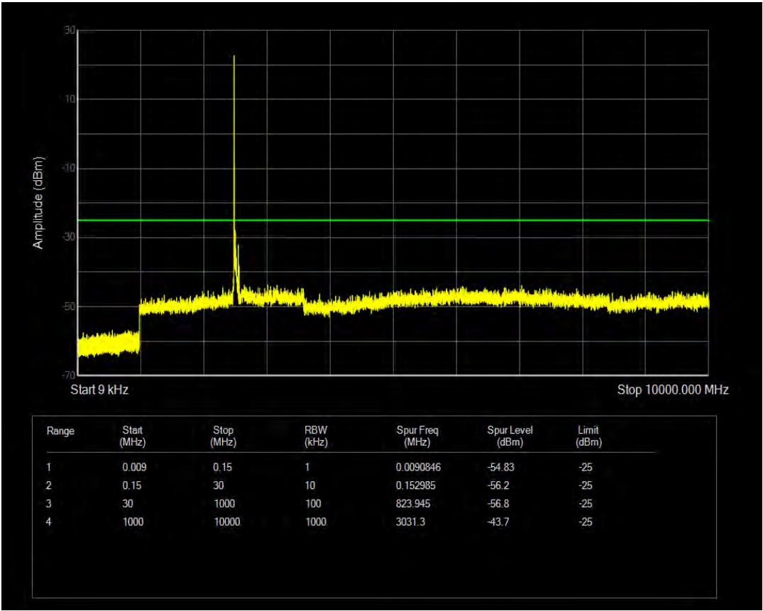
n41 SCS=30kHz CP_QPSK BW=40MHz Channel=503202 RB=1@105
