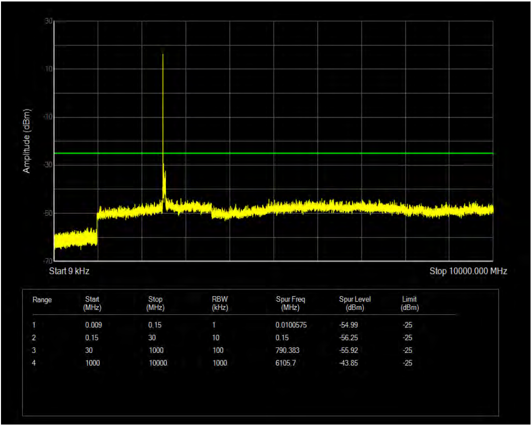
n41 SCS=30kHz CP_QPSK BW=60MHz Channel=505200 RB=1@161
