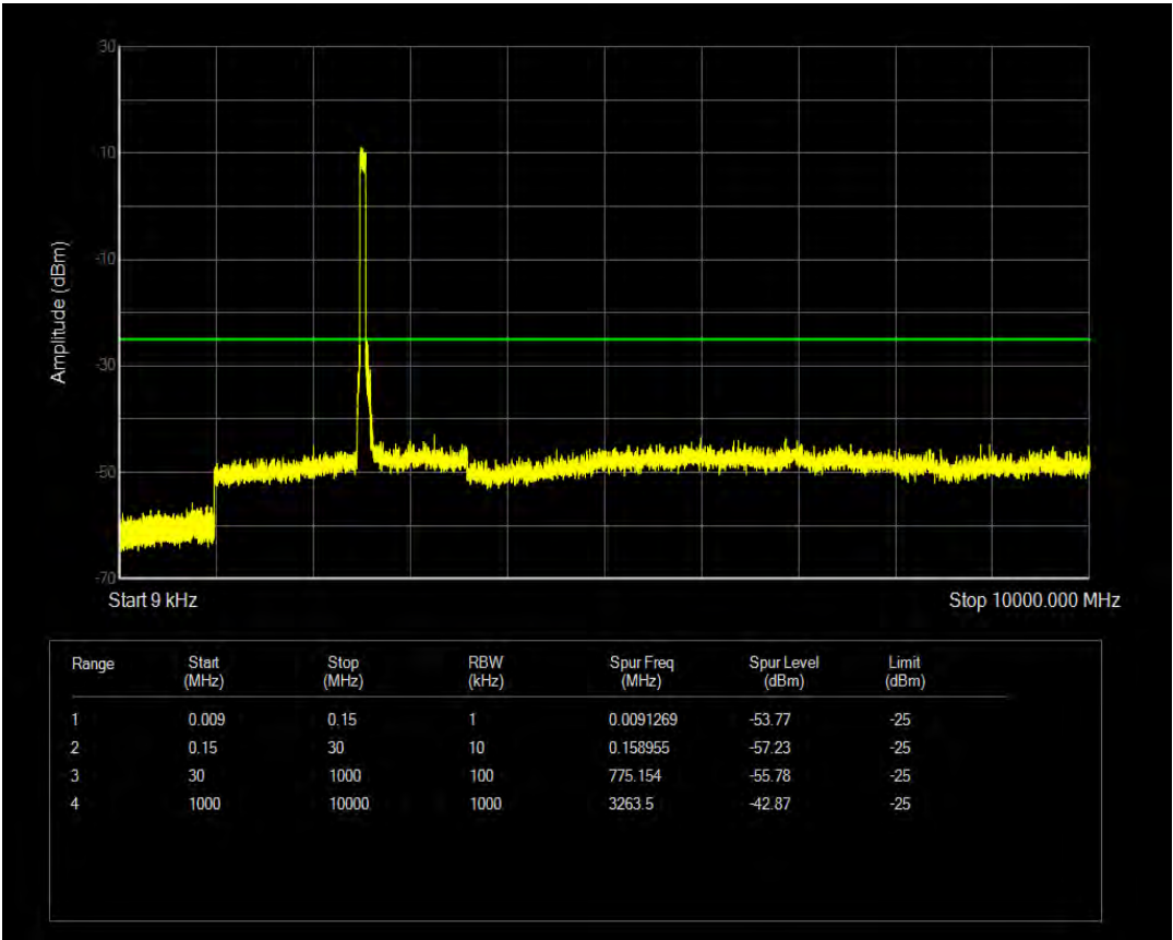
n41 SCS=30kHz CP_QPSK BW=60MHz Channel=505200 RB=1@0
