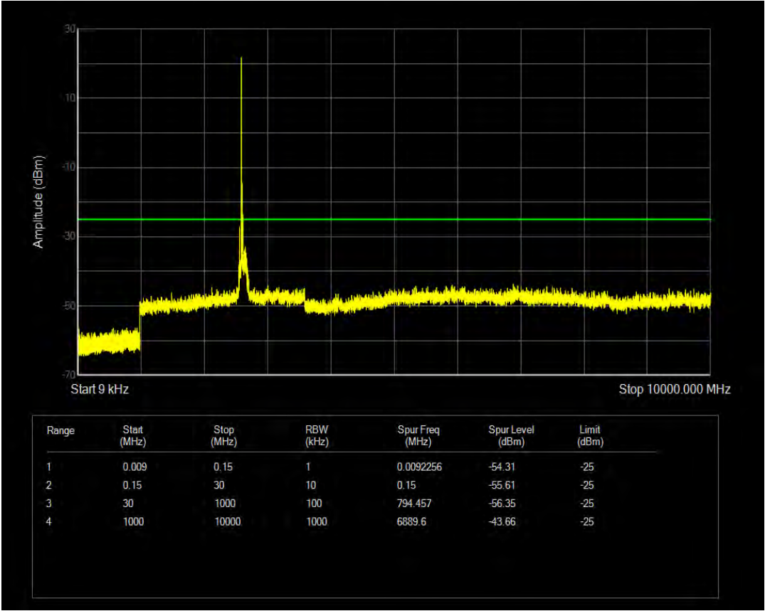
n41 SCS=30kHz CP_QPSK BW=90MHz Channel=528996 RB=1@244
