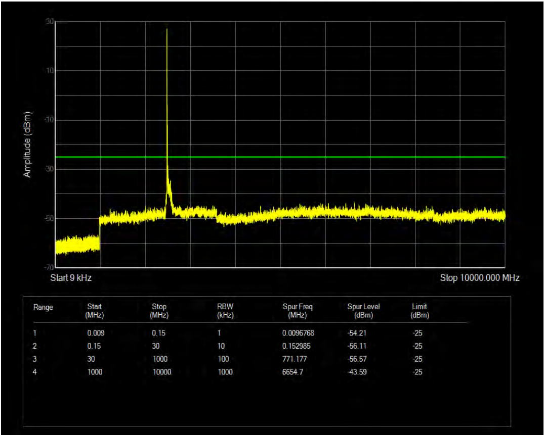
n41 SCS=30kHz CP_QPSK BW=80MHz Channel=507204 RB=1@216
