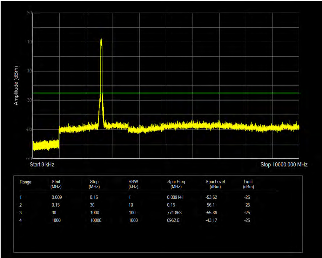
n41 SCS=30kHz CP_QPSK BW=60MHz Channel=518598 RB=1@0
