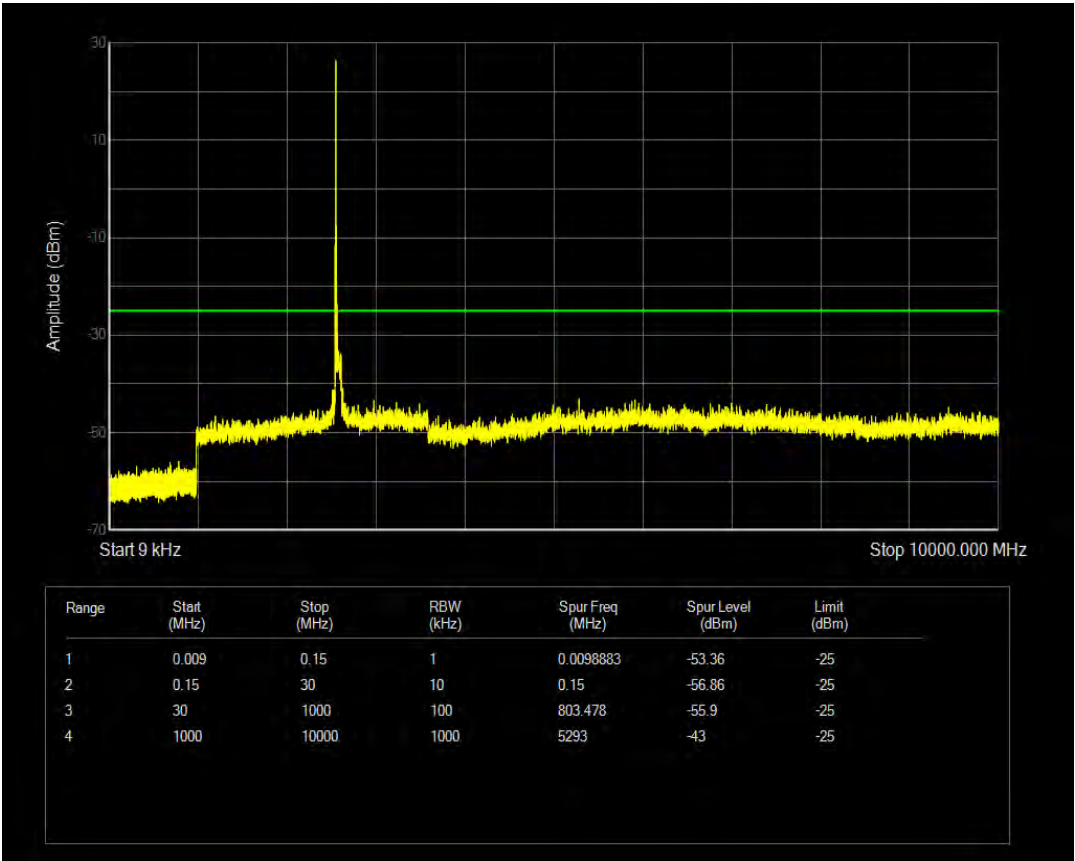
n41 SCS=30kHz CP_QPSK BW=60MHz Channel=518598 RB=1@161
