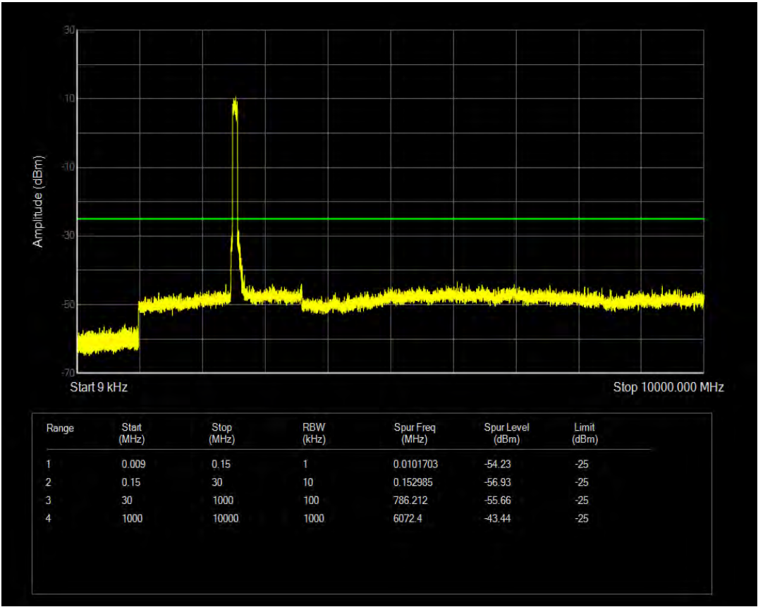
n41 SCS=30kHz CP_QPSK BW=80MHz Channel=507204 RB=1@0
