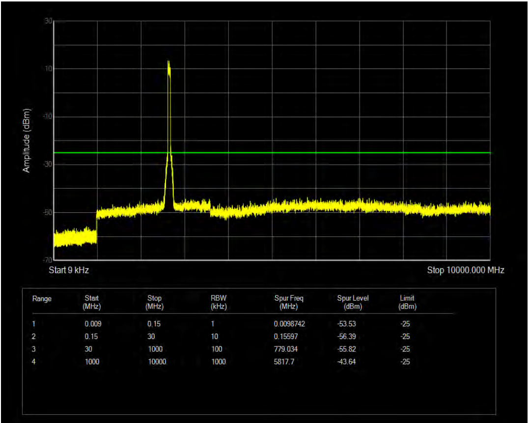
n41 SCS=30kHz CP_QPSK BW=60MHz Channel=531996 RB=1@0
