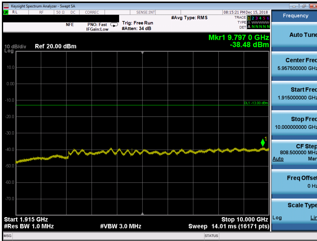
Plot 7-72. Conducted Spurious Plot (Band 25/2 - 20MHz QPSK - RB Size 1, RB Offset 0 - Mid Channel)
