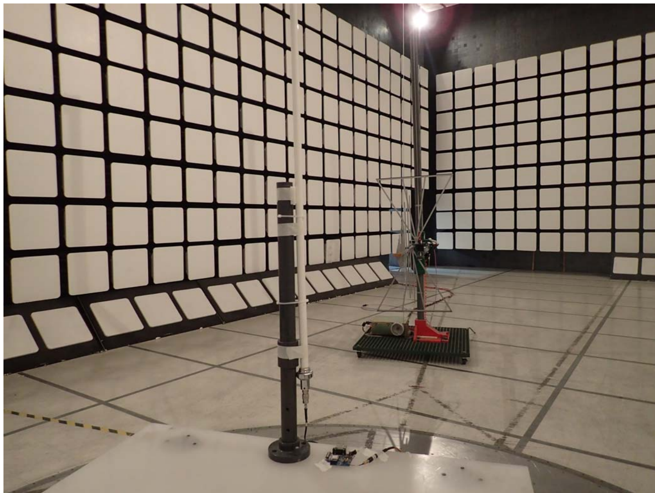
Radiated Emissions @ 3 m, Orthogonal Position 1 EUT with 15 dBi Omni-directional Antenna and 8.04 dB Assembly Cable Loss
