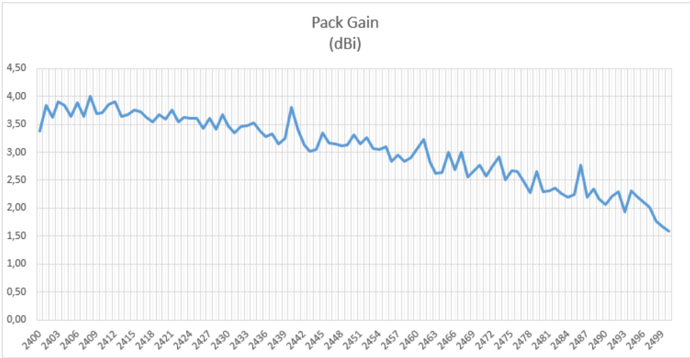
Fig. 3. Peak antenna gain between 2400 MHz and 2500 MHz.
