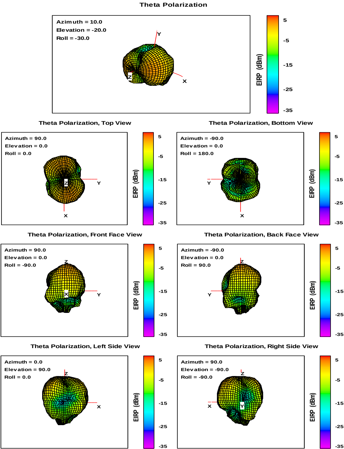
Fig. 11. Theta Polarization EIRP, Free Space, 2480 MHz.
