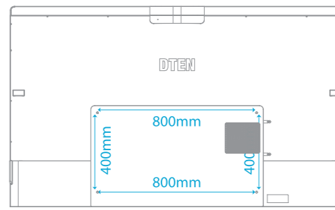
Mounting Hole Pattern: 800mm x 400mm
