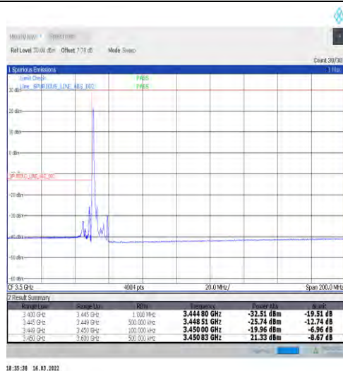
1-N77-3450-3550-30-10-L-4-CP-QPSK-Edge_1RB_Lef t-1@0-Ant1-PASS-see graph
