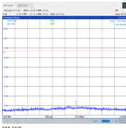
1-N77-3450-3550-30-100-L-1-DFT-PI2BPSK-Inner_1 RB_Left-1@1-30-1000-Ant1--69.24--23-PASS
