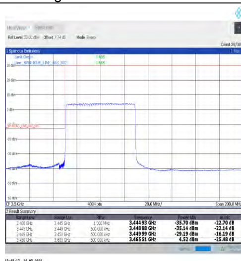
1-N77-3450-3550-30-60-L-3-DFT-PI2BPSK-Outer _Full-162@0-Ant1-PASS-see graph
