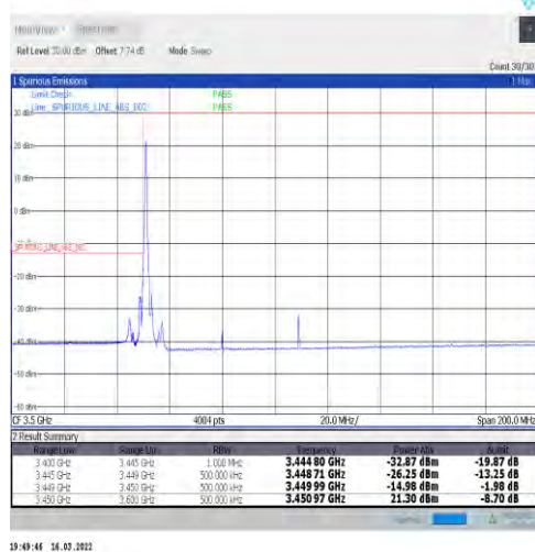
1-N77-3450-3550-30-60-L-4-CP-QPSK-Edge_1RB_Lef t-1@0-Ant1-PASS-see graph
