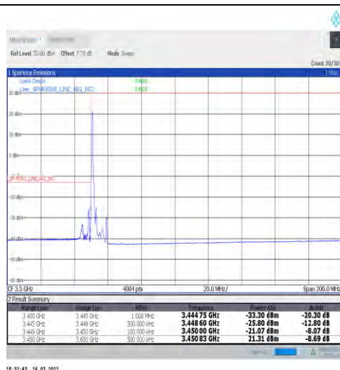
1-N77-3450-3550-30-10-L-1-DFT-PI2BPSK-Edge_1RB _Left-1@0-Ant1-PASS-see graph
