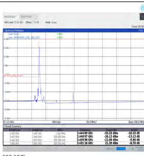
1-N77-3450-3550-30-50-L-1-DFT-PI2BPSK-Edge_1RB _Left-1@0-Ant1-PASS-see graph
