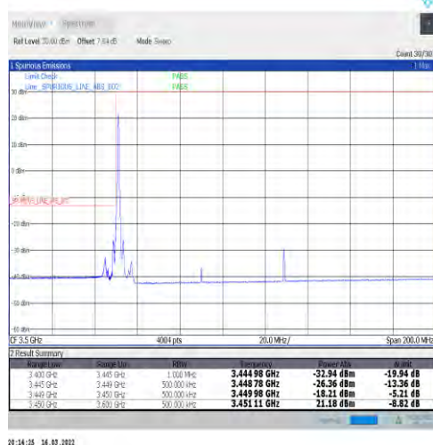
1-N77-3450-3550-30-80-L-4-CP-QPSK-Edge_1RB_Lef t-1@0-Ant1-PASS-see graph
