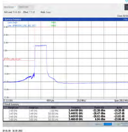
1-N77-3450-3550-30-20-L-6-CP-QPSK-Outer_Full -51@0-Ant1-PASS-see graph
