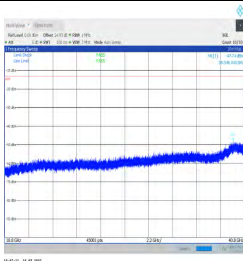
1-N77-3450-3550-30-100-L-1-DFT-PI2BPSK-Inner_1 RB_Left-1@1-18000-40000-Ant1--47.74--13-PASS
