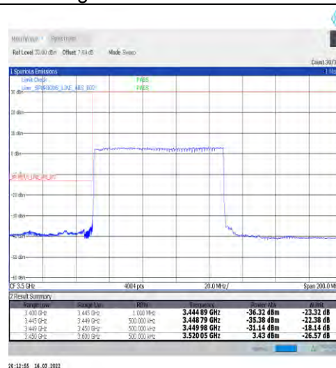
1-N77-3450-3550-30-80-L-3-DFT-PI2BPSK-Outer_Full-216@0-Ant1-PASS-see graph
