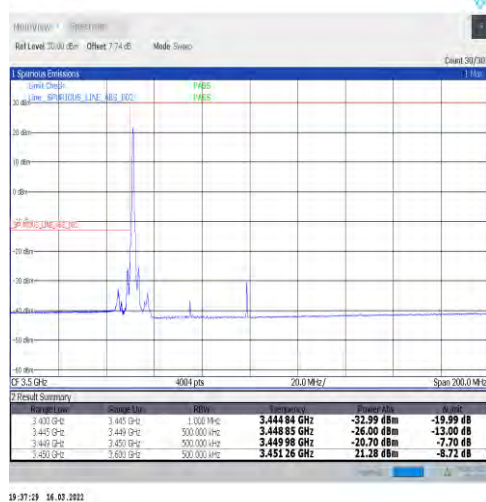
1-N77-3450-3550-30-50-L-4-CP-QPSK-Edge_1RB_Lef t-1@0-Ant1-PASS-see graph
