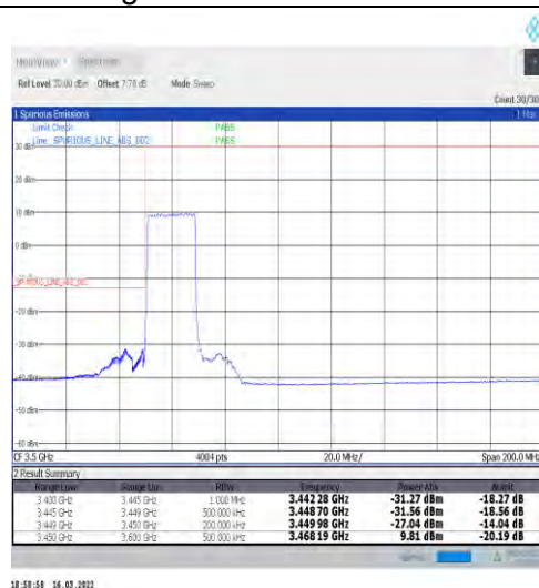
1-N77-3450-3550-30-20-L-3-DFT-PI2BPSK-Outer _Full-50@0-Ant1-PASS-see graph
