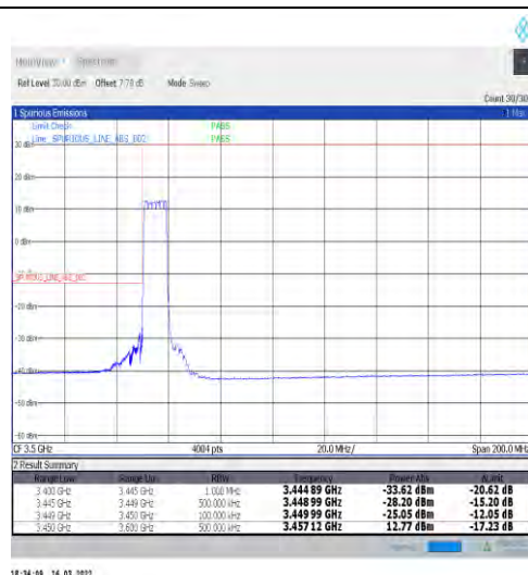
1-N77-3450-3550-30-10-L-3-DFT-PI2BPSK-Outer _Full-24@0-Ant1-PASS-see graph
