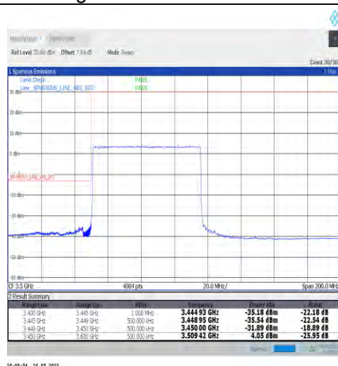
1-N77-3450-3550-30-70-L-3-DFT-PI2BPSK-Outer _Full-180@0-Ant1-PASS-see graph
