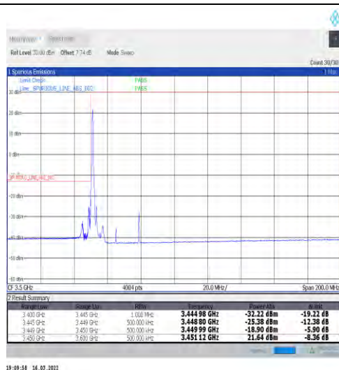
1-N77-3450-3550-30-30-L-1-DFT-PI2BPSK-Edge_1RB_Left-1@0-Ant1-PASS-see graph
