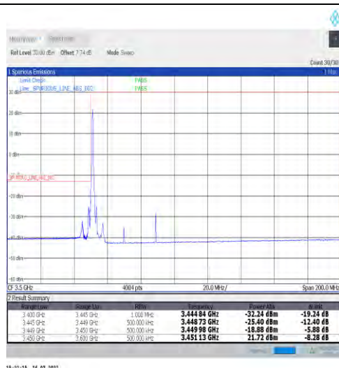
1-N77-3450-3550-30-40-L-1-DFT-PI2BPSK-Edge_1RB _Left-1@0-Ant1-PASS-see graph
