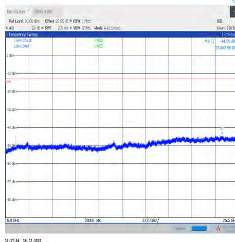
1-N77-3450-3550-30-100-L-1-DFT-PI2BPSK-Inner_1 RB_Left-1@1-6000-26500-Ant1--44.28--13-PASS
