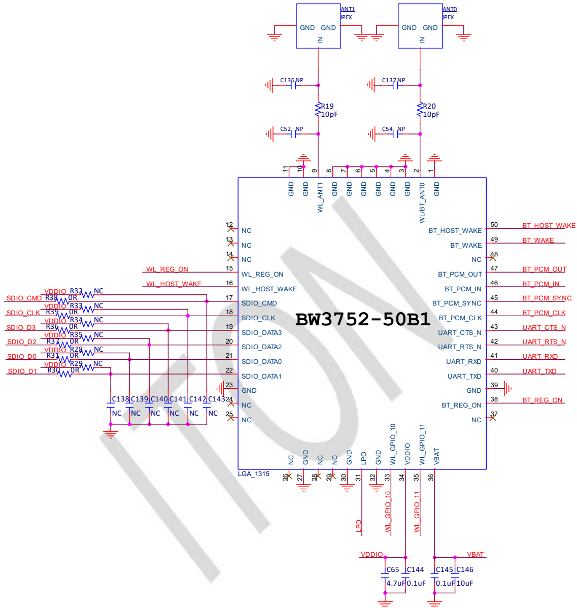
Figure 3. Application Schematic Diagram of BW3752-50B1
