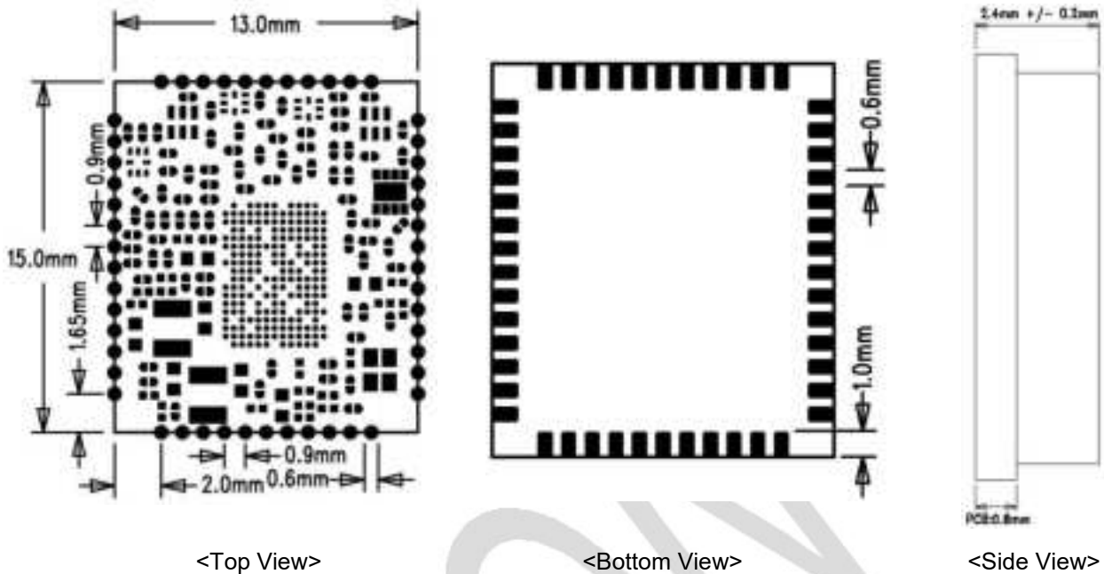
Figure 4. Mechanical Size of BW3752-50B1
