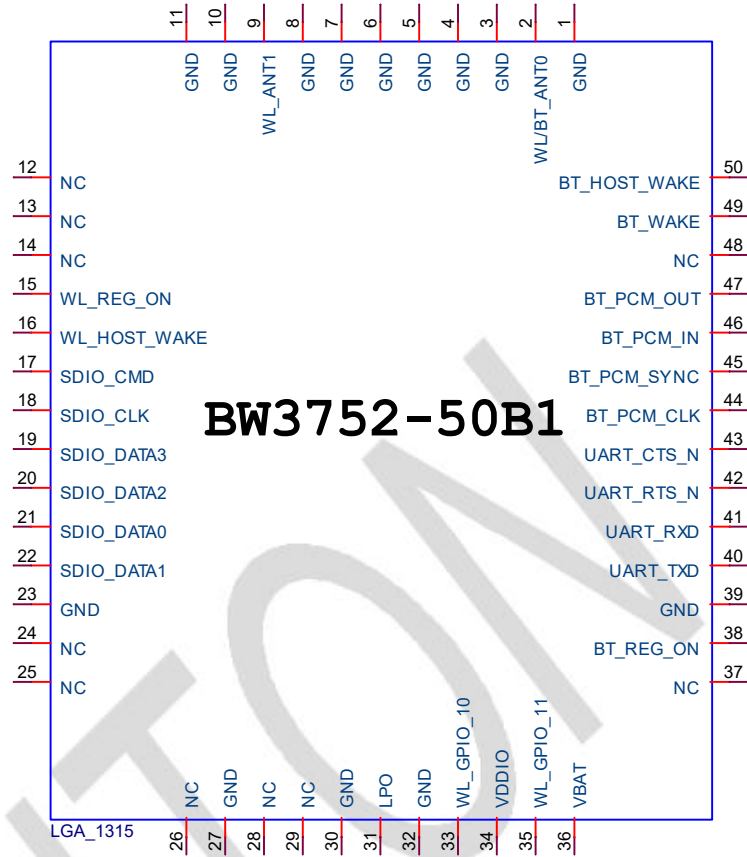
Figure 2.Pin Diagram of BW3752-50B1
