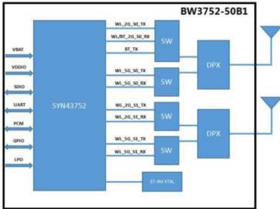
Figure 1. Block Diagram of BW3752-50B1
