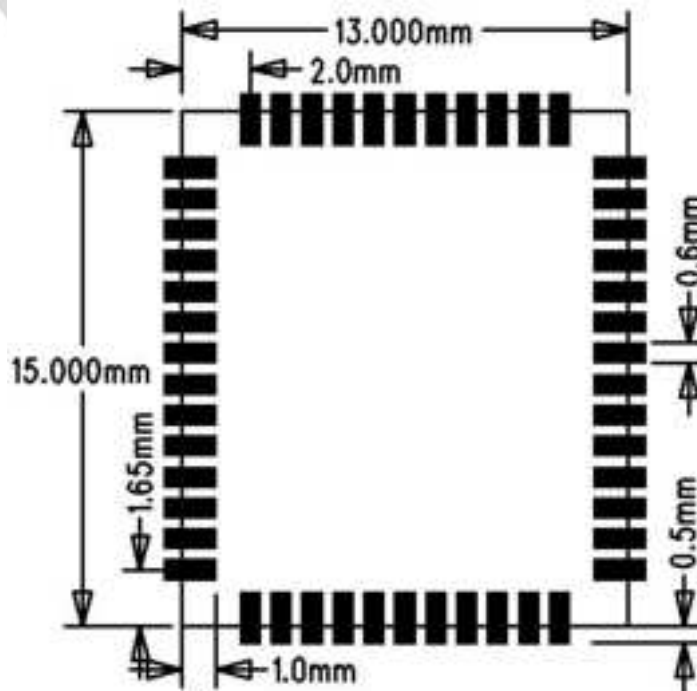
Figure 5. Recommended Land Pattern of BW3752-50B1
