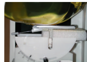
Fig. 20 Head SAR Test Setup
