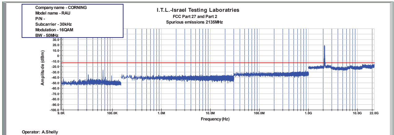
Figure 855: Spurious Emissions at Antenna Terminal 16QAM 50MHz B.W.; 2135.0MHz, 30kHz
