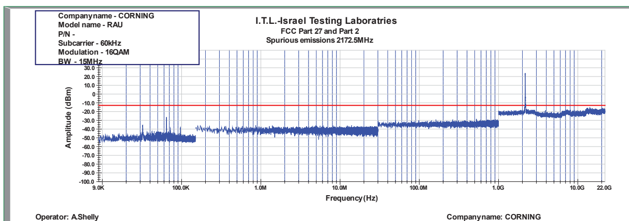
Figure 824: Spurious Emissions at Antenna Terminal 16QAM 15MHz B.W.; 2172.5MHz, 60kHz
