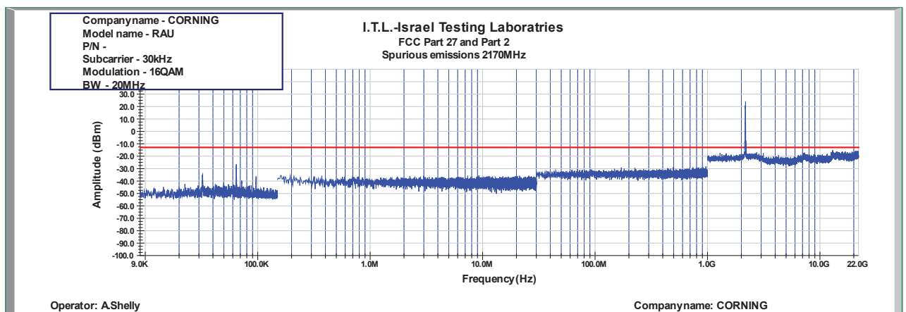
Figure 830: Spurious Emissions at Antenna Terminal 16QAM 20MHz B.W.; 2170.0MHz, 30kHz
