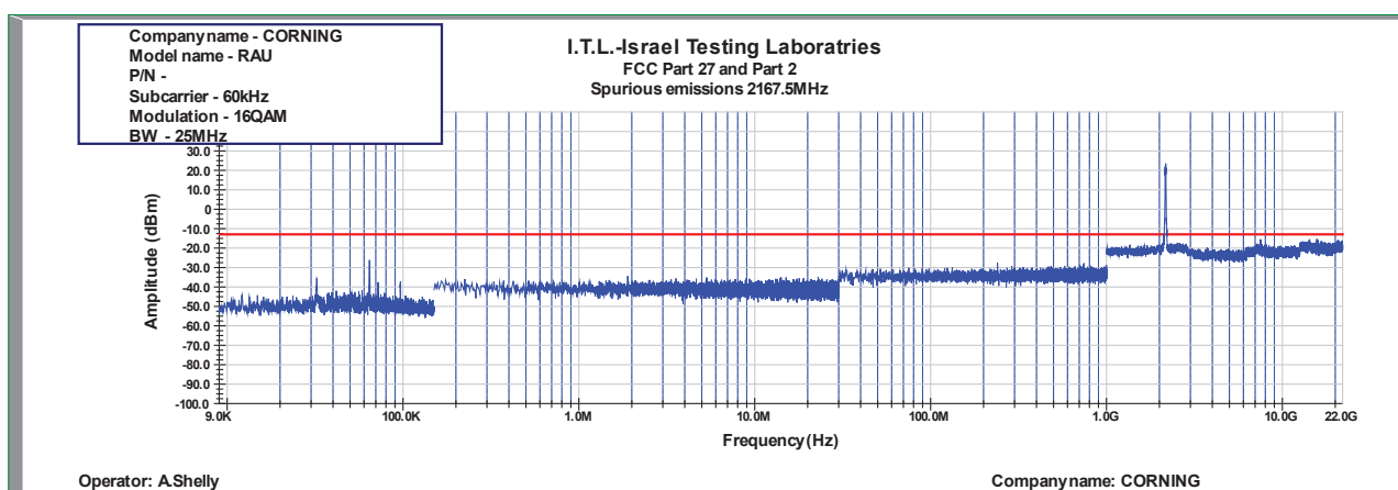
Figure 842: Spurious Emissions at Antenna Terminal 16QAM 25MHz B.W.; 2167.5MHz, 60kHz
