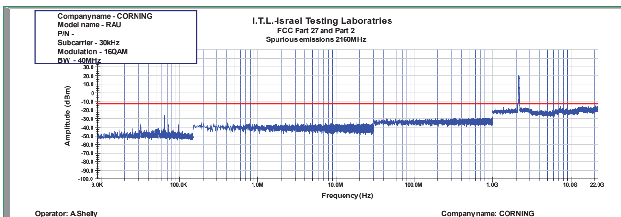
Figure 848: Spurious Emissions at Antenna Terminal 16QAM 40MHz B.W.; 2160.0MHz, 30kHz
