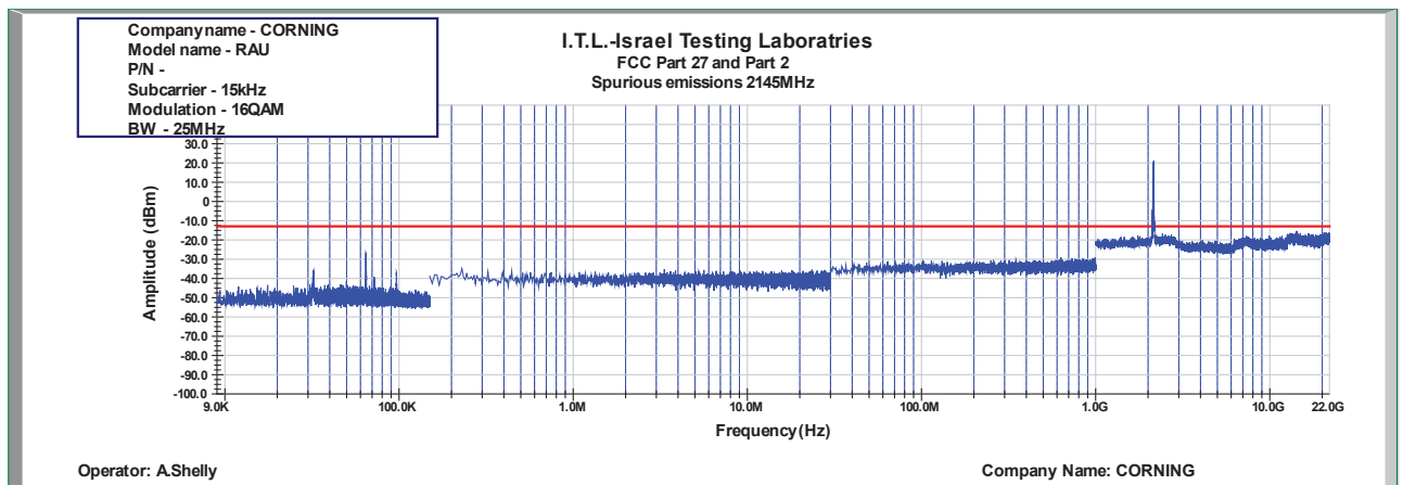
Figure 835: Spurious Emissions at Antenna Terminal 16QAM 25MHz B.W.; 2145.0MHz, 15kHz
