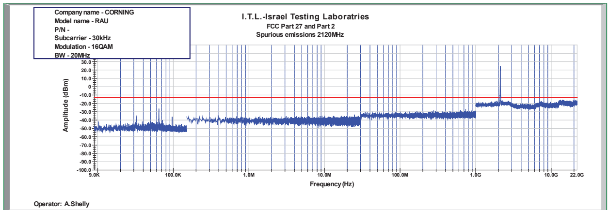
Figure 828: Spurious Emissions at Antenna Terminal 16QAM 20MHz B.W.; 2120.0MHz, 30kHz
