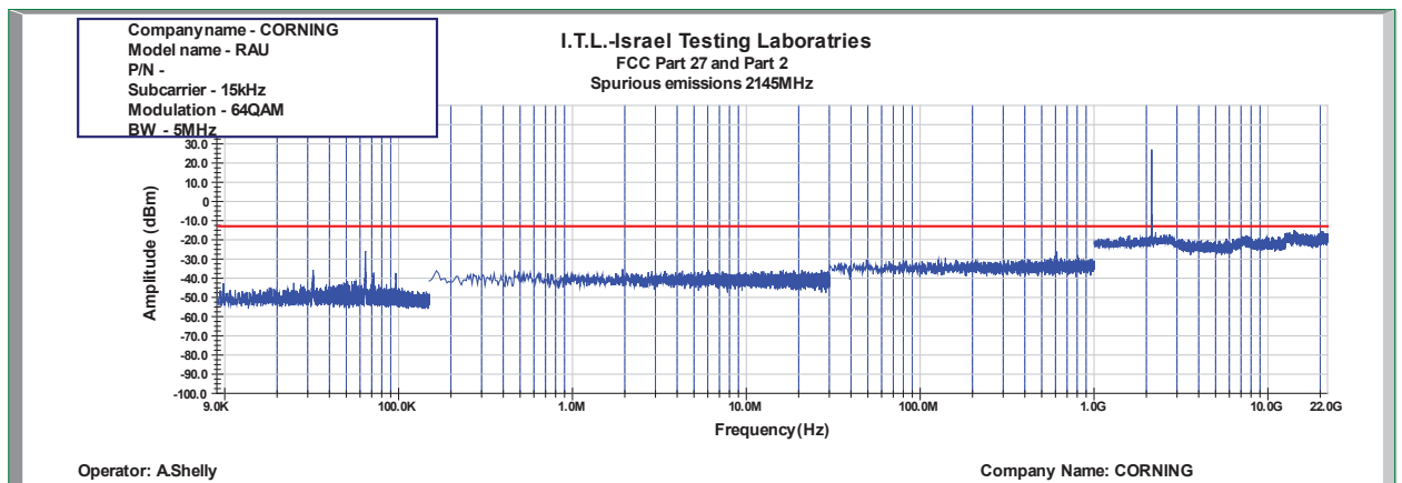
Figure 868: Spurious Emissions at Antenna Terminal 64QAM 5MHz B.W.; 2145.0MHz, 15kHz
