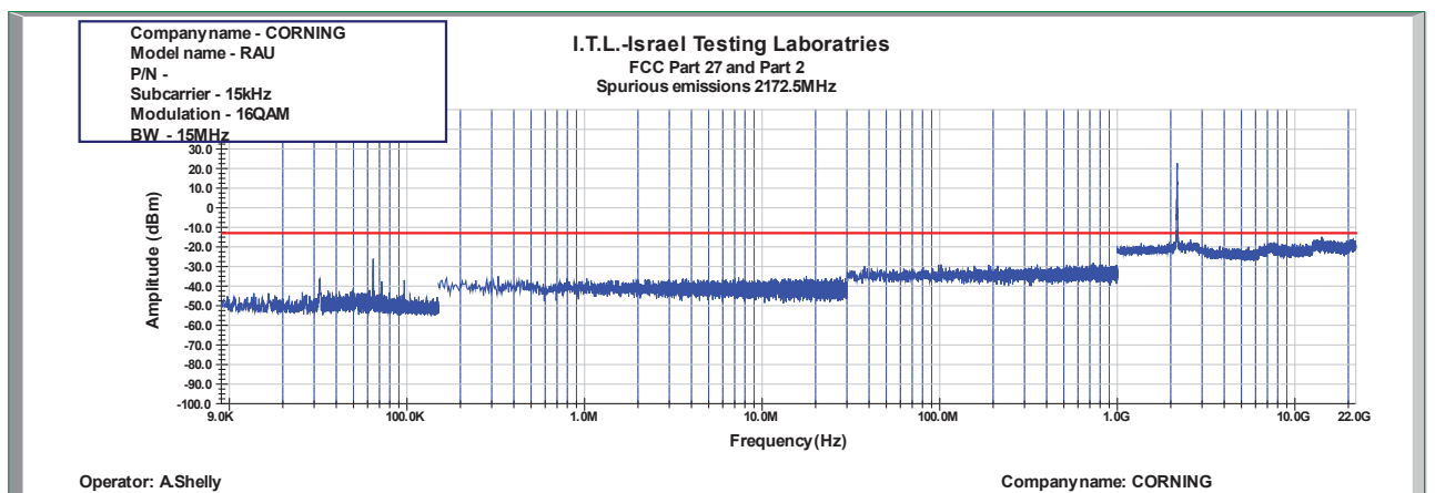
Figure 818: Spurious Emissions at Antenna Terminal 16QAM 15MHz B.W.; 2172.5MHz, 15kHz
