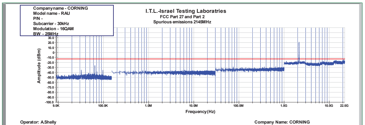
Figure 838: Spurious Emissions at Antenna Terminal 16QAM 25MHz B.W.; 2145.0MHz, 30kHz
