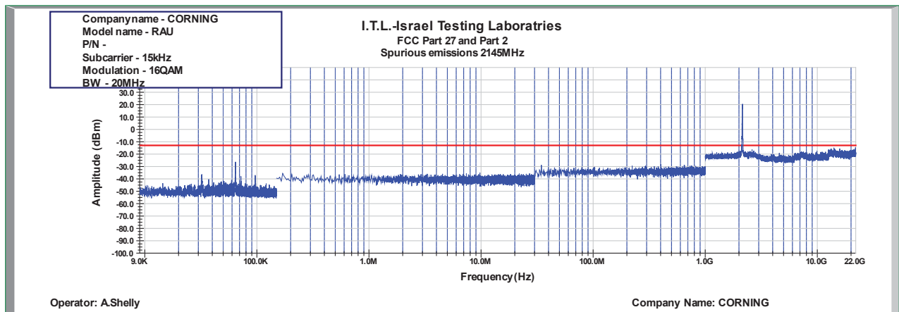
Figure 826: Spurious Emissions at Antenna Terminal 16QAM 20MHz B.W.; 2145.0MHz, 15kHz
