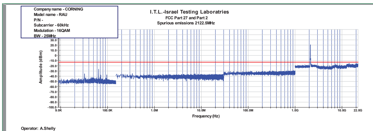
Figure 840: Spurious Emissions at Antenna Terminal 16QAM 25MHz B.W.; 2122.5MHz, 60kHz
