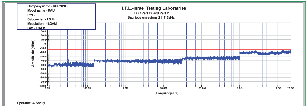
Figure 816: Spurious Emissions at Antenna Terminal 16QAM 15MHz B.W.; 2117.5MHz, 15kHz
