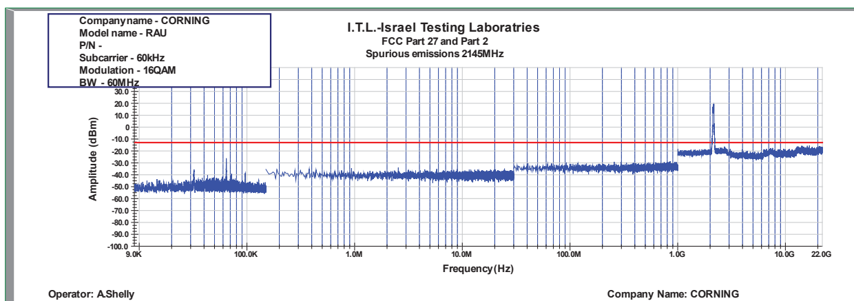
Figure 865: Spurious Emissions at Antenna Terminal 16QAM 60MHz B.W.; 2145.0MHz, 60kHz
