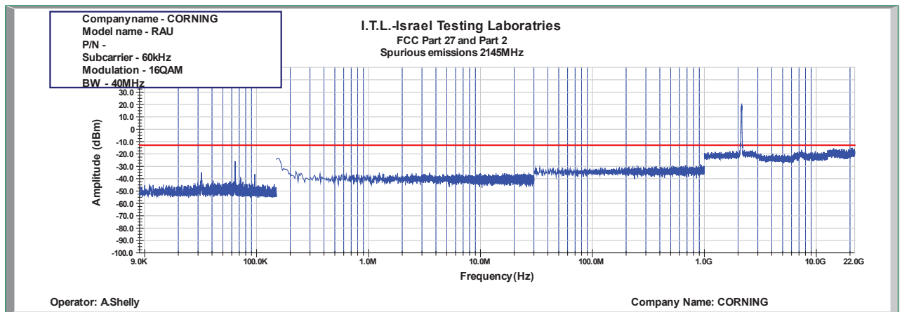
Figure 850: Spurious Emissions at Antenna Terminal 16QAM 40MHz B.W.; 2145.0MHz, 60kHz
