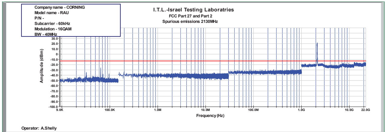
Figure 849: Spurious Emissions at Antenna Terminal 16QAM 40MHz B.W.; 2130.0MHz, 60kHz
