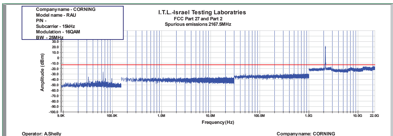
Figure 836: Spurious Emissions at Antenna Terminal 16QAM 25MHz B.W.; 2167.5MHz, 15kHz
