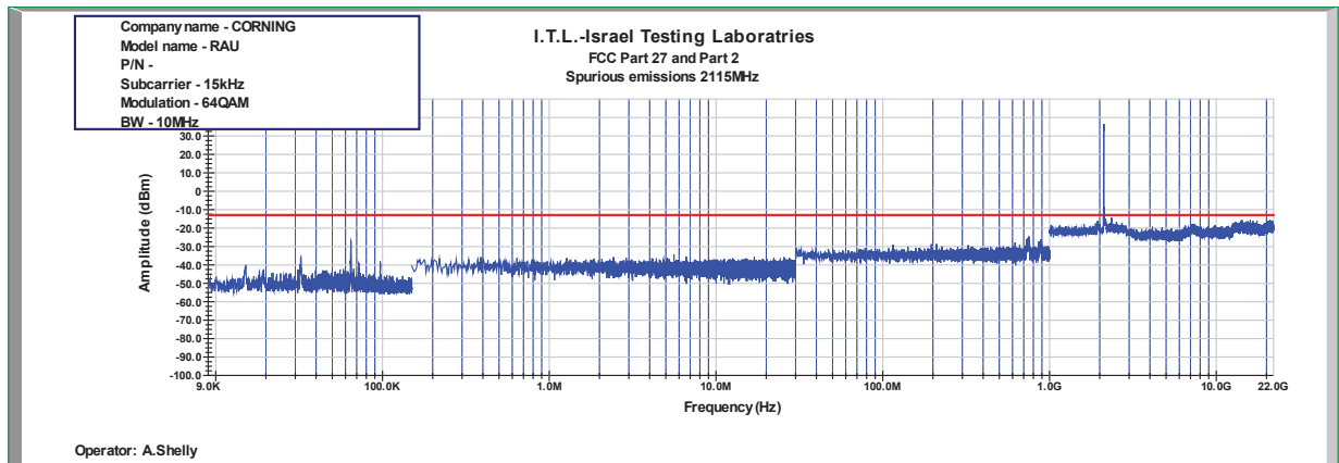
Figure 873: Spurious Emissions at Antenna Terminal 64QAM 10MHz B.W.; 2115.0MHz, 15kHz
