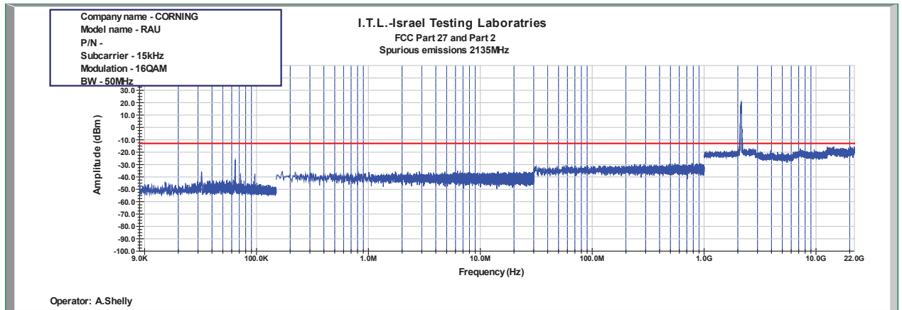
Figure 852: Spurious Emissions at Antenna Terminal 16QAM 50MHz B.W.; 2135.0MHz, 15kHz
