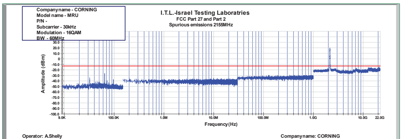
Figure 863: Spurious Emissions at Antenna Terminal 16QAM 60MHz B.W.; 2155.0MHz, 30kHz
