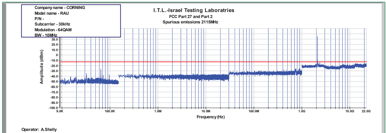
Figure 876: Spurious Emissions at Antenna Terminal 64QAM 10MHz B.W.; 2115.0MHz, 30kHz
