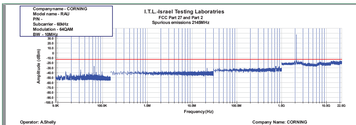
Figure 880: Spurious Emissions at Antenna Terminal 64QAM 10MHz B.W.; 2145.0MHz, 60kHz
