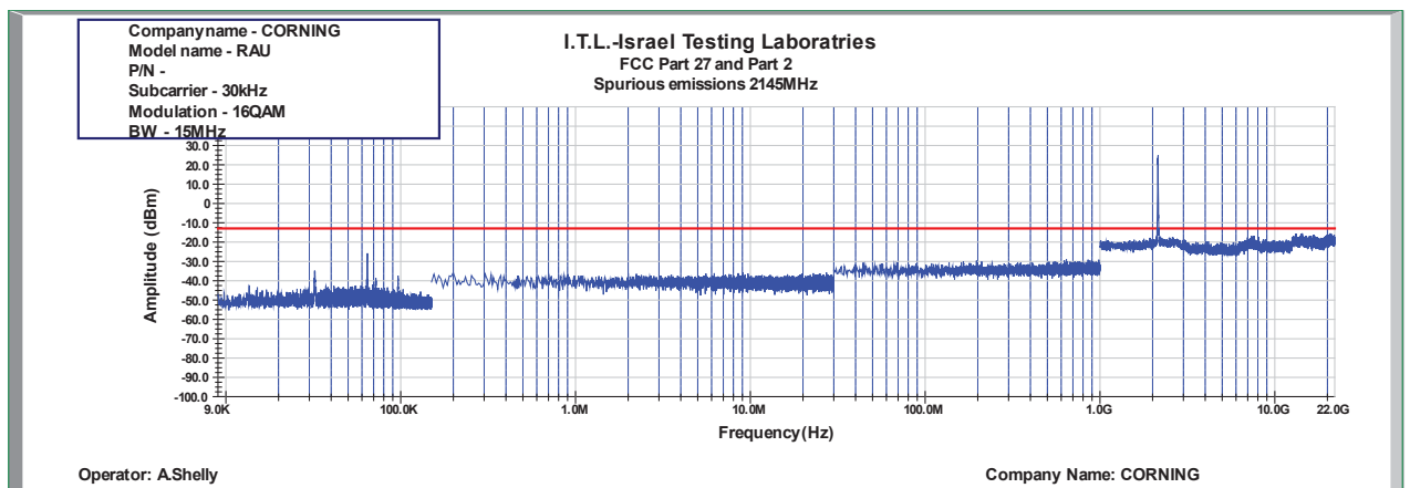
Figure 820: Spurious Emissions at Antenna Terminal 16QAM 15MHz B.W.; 2145.0MHz, 30kHz
