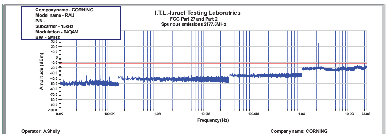
Figure 869: Spurious Emissions at Antenna Terminal 64QAM 5MHz B.W.; 2177.5MHz, 15kHz
