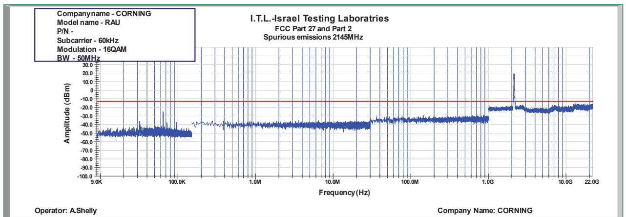
Figure 859: Spurious Emissions at Antenna Terminal 16QAM 50MHz B.W.; 2145.0MHz, 60kHz
