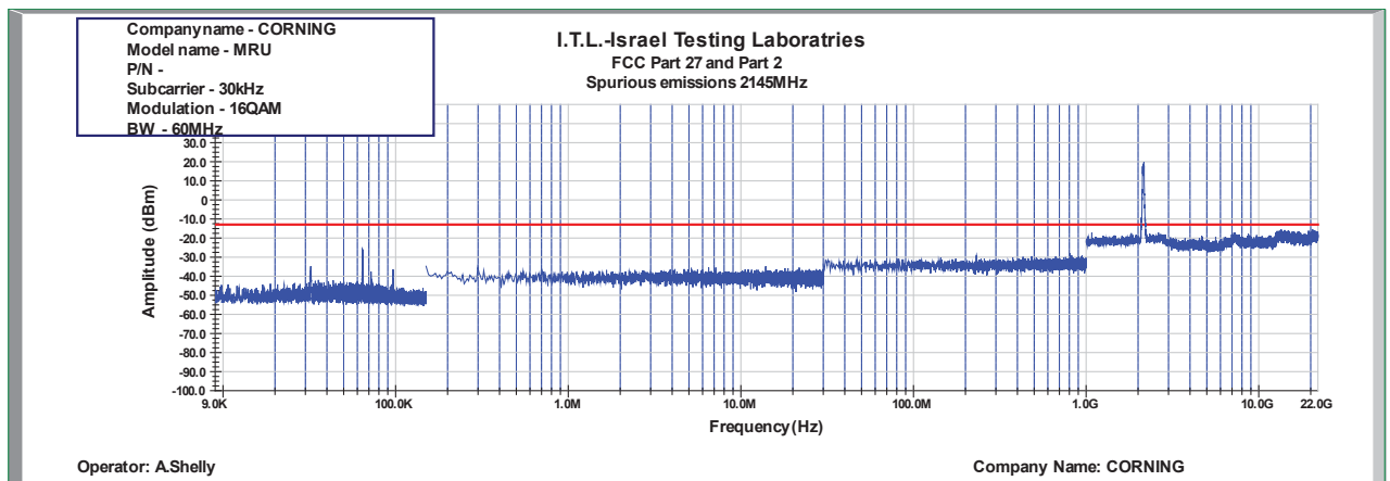
Figure 862: Spurious Emissions at Antenna Terminal 16QAM 60MHz B.W.; 2145.0MHz, 30kHz
