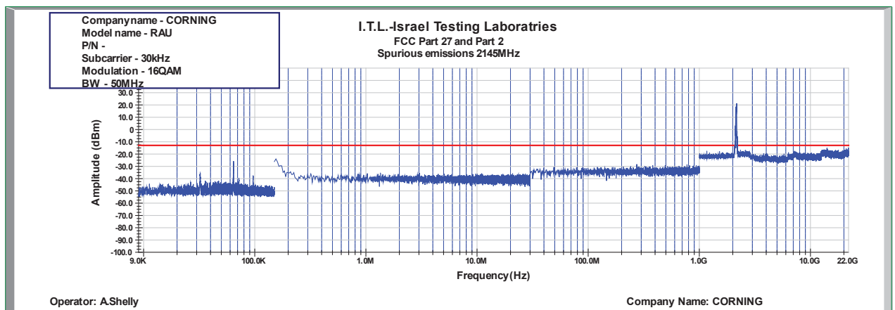
Figure 856: Spurious Emissions at Antenna Terminal 16QAM 50MHz B.W.; 2145.0MHz, 30kHz
