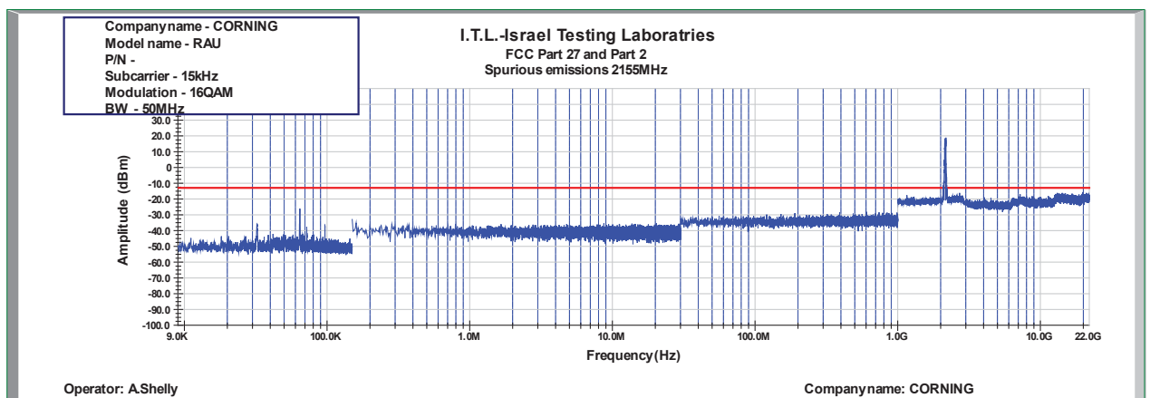
Figure 854: Spurious Emissions at Antenna Terminal 16QAM 50MHz B.W.; 2155.0MHz, 15kHz
