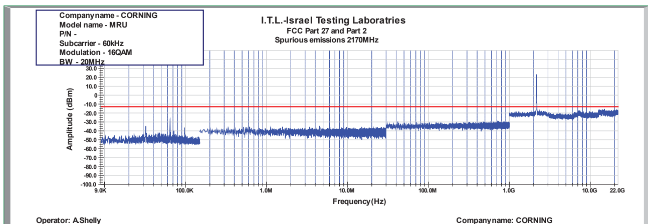
Figure 833: Spurious Emissions at Antenna Terminal 16QAM 20MHz B.W.; 2170.0MHz, 60kHz
