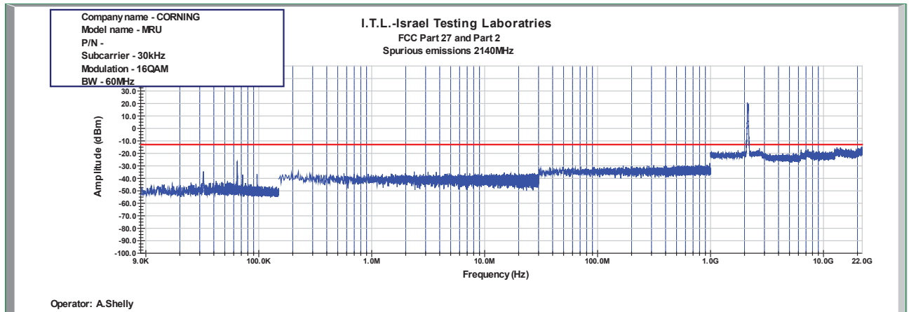
Figure 861: Spurious Emissions at Antenna Terminal 16QAM 60MHz B.W.; 2140.0MHz, 30kHz
