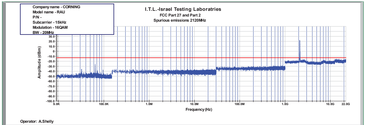
Figure 825: Spurious Emissions at Antenna Terminal 16QAM 20MHz B.W.; 2120.0MHz, 15kHz
