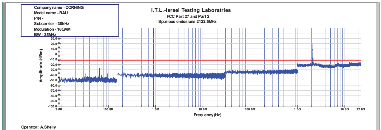
Figure 837: Spurious Emissions at Antenna Terminal 16QAM 25MHz B.W.; 2122.5MHz, 30kHz
