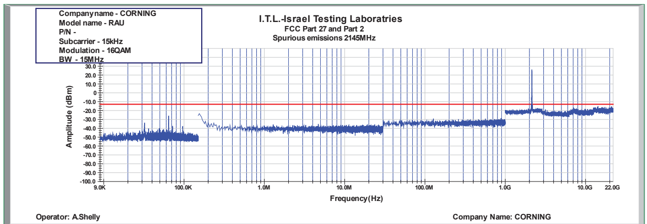
Figure 817: Spurious Emissions at Antenna Terminal 16QAM 15MHz B.W.; 2145.0MHz, 15kHz
