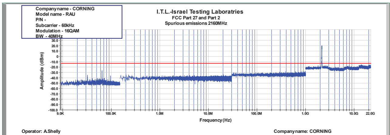
Figure 851: Spurious Emissions at Antenna Terminal 16QAM 40MHz B.W.; 2160.0MHz, 60kHz
