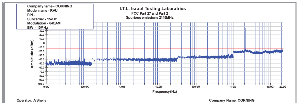
Figure 874: Spurious Emissions at Antenna Terminal 64QAM 10MHz B.W.; 2145.0MHz, 15kHz
