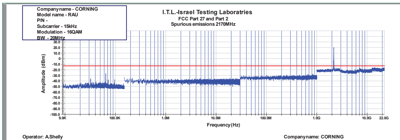
Figure 827: Spurious Emissions at Antenna Terminal 16QAM 20MHz B.W.; 2170.0MHz, 15kHz
