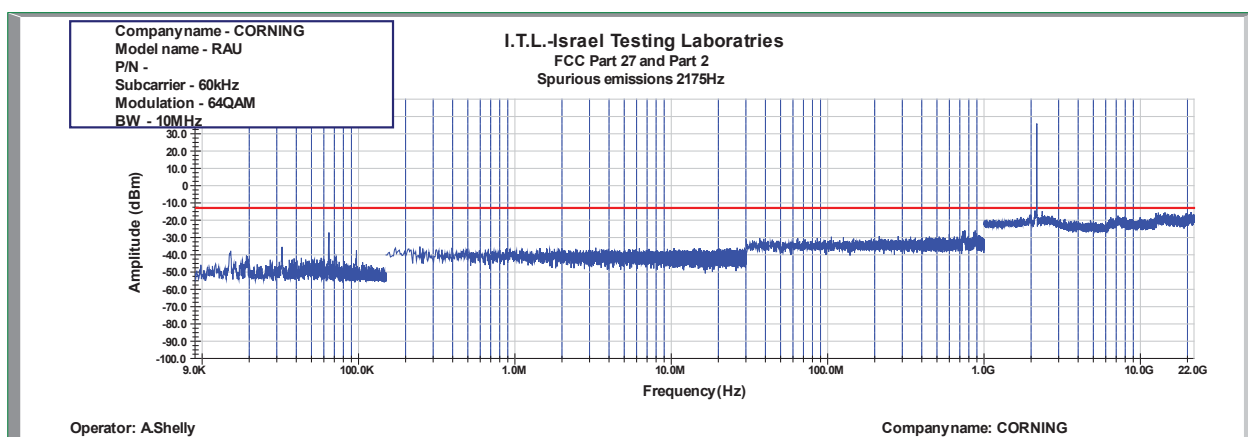
Figure 881: Spurious Emissions at Antenna Terminal 64QAM 10MHz B.W.; 2175.0MHz, 60kHz
