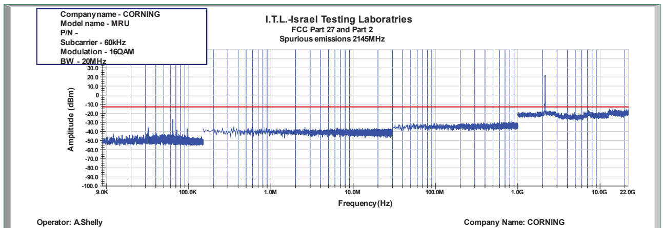
Figure 832: Spurious Emissions at Antenna Terminal 16QAM 20MHz B.W.; 2145.0MHz, 60kHz
