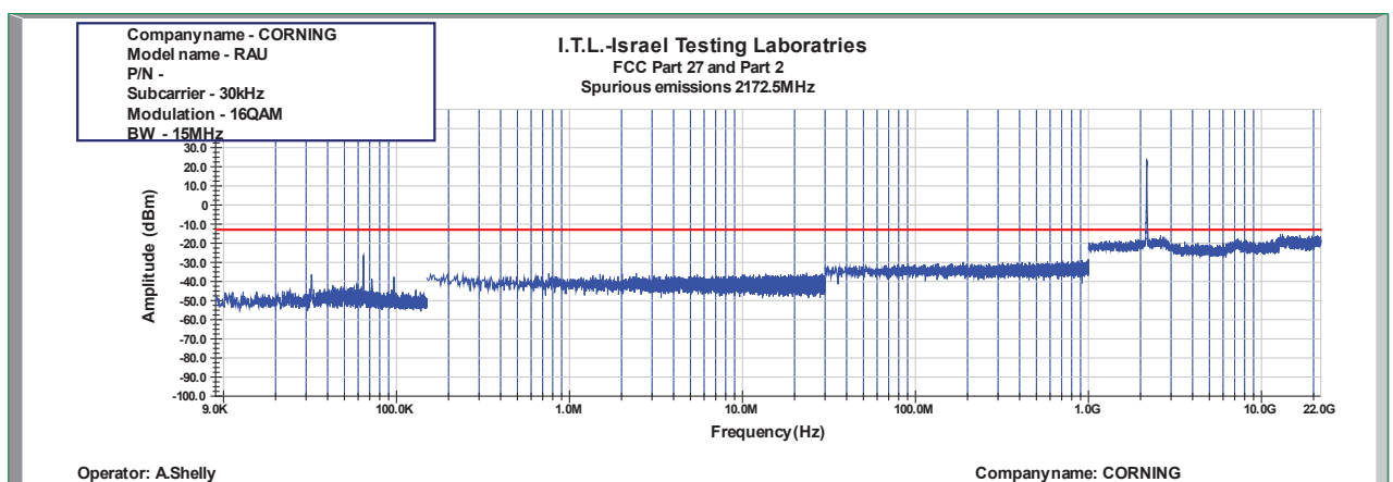
Figure 821: Spurious Emissions at Antenna Terminal 16QAM 15MHz B.W.; 2172.5MHz, 30kHz
