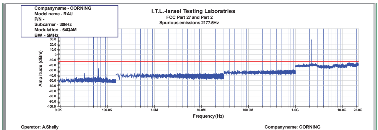
Figure 872: Spurious Emissions at Antenna Terminal 64QAM 5MHz B.W.; 2177.5MHz, 30kHz
