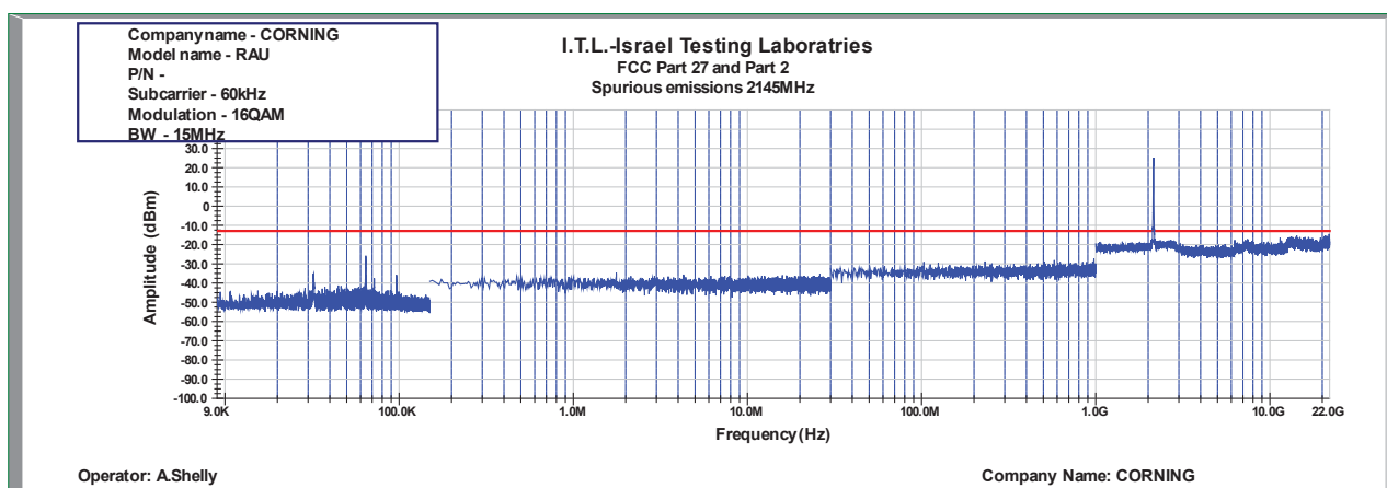
Figure 823: Spurious Emissions at Antenna Terminal 16QAM 15MHz B.W.; 2145.0MHz, 60kHz
