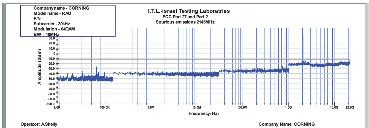
Figure 877: Spurious Emissions at Antenna Terminal 64QAM 10MHz B.W.; 2145.0MHz, 30kHz
