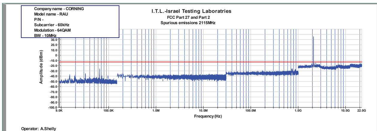
Figure 879: Spurious Emissions at Antenna Terminal 64QAM 10MHz B.W.; 2115.0MHz, 60kHz
