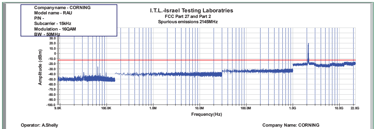
Figure 853: Spurious Emissions at Antenna Terminal 16QAM 50MHz B.W.; 2145.0MHz, 15kHz
