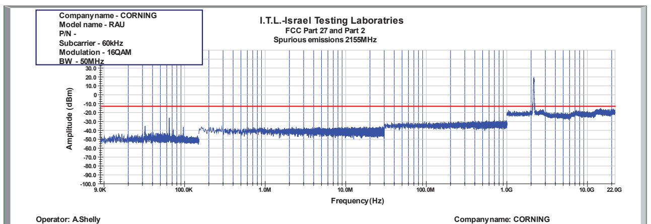
Figure 860: Spurious Emissions at Antenna Terminal 16QAM 50MHz B.W.; 2155.0MHz, 60kHz
