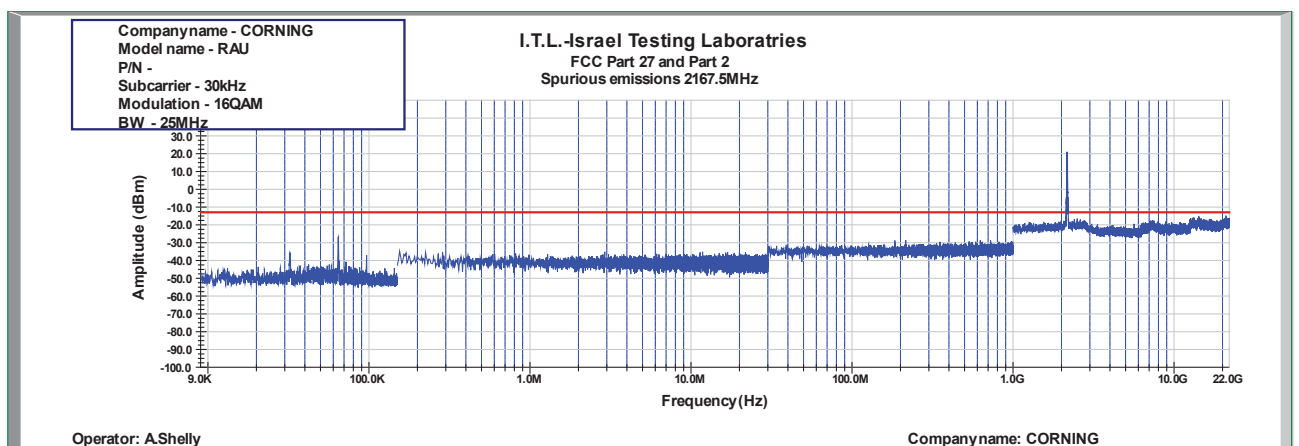
Figure 839: Spurious Emissions at Antenna Terminal 16QAM 25MHz B.W.; 2167.5MHz, 30kHz
