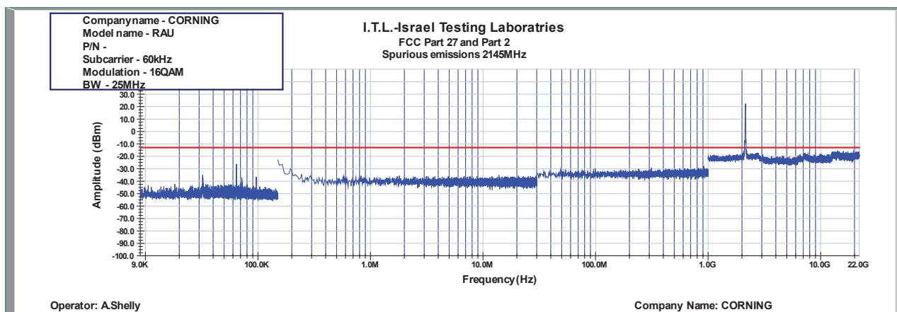
Figure 841: Spurious Emissions at Antenna Terminal 16QAM 25MHz B.W.; 2145.0MHz, 60kHz
