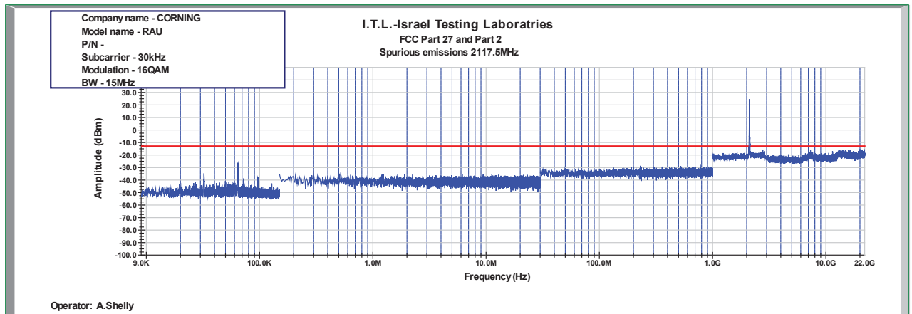
Figure 819: Spurious Emissions at Antenna Terminal 16QAM 15MHz B.W.; 2117.5MHz, 30kHz
