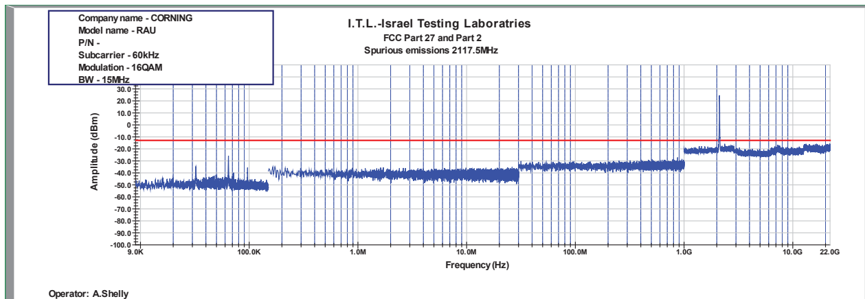
Figure 822: Spurious Emissions at Antenna Terminal 16QAM 15MHz B.W.; 2117.5MHz, 60kHz
