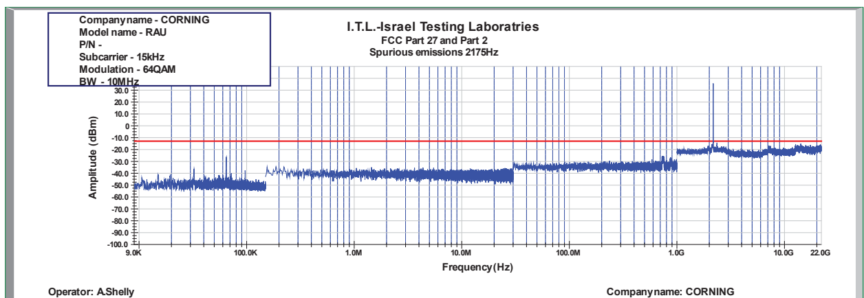
Figure 875: Spurious Emissions at Antenna Terminal 64QAM 10MHz B.W.; 2175.0MHz, 15kHz
