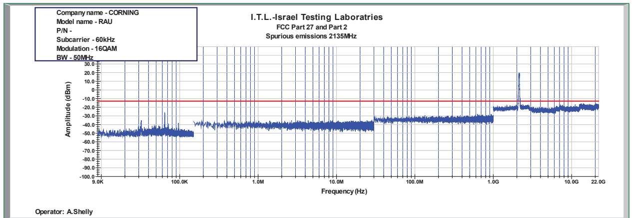
Figure 858: Spurious Emissions at Antenna Terminal 16QAM 50MHz B.W.; 2135.0MHz, 60kHz
