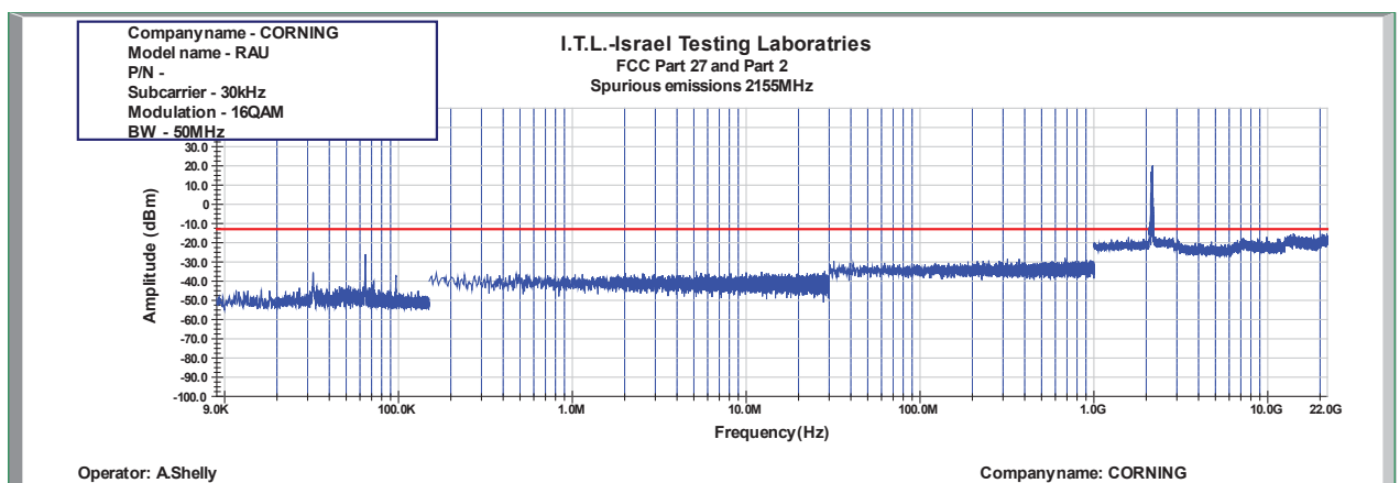
Figure 857: Spurious Emissions at Antenna Terminal 16QAM 50MHz B.W.; 2155.0MHz, 30kHz
