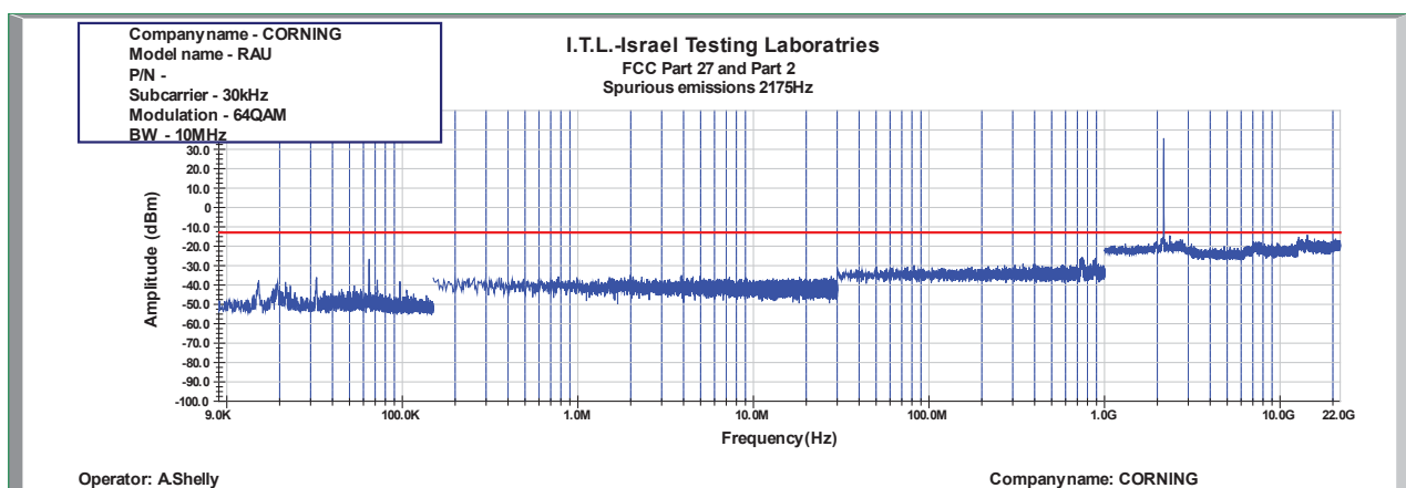
Figure 878: Spurious Emissions at Antenna Terminal 64QAM 10MHz B.W.; 2175.0MHz, 30kHz
