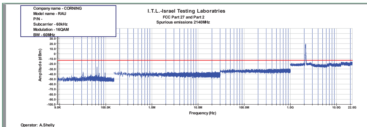
Figure 864: Spurious Emissions at Antenna Terminal 16QAM 60MHz B.W.; 2140.0MHz, 60kHz
