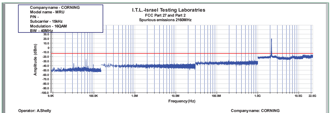
Figure 845: Spurious Emissions at Antenna Terminal 16QAM 40MHz B.W.; 2160.0MHz, 15kHz
