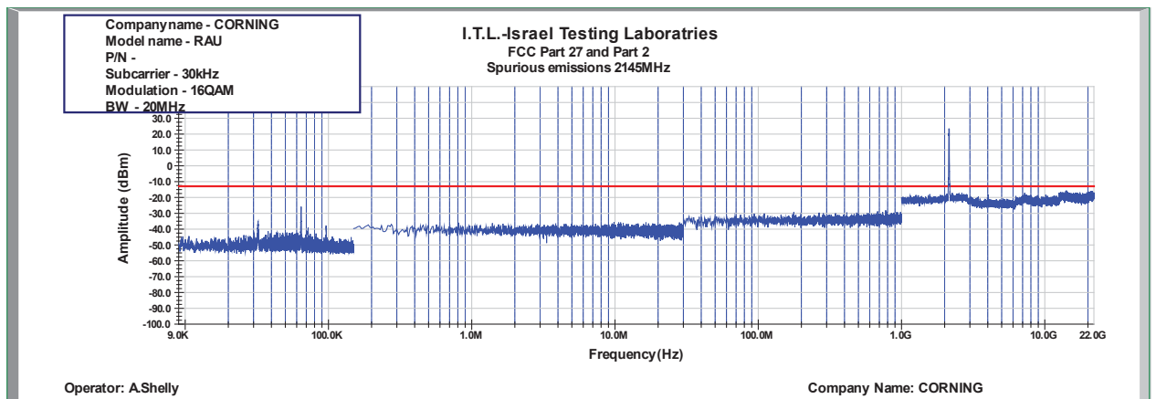
Figure 829: Spurious Emissions at Antenna Terminal 16QAM 20MHz B.W.; 2145.0MHz, 30kHz
