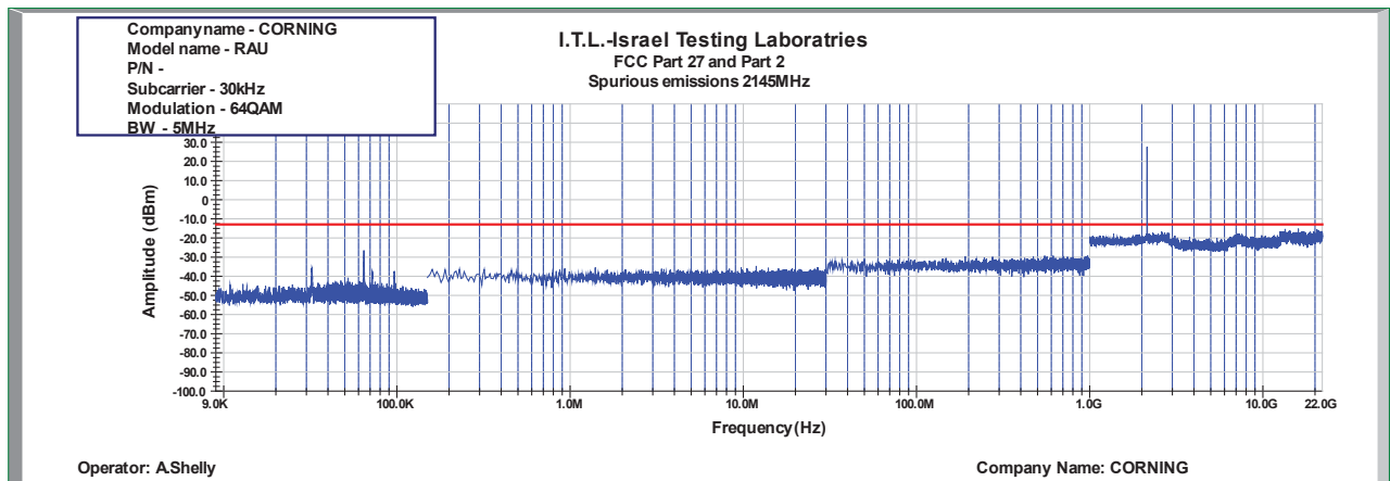
Figure 871: Spurious Emissions at Antenna Terminal 64QAM 5MHz B.W.; 2145.0MHz, 30kHz
