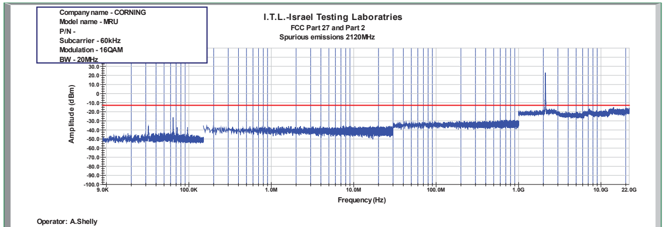
Figure 831: Spurious Emissions at Antenna Terminal 16QAM 20MHz B.W.; 2120.0MHz, 60kHz
