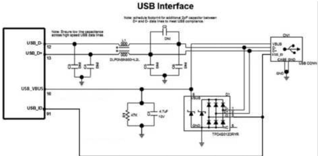
Figure 4-3: USB Interface
