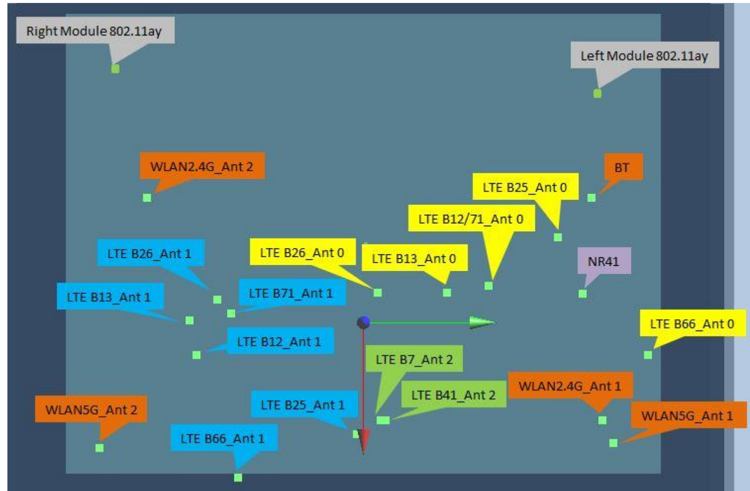
Each transmitter SAR and PD peak location for Front exposure position
