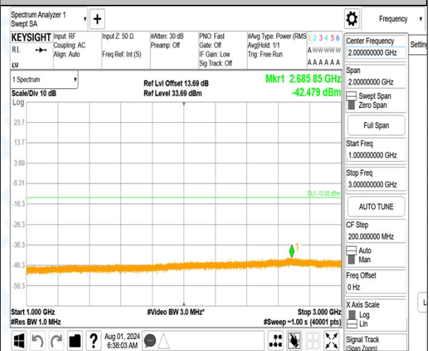
Band12_10MHz_QPSK_23130_1RB#0_1000~3000_1000~3000
