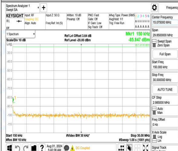
Band12_5MHz_16QAM_23155_1RB#0_0.15~30_0.15~30
