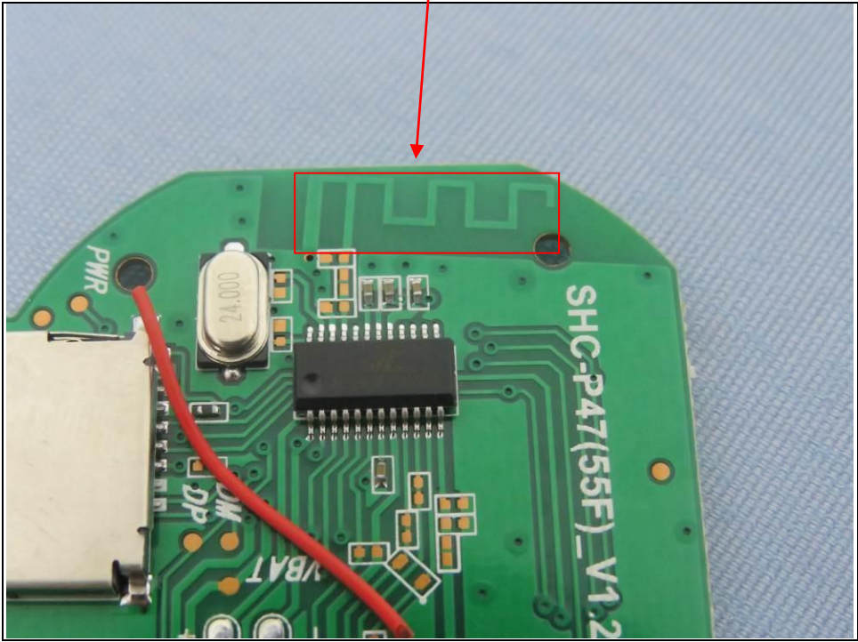
RF Antenna
