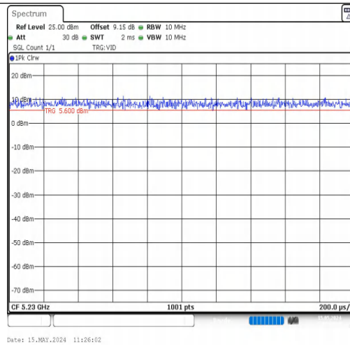
NTNV-11N40MIMO-Ant2-5230
