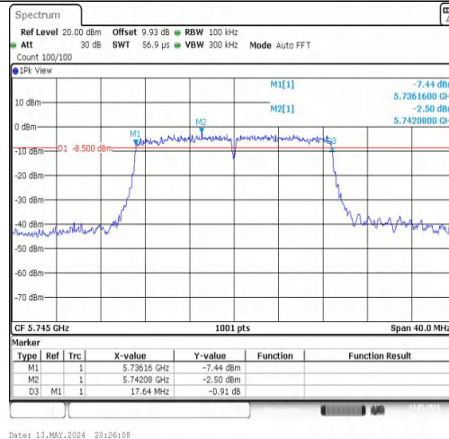
11N20MIMO-Ant2-5745-PASS
