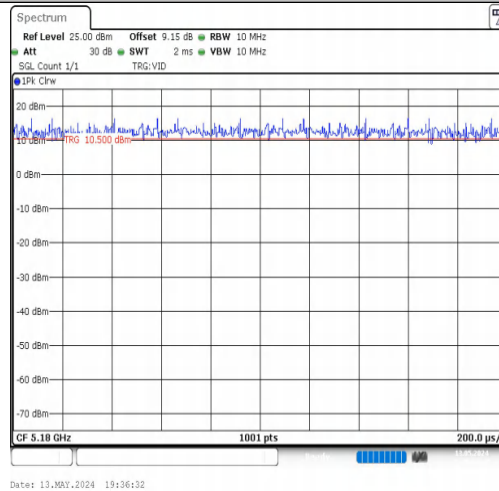
NTNV-11A-CDD-Ant2-5180
