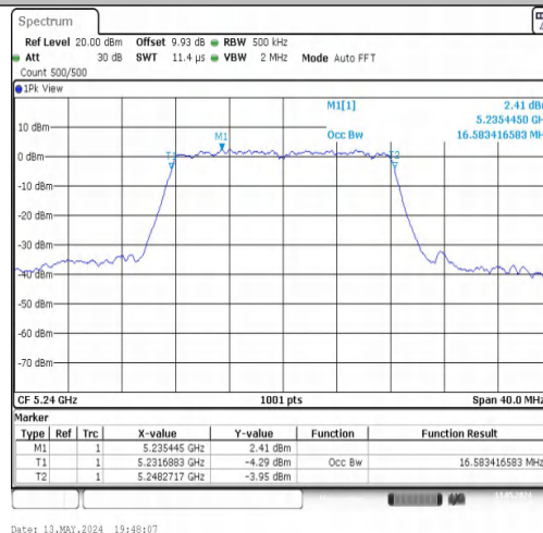
11A-CDD-Ant2-5240
