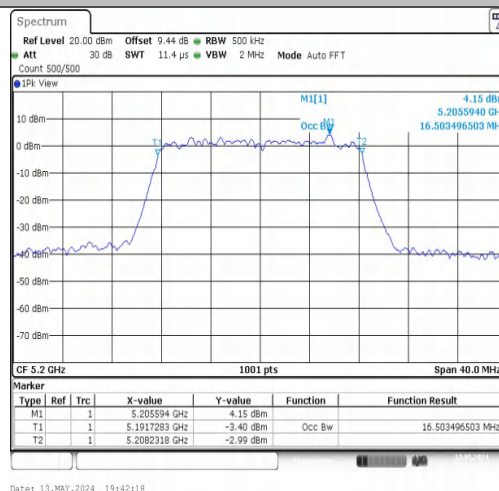
11A-CDD-Ant1-5200
