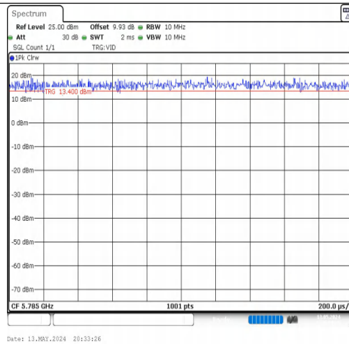
NTNV-11N20MIMO-Ant2-5785
