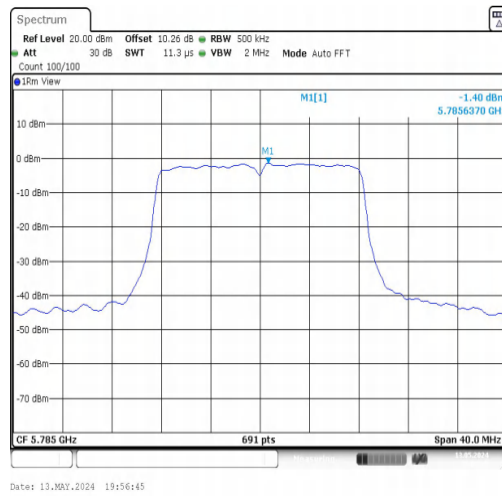
11A-CDD-Ant1-5785-PASS
