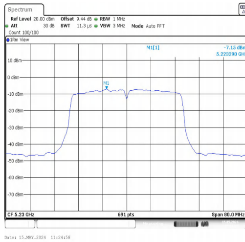
11N40MIMO-Ant1-5230-PASS
