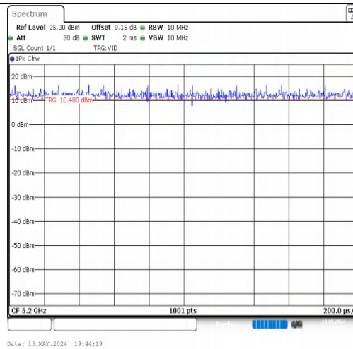
NTNV-11A-CDD-Ant2-5200
