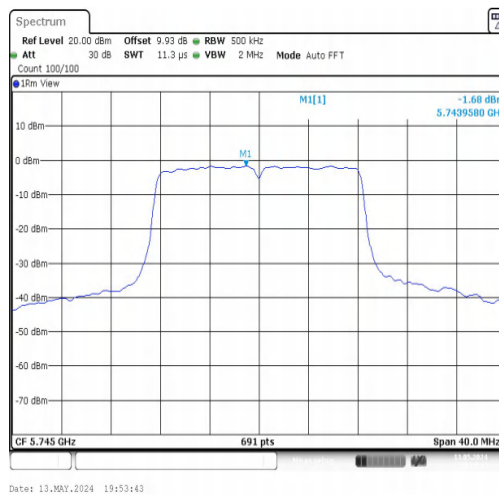
11A-CDD-Ant2-5745-PASS
