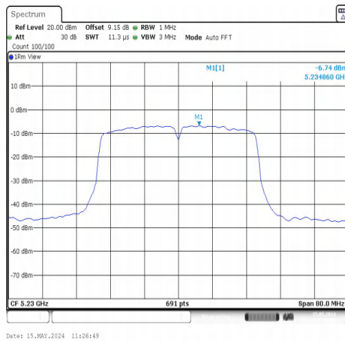
11N40MIMO-Ant2-5230-PASS
