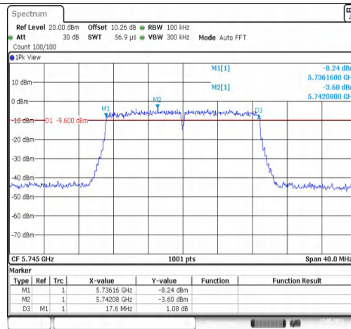
11N20MIMO-Ant1-5745-PASS
