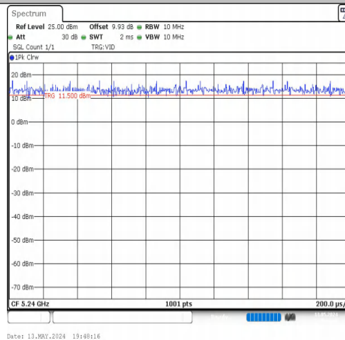
NTNV-11A-CDD-Ant2-5240
