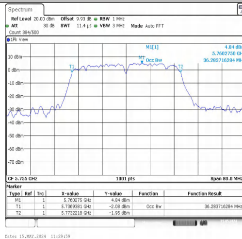
11N40MIMO-Ant2-5755
