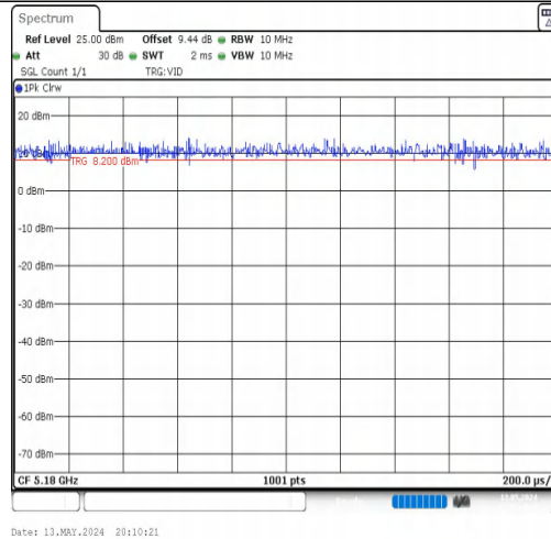
NTVN-11N20MIMO-Ant1-5180
