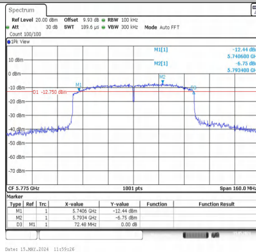
11AC80MIMO-Ant2-5775-PASS
