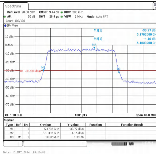
11N20MIMO-Ant1-5180
