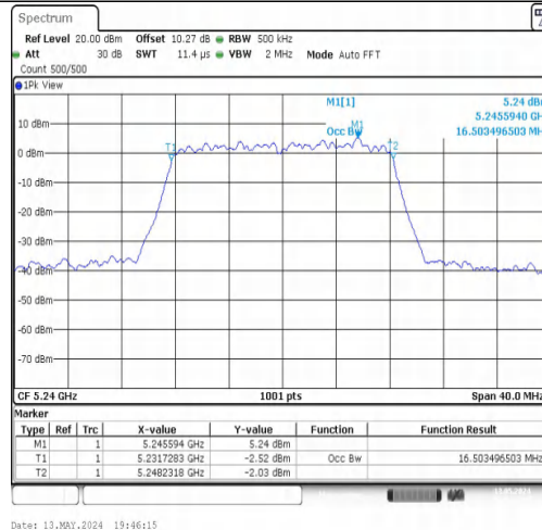
11A-CDD-Ant1-5240
