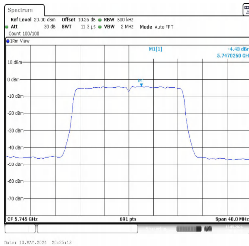
11N20MIMO-Ant1-5745-PASS
