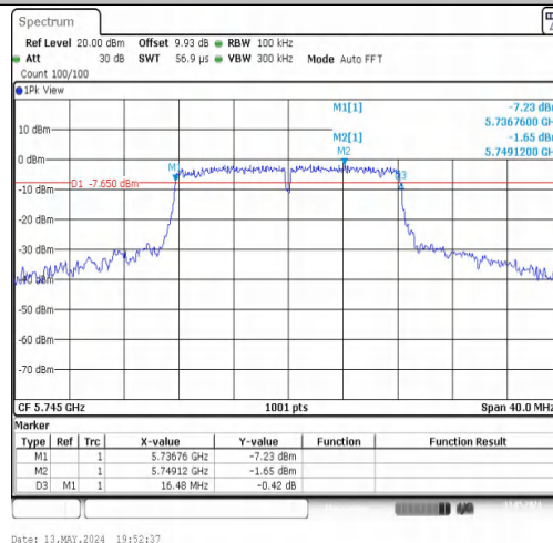
11A-CDD-Ant2-5745-PASS
