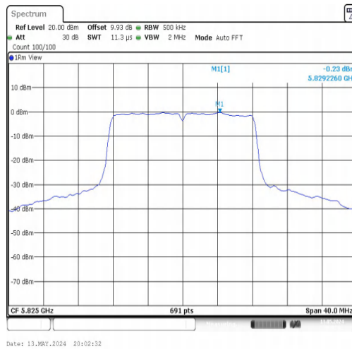
11A-CDD-Ant2-5825-PASS
