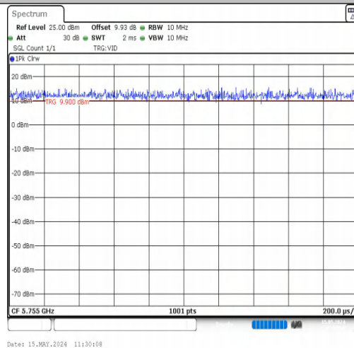
NTNV-11N40MIMO-Ant2-5755
