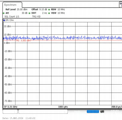
NTNV-11AC80MIMO-Ant2-5210
