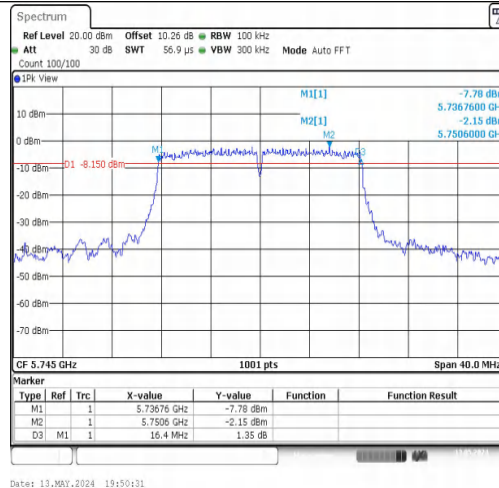
11A-CDD-Ant1-5745-PASS
