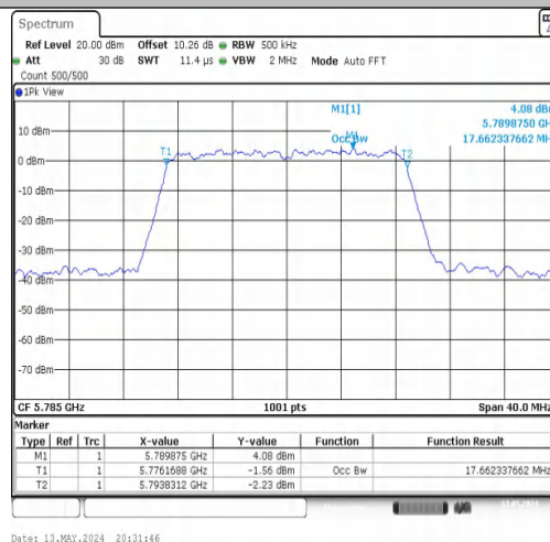
11N20MIMO-Ant1-5785
