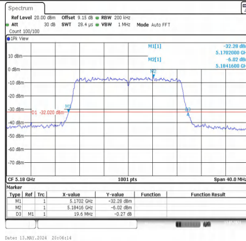
11N20MIMO-Ant2-5180
