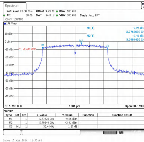
11N40MIMO-Ant2-5795-PASS
