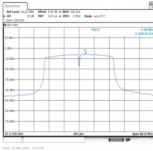
11N40MIMO-Ant2-5755-PASS
