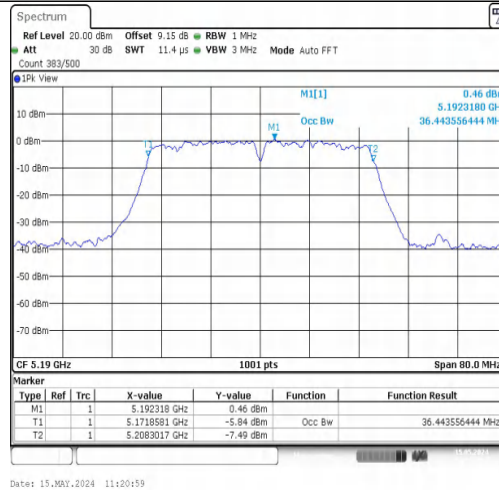
11N40MIMO-Ant2-5190
