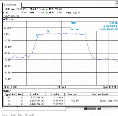
11A-CDD-Ant2-5180
