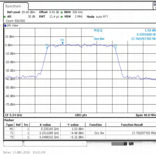
11N20MIMO-Ant2-5240
