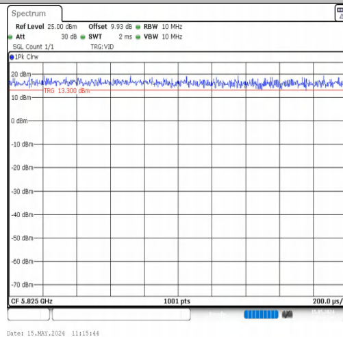
NTNV-11N20MIMO-Ant2-5825
