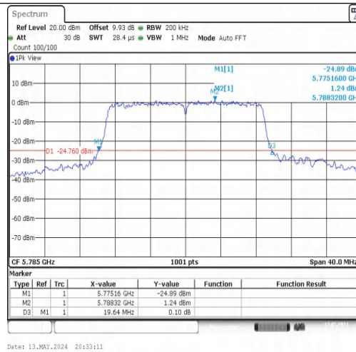
11N20MIMO-Ant2-5785
