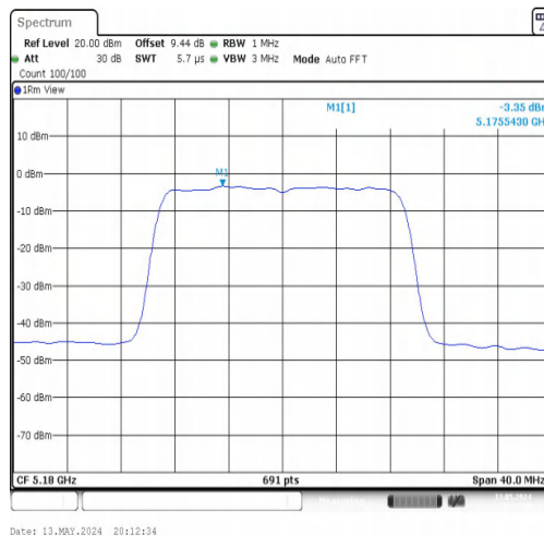
11N20MIMO-Ant1-5180-PASS
