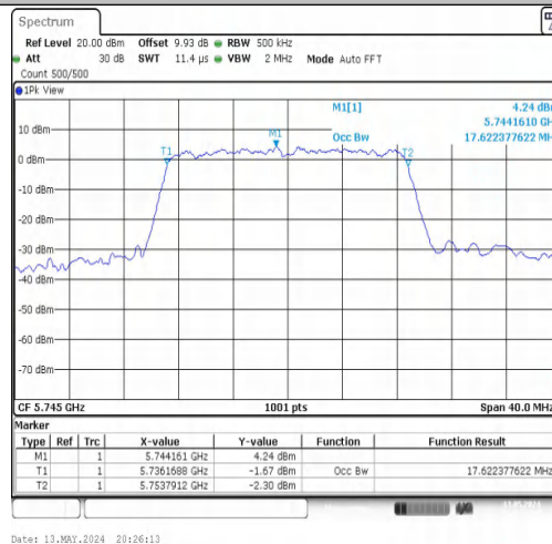
11N20MIMO-Ant2-5745
