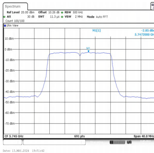
11A-CDD-Ant1-5745-PASS
