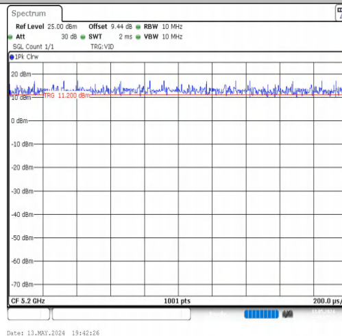
NTNV-11A-CDD-Ant1-5200
