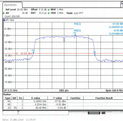
11AC80MIMO-Ant2-5210
