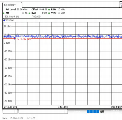
NTVN-11N40MIMO-Ant1-5190
