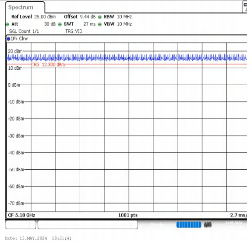
NTNV-11A-CDD-Ant1-5180
