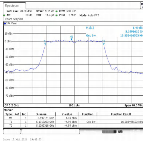
11A-CDD-Ant2-5200
