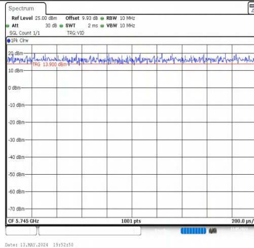
NTNV-11A-CDD-Ant2-5745
