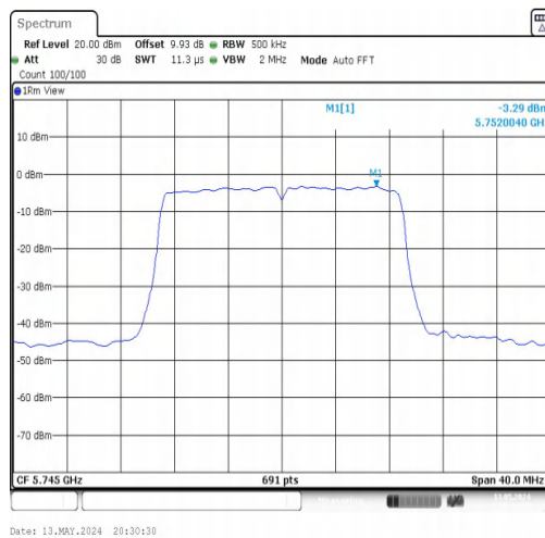
11N20MIMO-Ant2-5745-PASS
