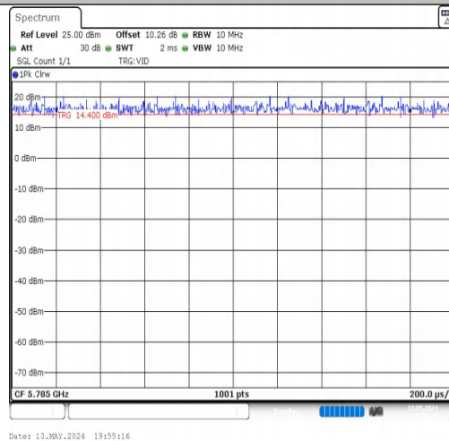
NTNV-11A-CDD-Ant1-5785
