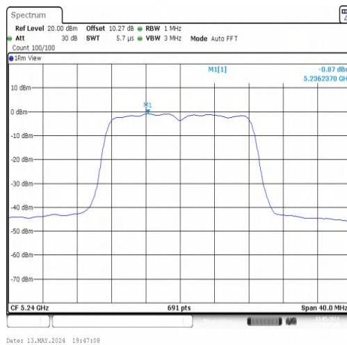
11A-CDD-Ant1-5240-PASS
