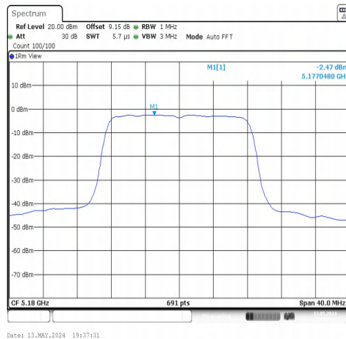
11A-CDD-Ant2-5180-PASS
