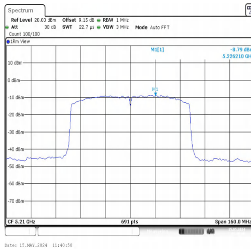
11AC80MIMO-Ant2-5210-PASS
