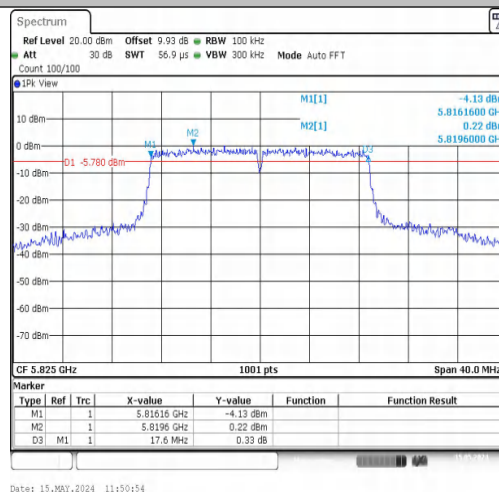
11N20MIMO-Ant2-5825-PASS
