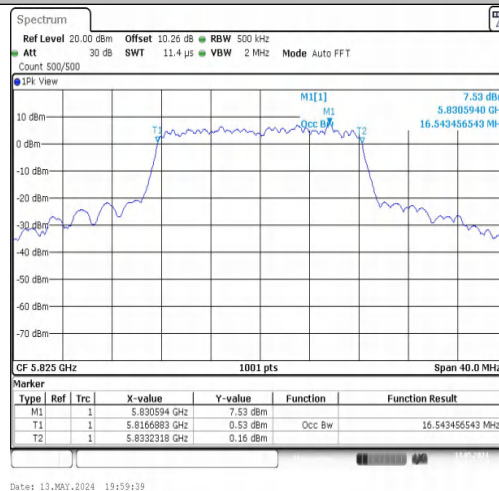
11A-CDD-Ant1-5825
