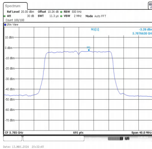
11N20MIMO-Ant1-5785-PASS
