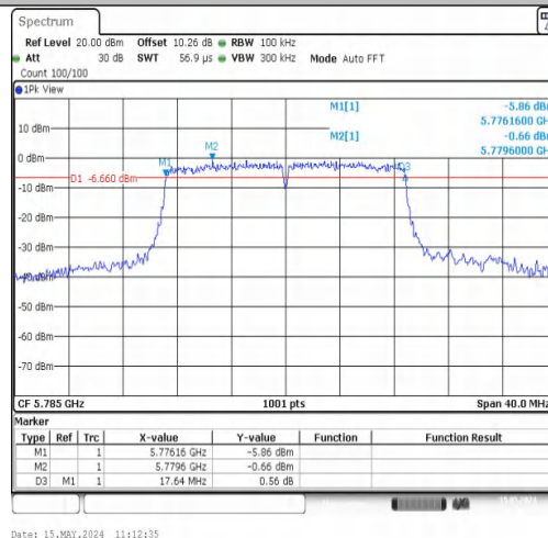
11N20MIMO-Ant1-5785-PASS
