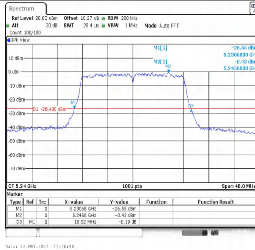
11A-CDD-Ant1-5240
