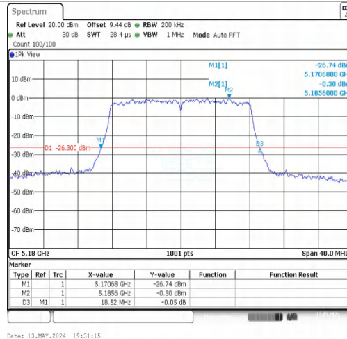
11A-CDD-Ant1-5180
