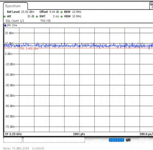
NTVN-11N40MIMO-Ant1-5230
