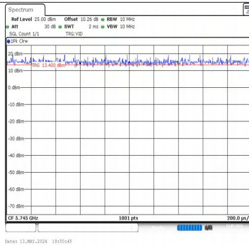
NTNV-11A-CDD-Ant1-5745
