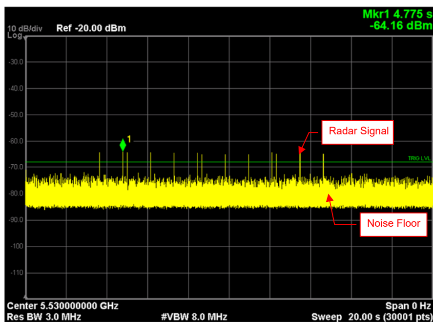
Radar Signal 5
