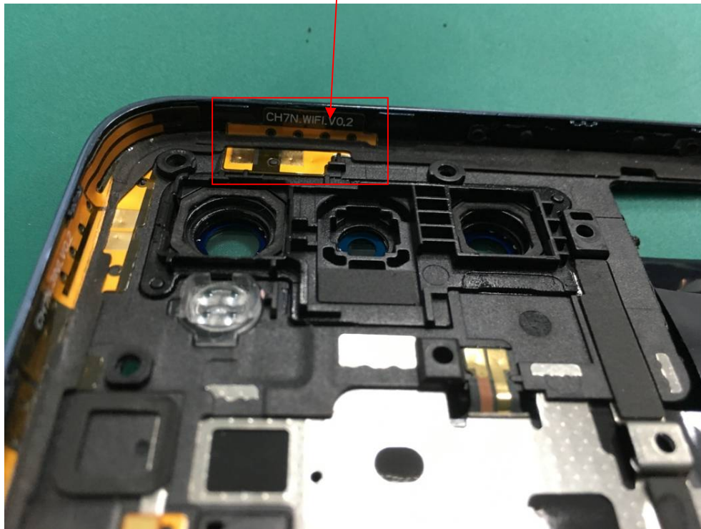
5G WIFI Antenna
