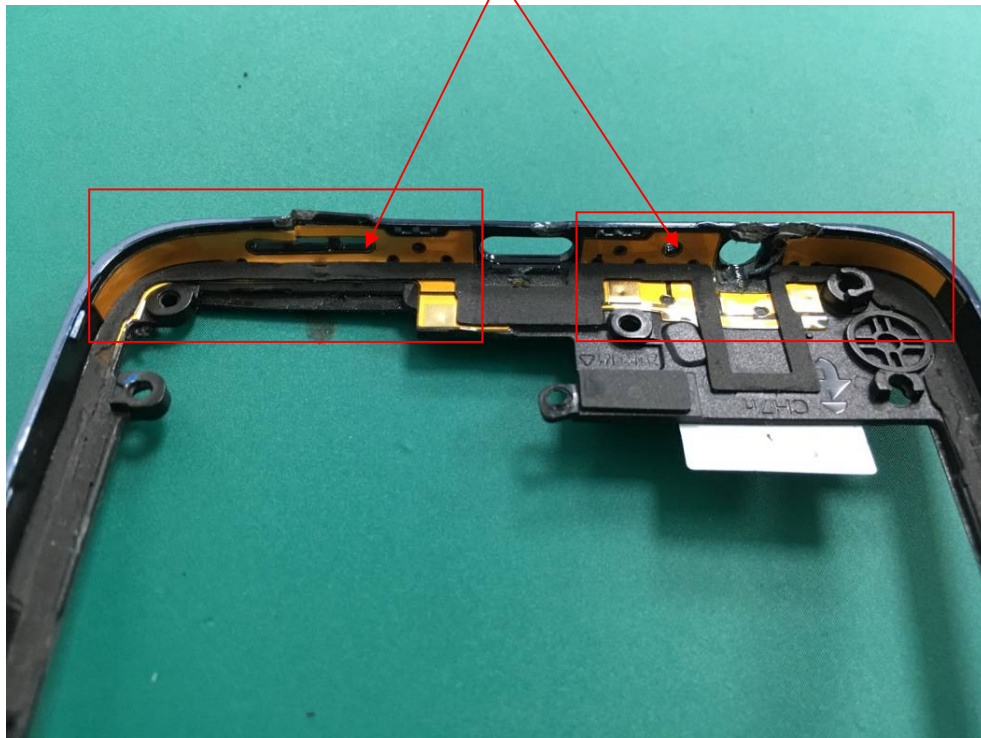
Aux Antenna
