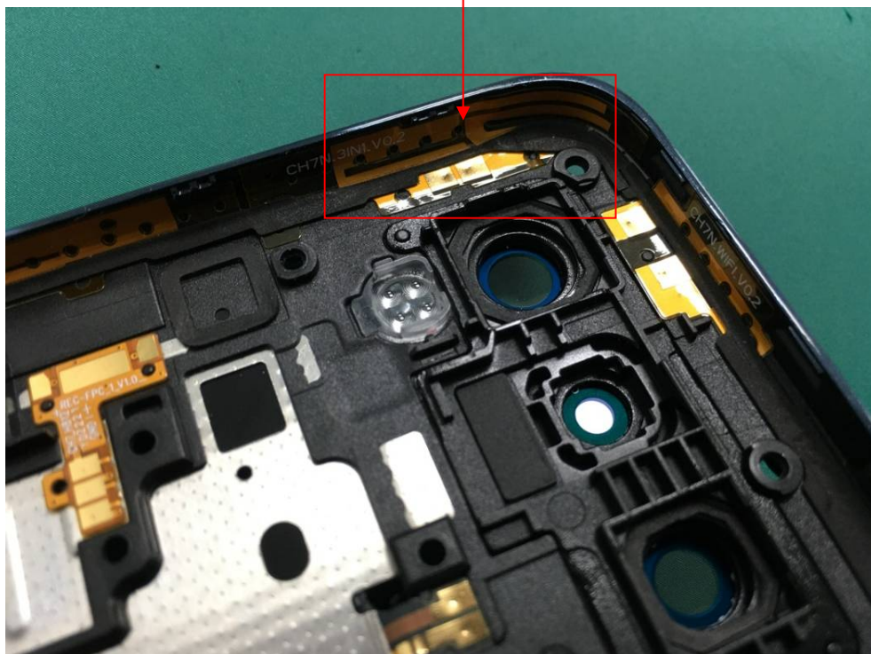
BT/BLE/2.4G WIFI Antenna
