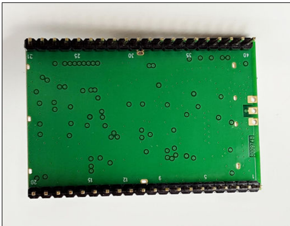
Figure 4: External Photo – DNT2400PP Bottom
