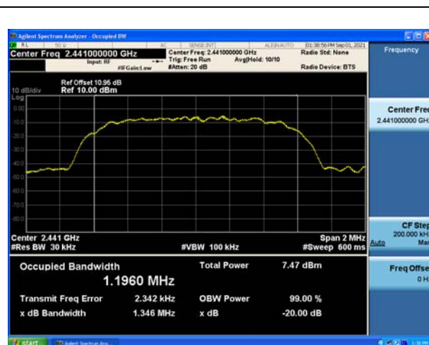
Modulation: 8DPSK 2441MHz
