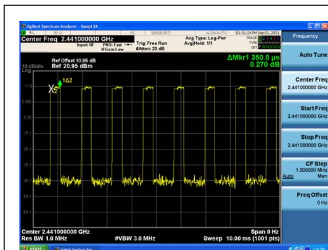
Modulation: 8DPSK 3DH1 2441MHz
