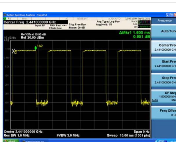
Modulation: \pi/4 DQPSK 2DH3 2441MHz
