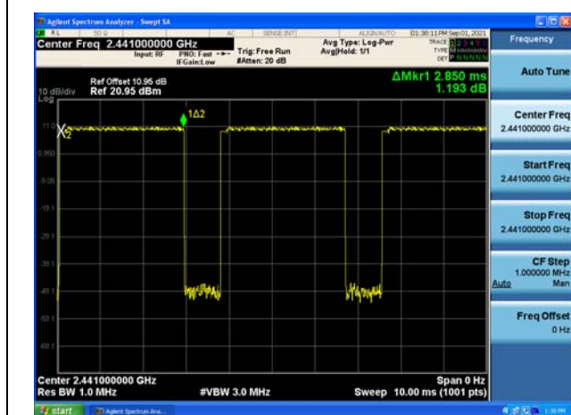
Modulation: 8DPSK 3DH5 2441MHz
