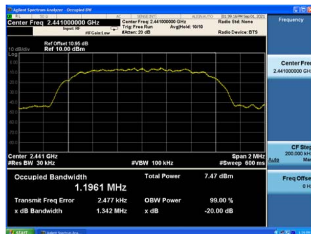
Modulation: 8DPSK 2441MHz
