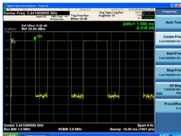
Modulation: GFSK DH3 2441MHz
