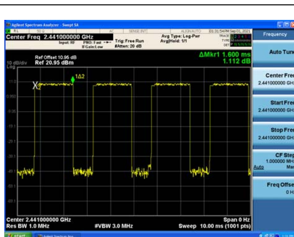
Modulation: 8DPSK 3DH3 2441MHz
