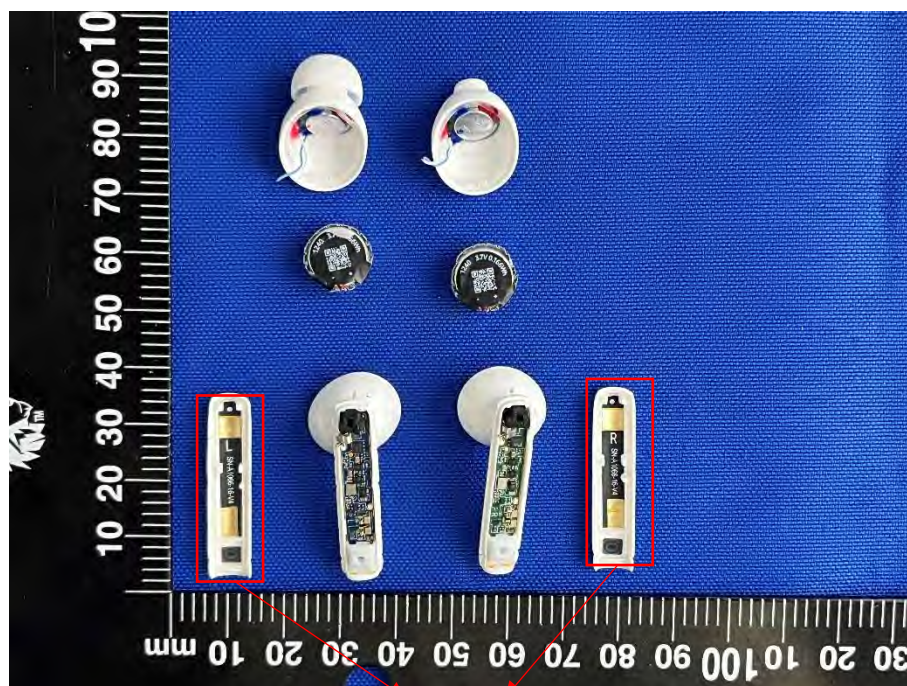
FPC Antenna
